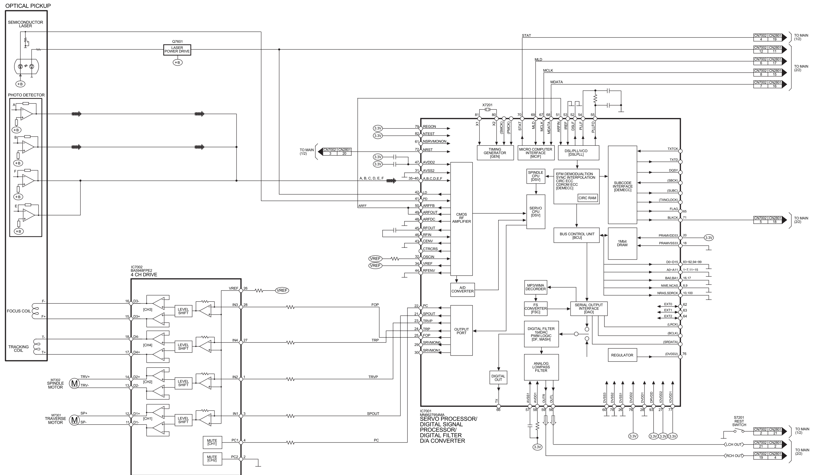
SA-AK750GCP CD SERVO BLOCK DIAGRAM
