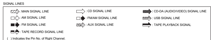
SA-AK750GCP DECK/DECK MECHANISM BLOCK DIAGRAM
