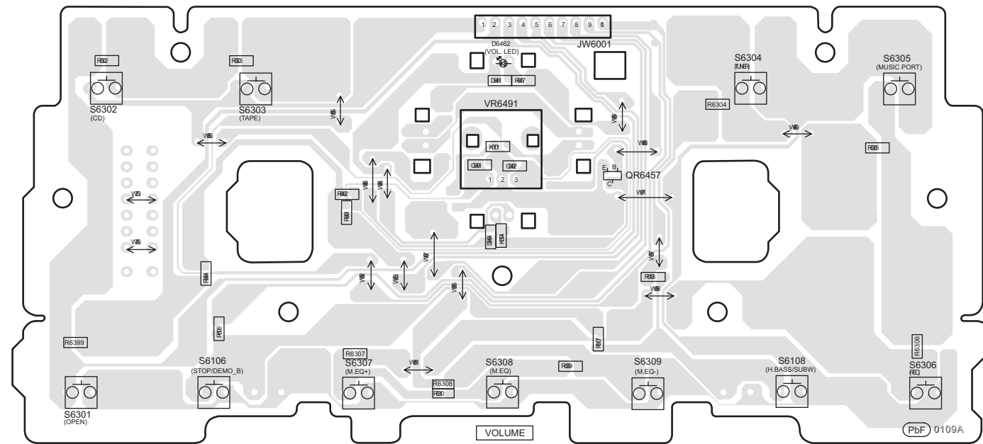
D SUB PANEL P.C.B (REPV0131B)
