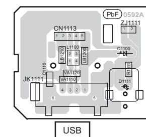
K USB CONNECTOR/LED P.C.B. (REPX0673E)
