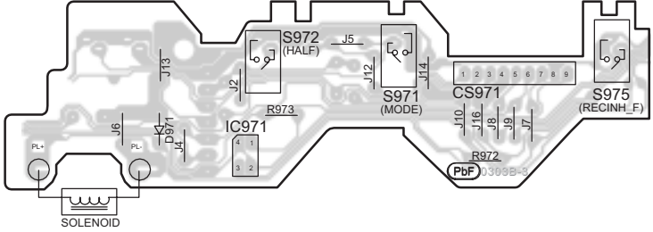
J DECK MECHANISM P.C.B. (REPX0321L)
