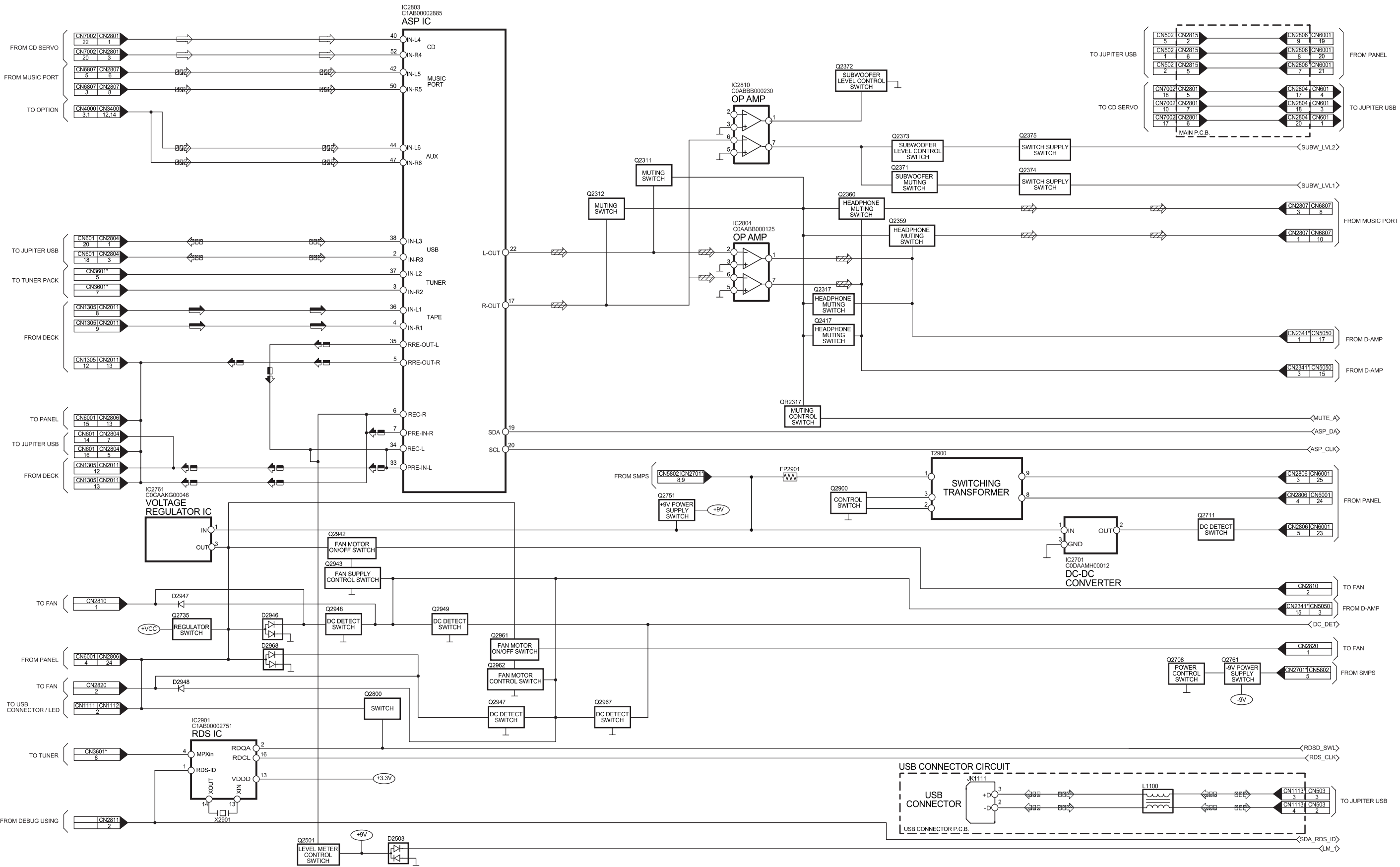
SA-AK770EB/EG MAIN(1/2) / USB CONNECTOR BLOCK DIAGRAM
