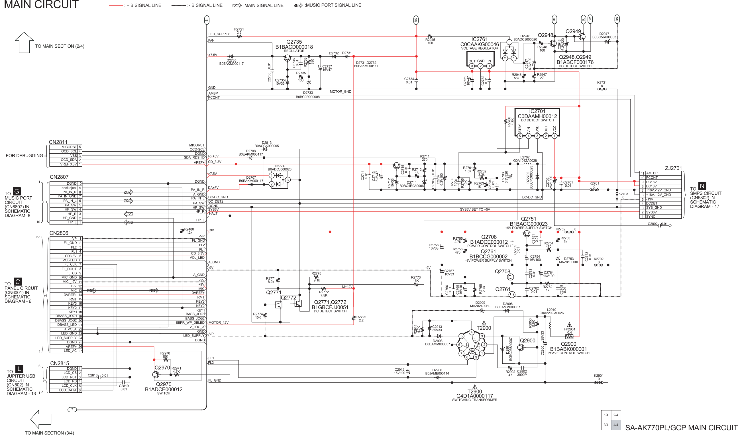
SCHEMATIC DIAGRAM - 5
