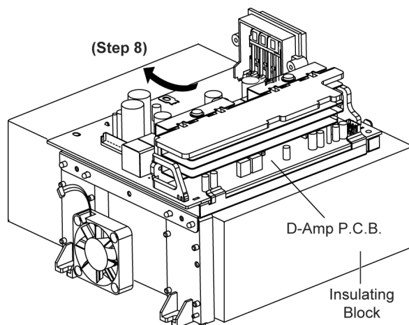
Step 8 Lift up D-Amp P.C.B. as arrow shown.
