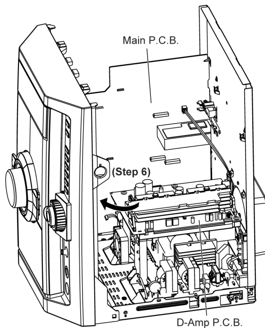
Step 7 Remove 3 screws from D-Amp P.C.B..
