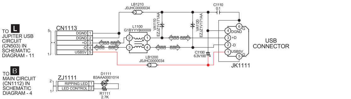
K USB CONNECTOR/LED CIRCUIT
