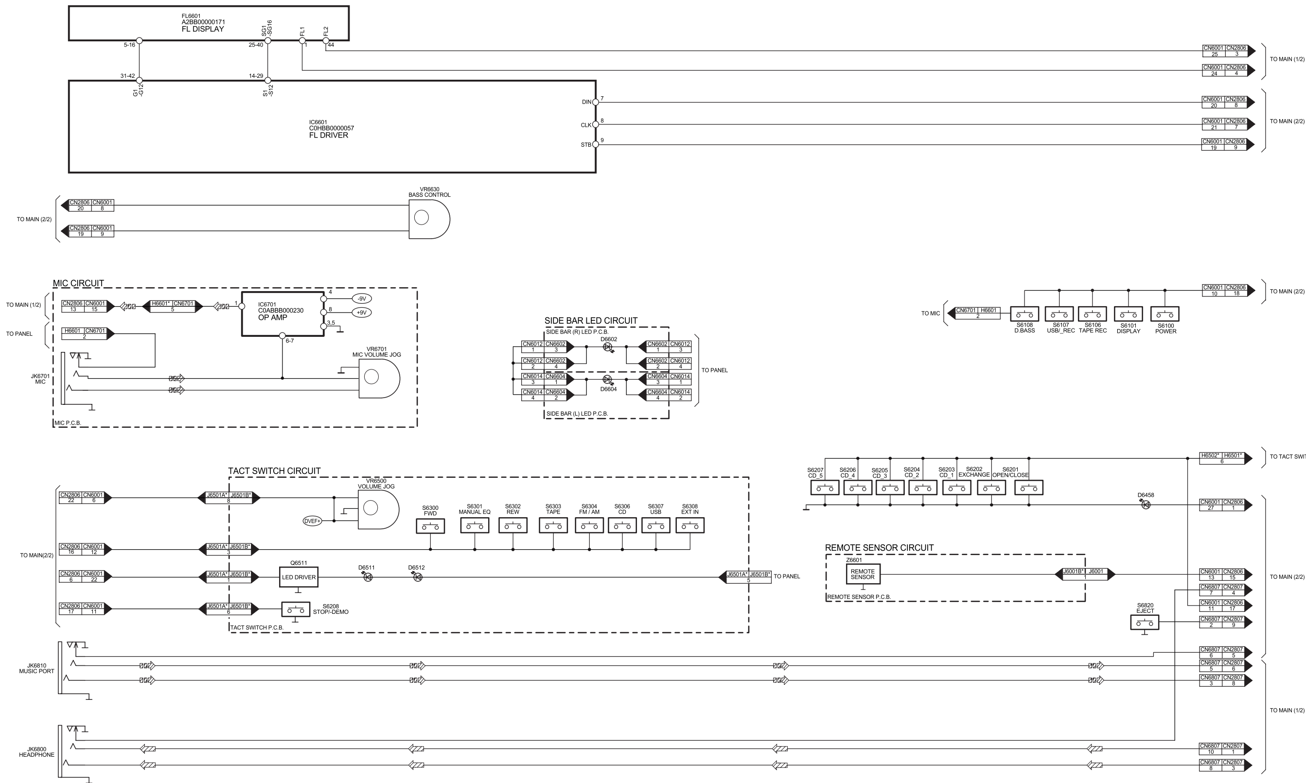
SA-AK770PL/GCP SIDE BAR LED / PANEL / REMOTE SENSOR / MUSIC PORT / HEADPHONE / TACT SWITCH / MICROPHONE BLOCK DIAGRAM
