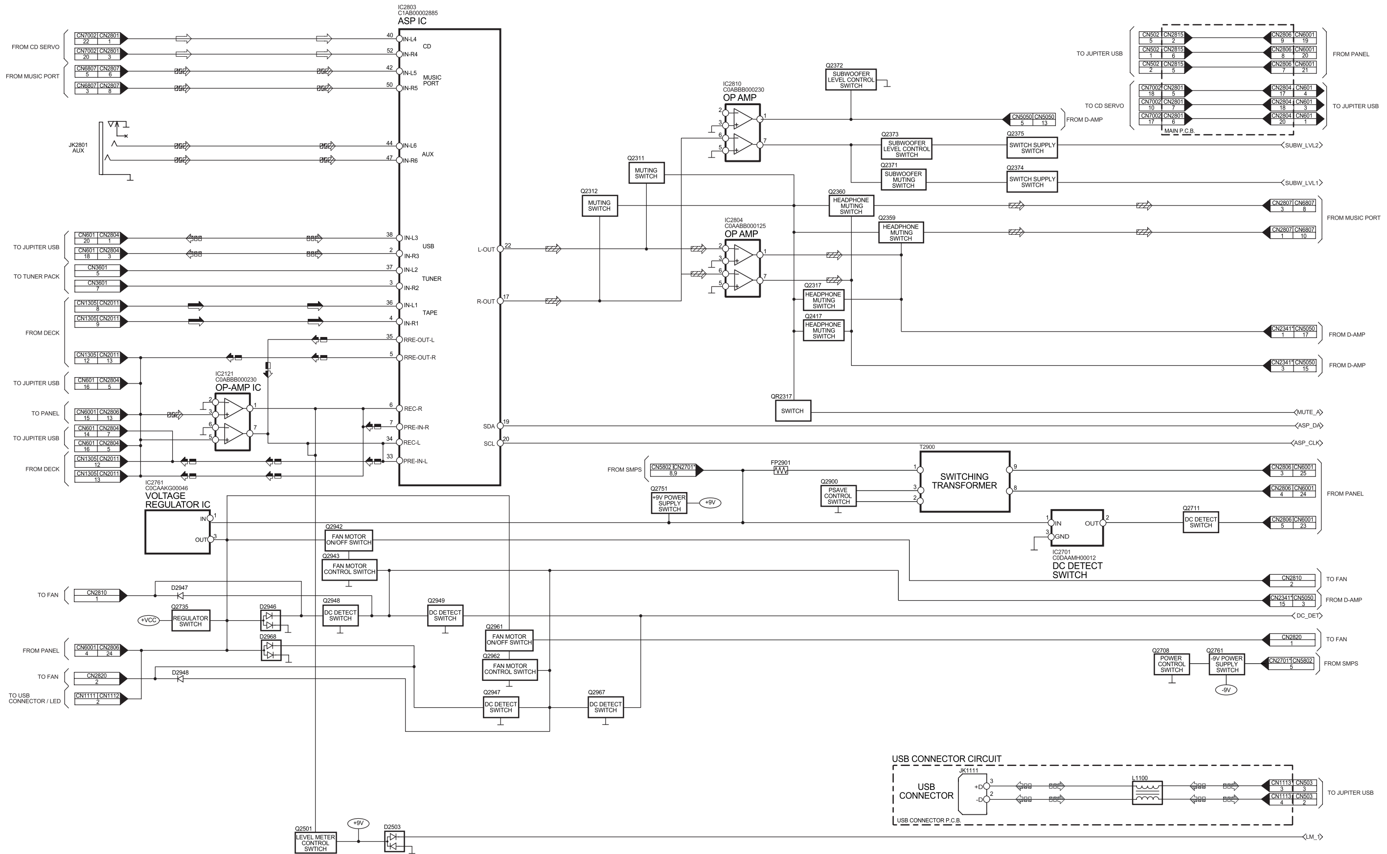
SA-AK770PL/GCP MAIN(1/2) / USB CONNECTOR BLOCK DIAGRAM
