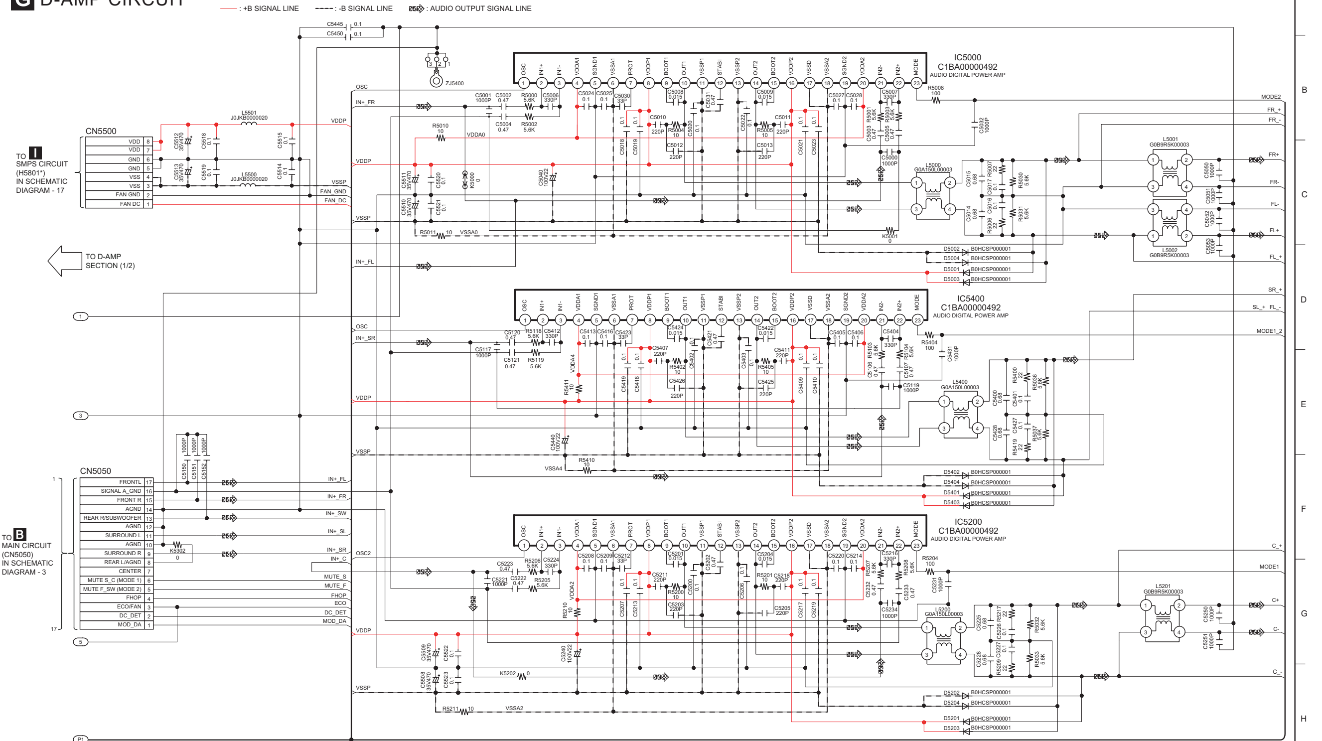
SCHEMATIC DIAGRAM - 12
