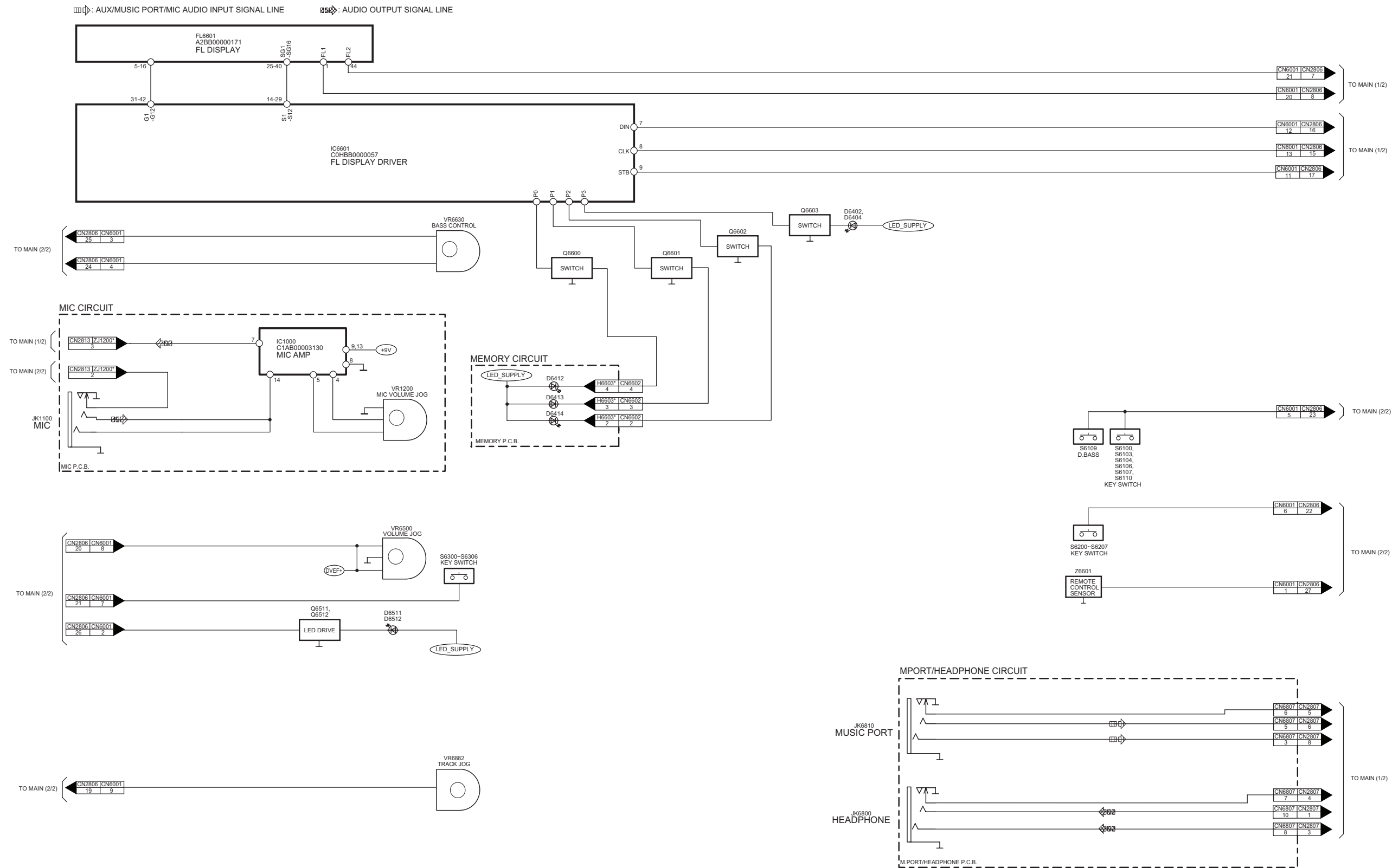
SA-AK780PH/PN PANEL / MPORT/HEADPHONE / MIC / MEMORY BLOCK DIAGRAM
