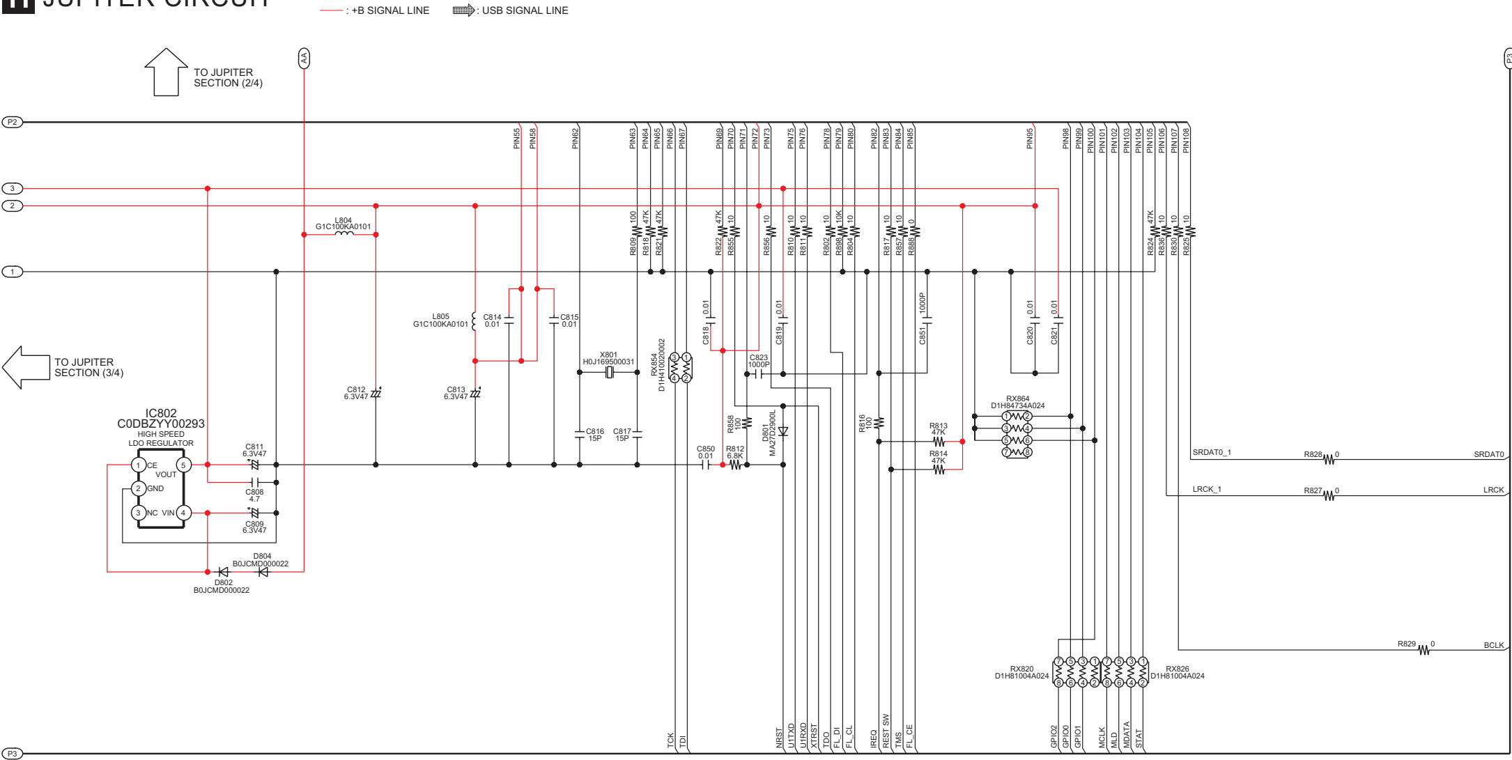
SCHEMATIC DIAGRAM - 16
