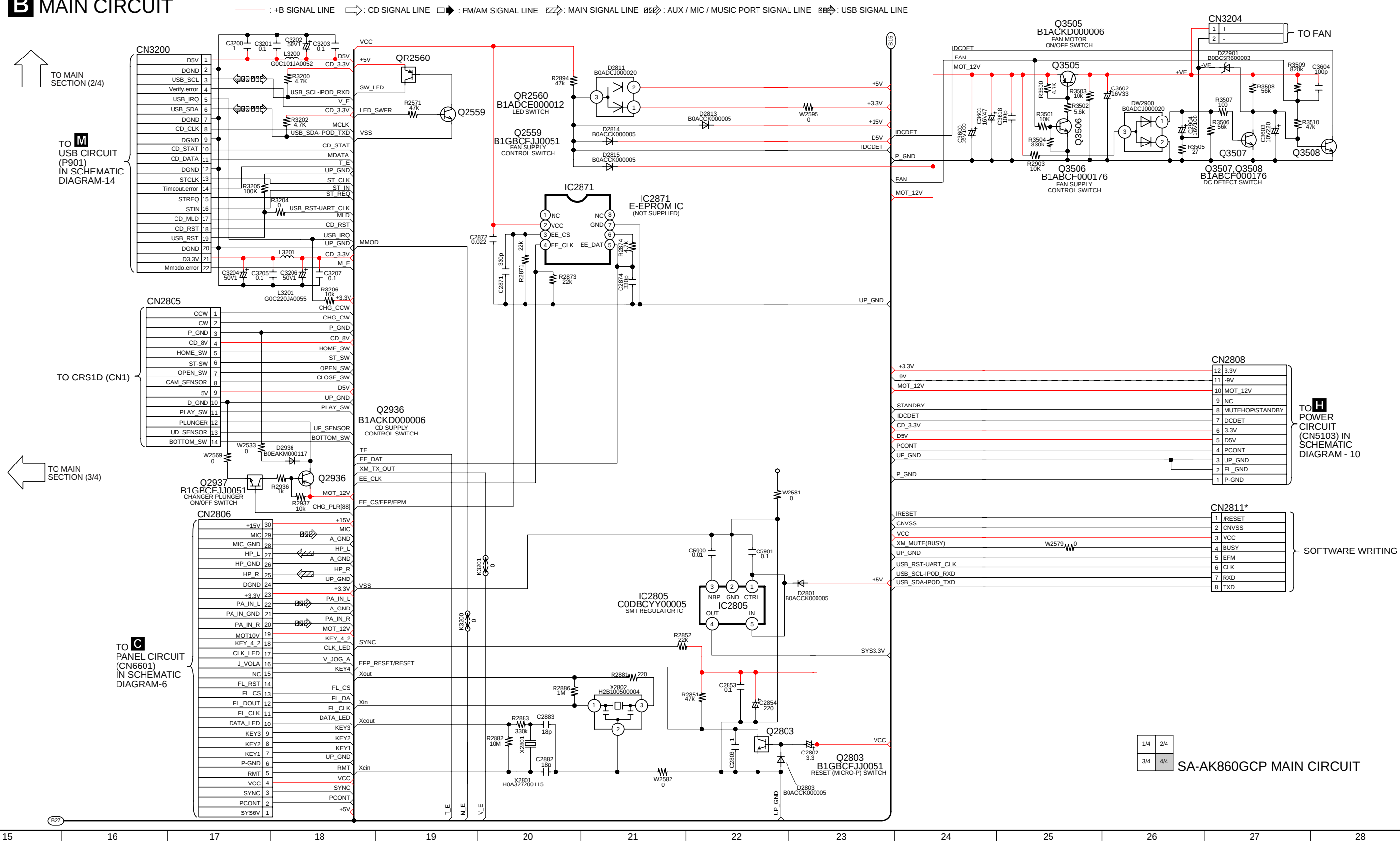
SCHEMATIC DIAGRAM - 5
