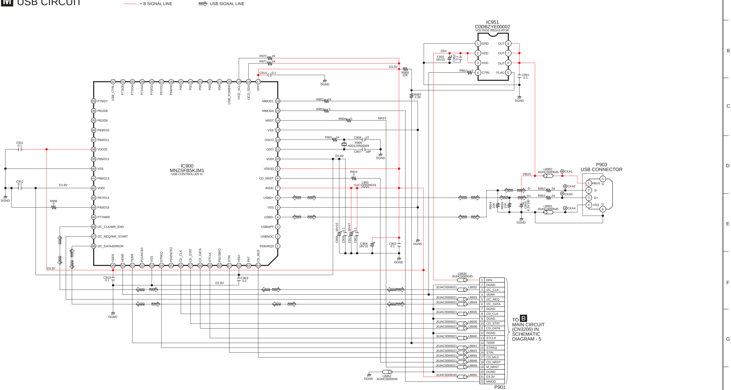
SA-AK860GCP USB CIRCUIT
