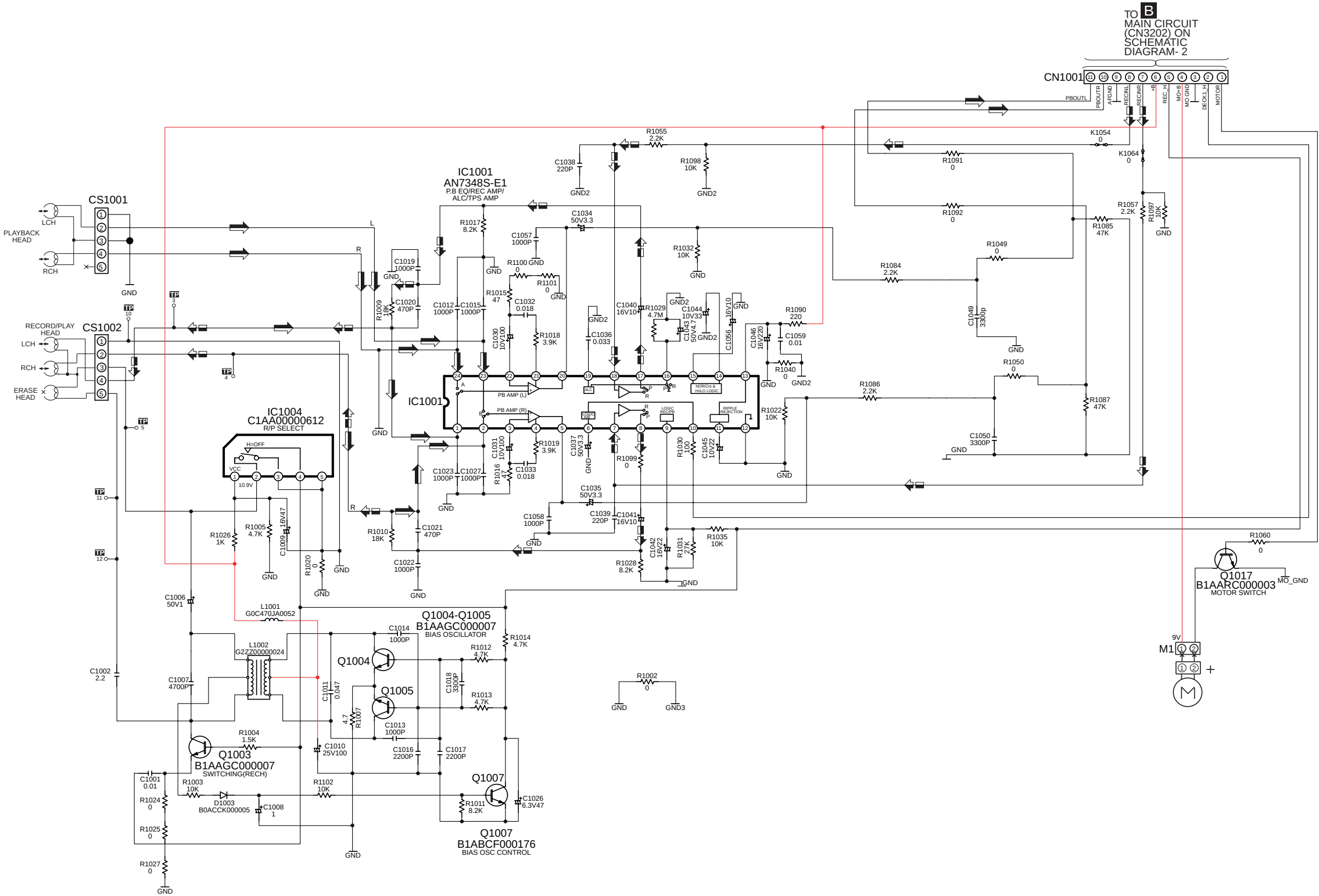
SCHEMATIC DIAGRAM - 12
