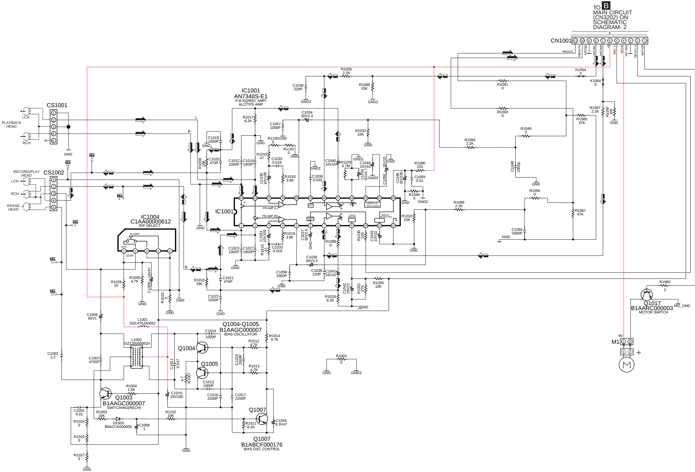
SCHEMATIC DIAGRAM - 12
