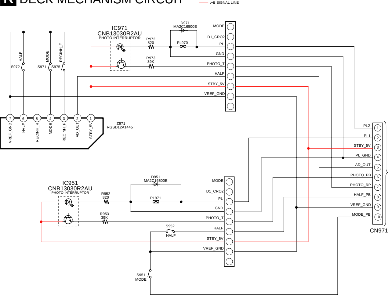
SCHEMATIC DIAGRAM - 8
