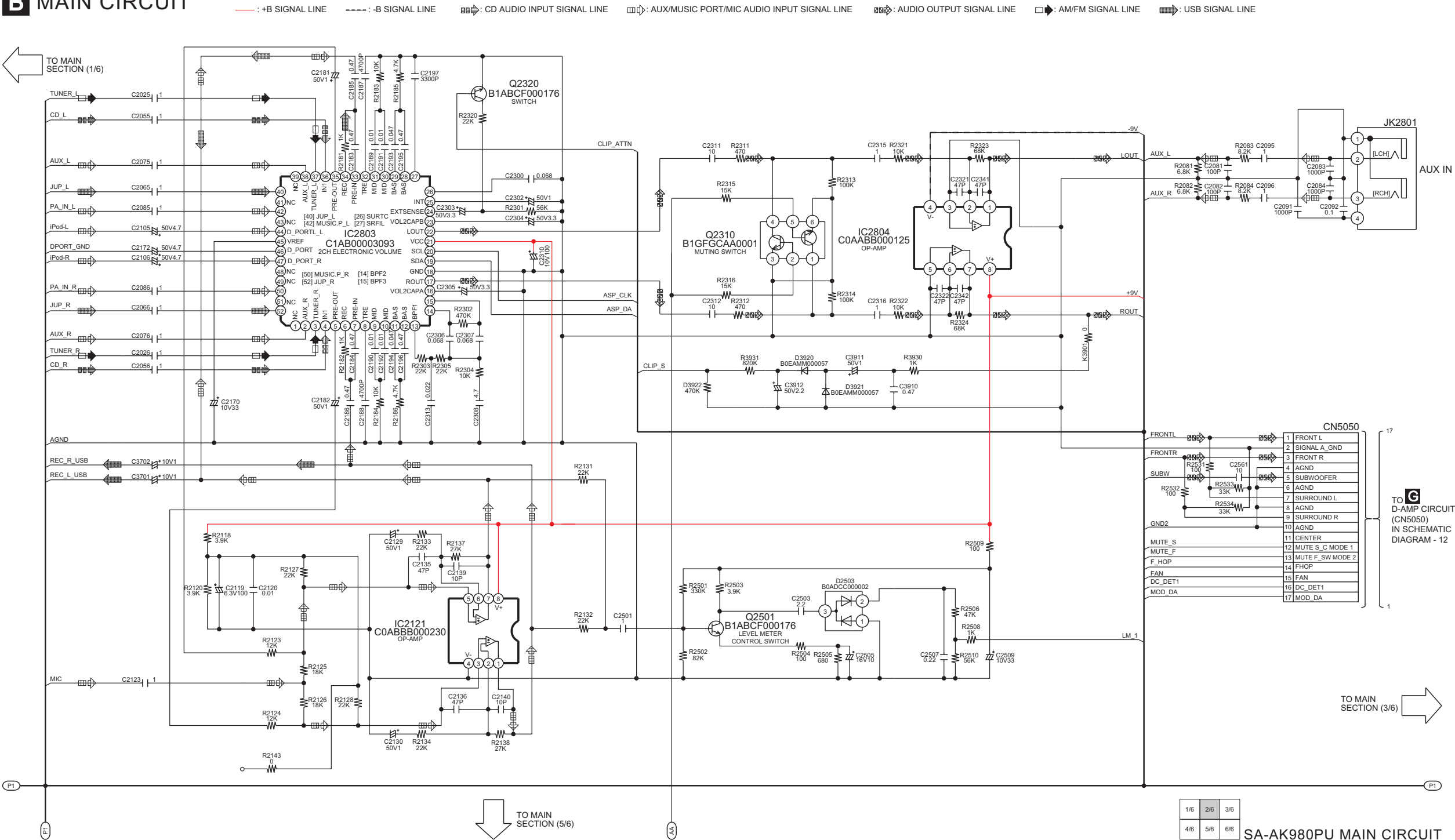
SCHEMATIC DIAGRAM - 3
