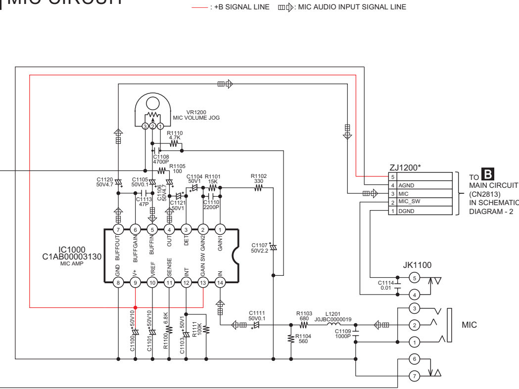
F MIC CIRCUIT
