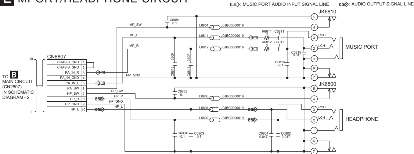
E MPORT/HEADPHONE CIRCUIT
