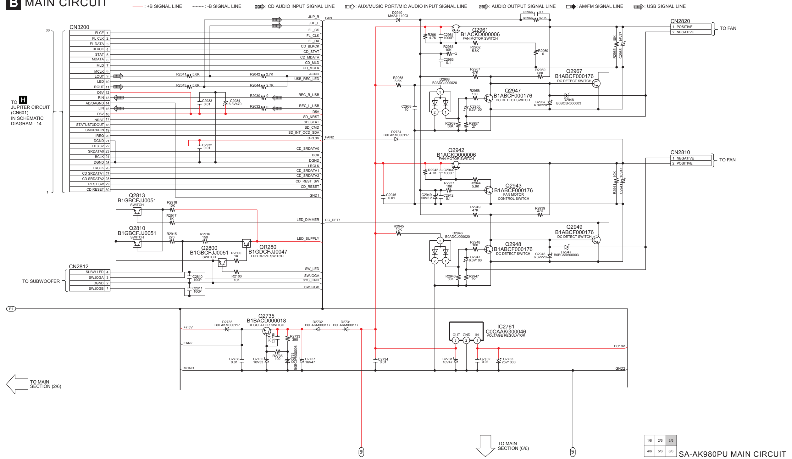
SCHEMATIC DIAGRAM - 4
