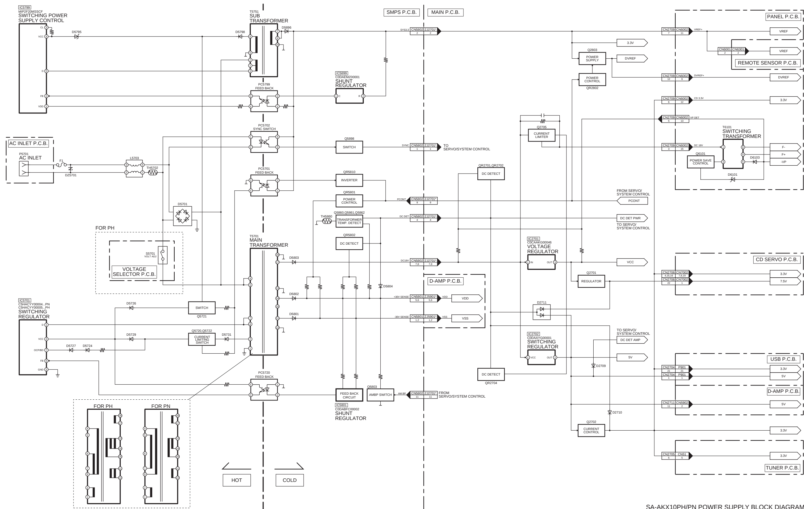
SA-AKX10PH/PN POWER SUPPLY BLOCK DIAGRAM
