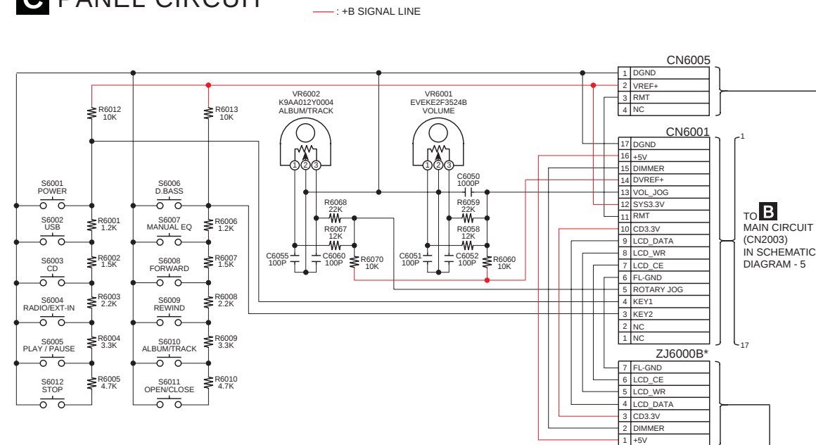
SCHEMATIC DIAGRAM - 7
