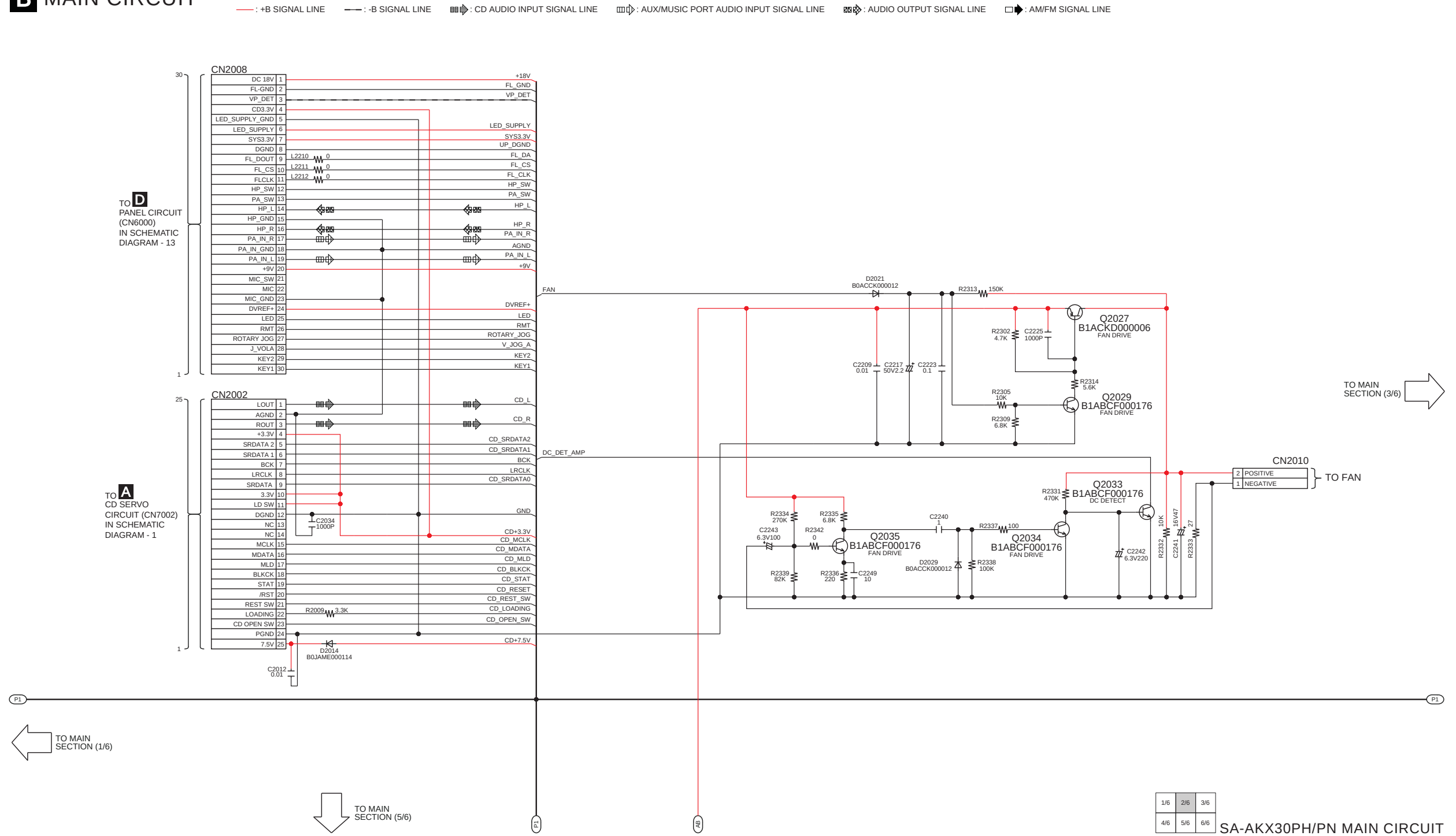
SCHEMATIC DIAGRAM - 3
