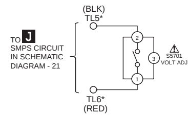
SCHEMATIC DIAGRAM - 22 K VOLTAGE SELECTOR CIRCUIT (FOR PH)
