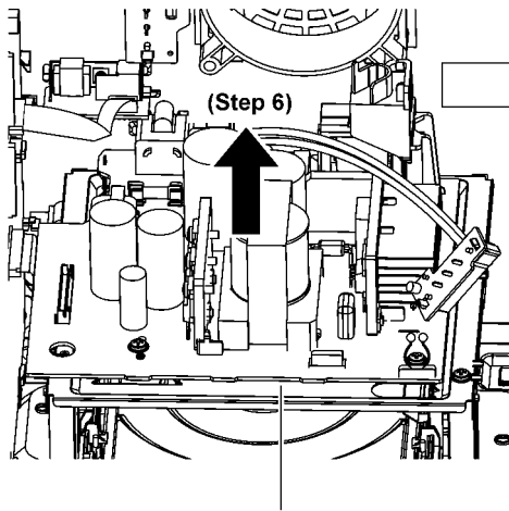
SMPS Inner Chassis Unit
