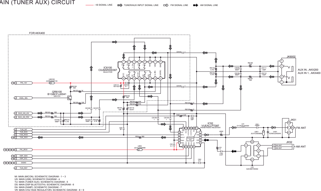
SCHEMATIC DIAGRAM - 5
