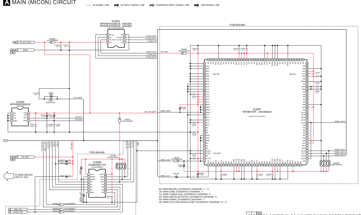
SCHEMATIC DIAGRAM - 3
