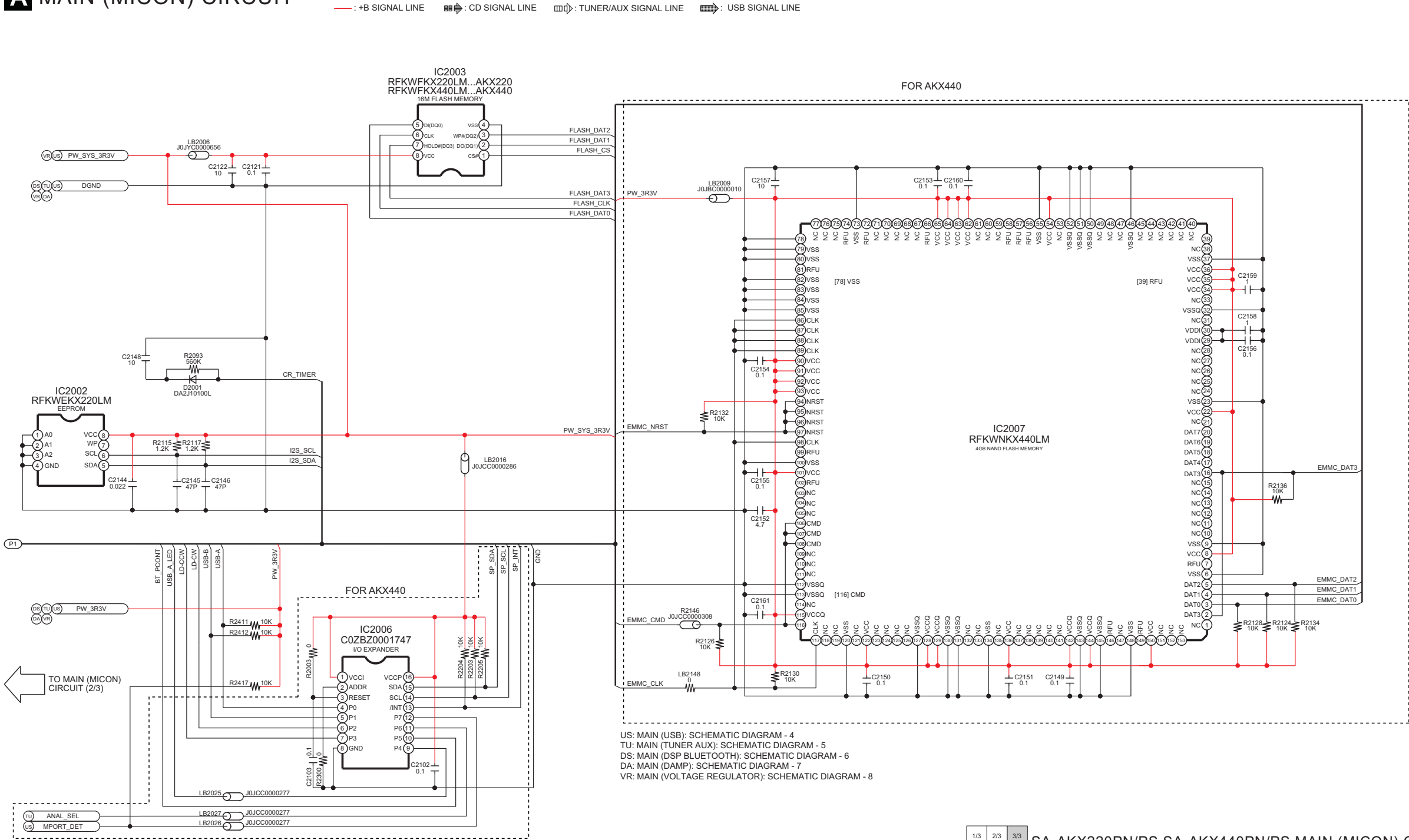
SCHEMATIC DIAGRAM - 3
