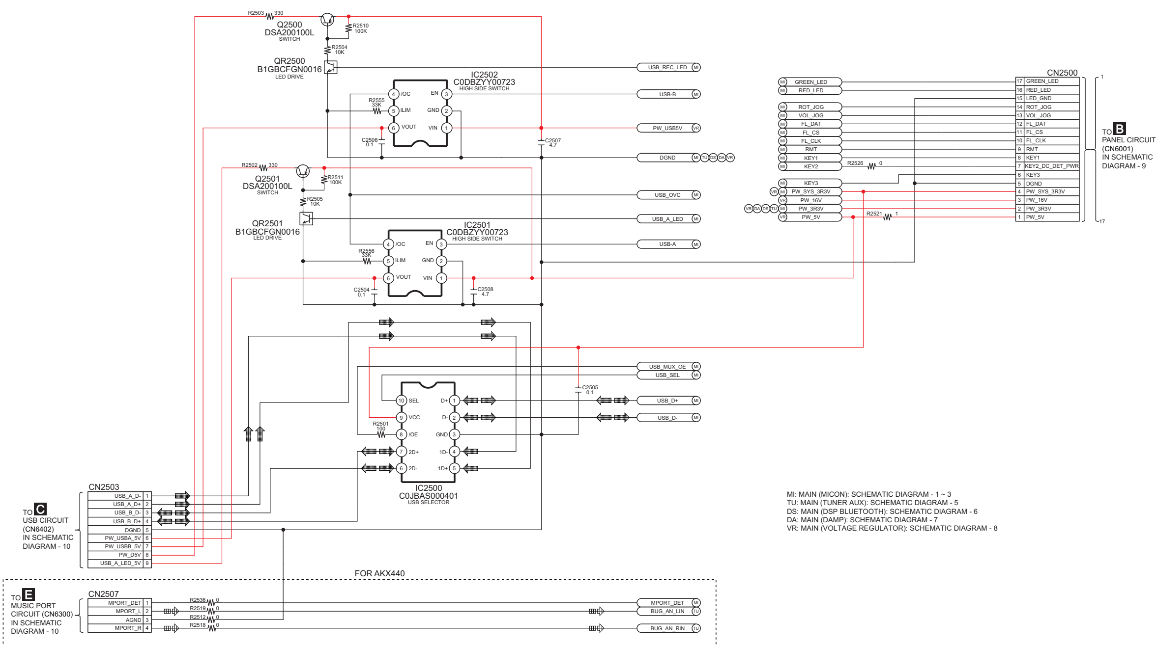
SA-AKX220PN/PS,SA-AKX440PN/PS MAIN (USB) CIRCUIT
