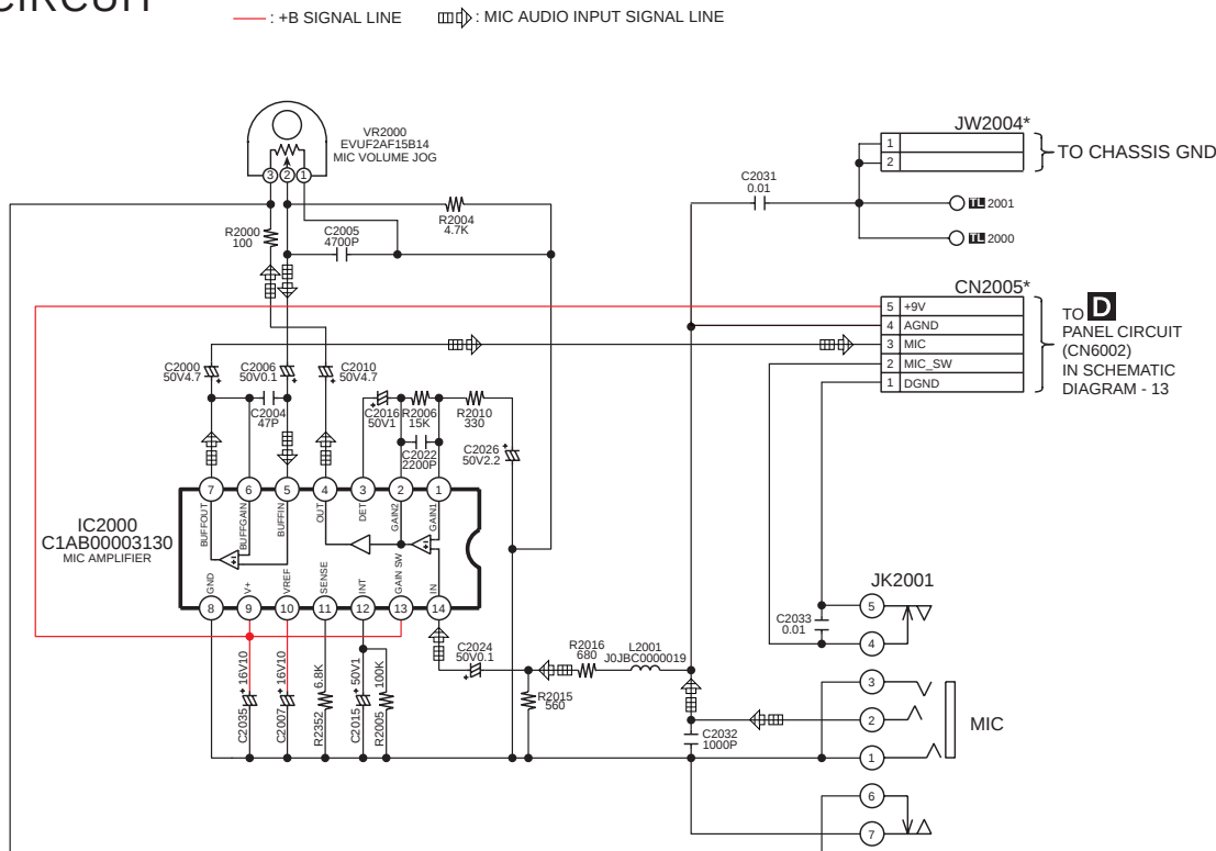
SCHEMATIC DIAGRAM - 19
