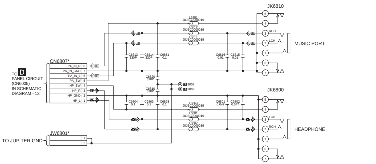
SA-AKX50PH/PN CD OPEN BUTTON / REMOTE SENSOR / TUNER / MUSIC PORT/HEADPHONE CIRCUIT
