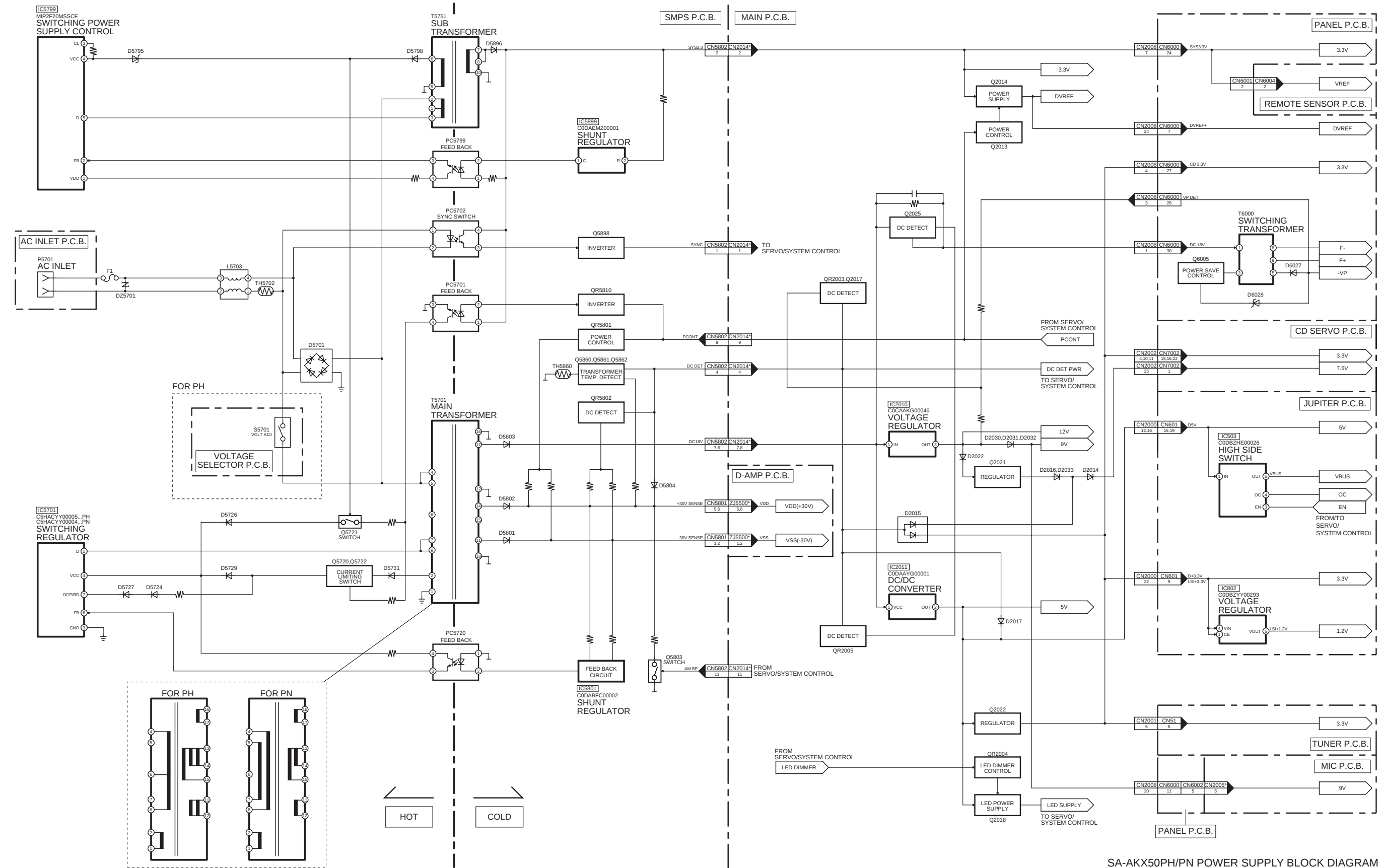
SA-AKX50PH/PN POWER SUPPLY BLOCK DIAGRAM
