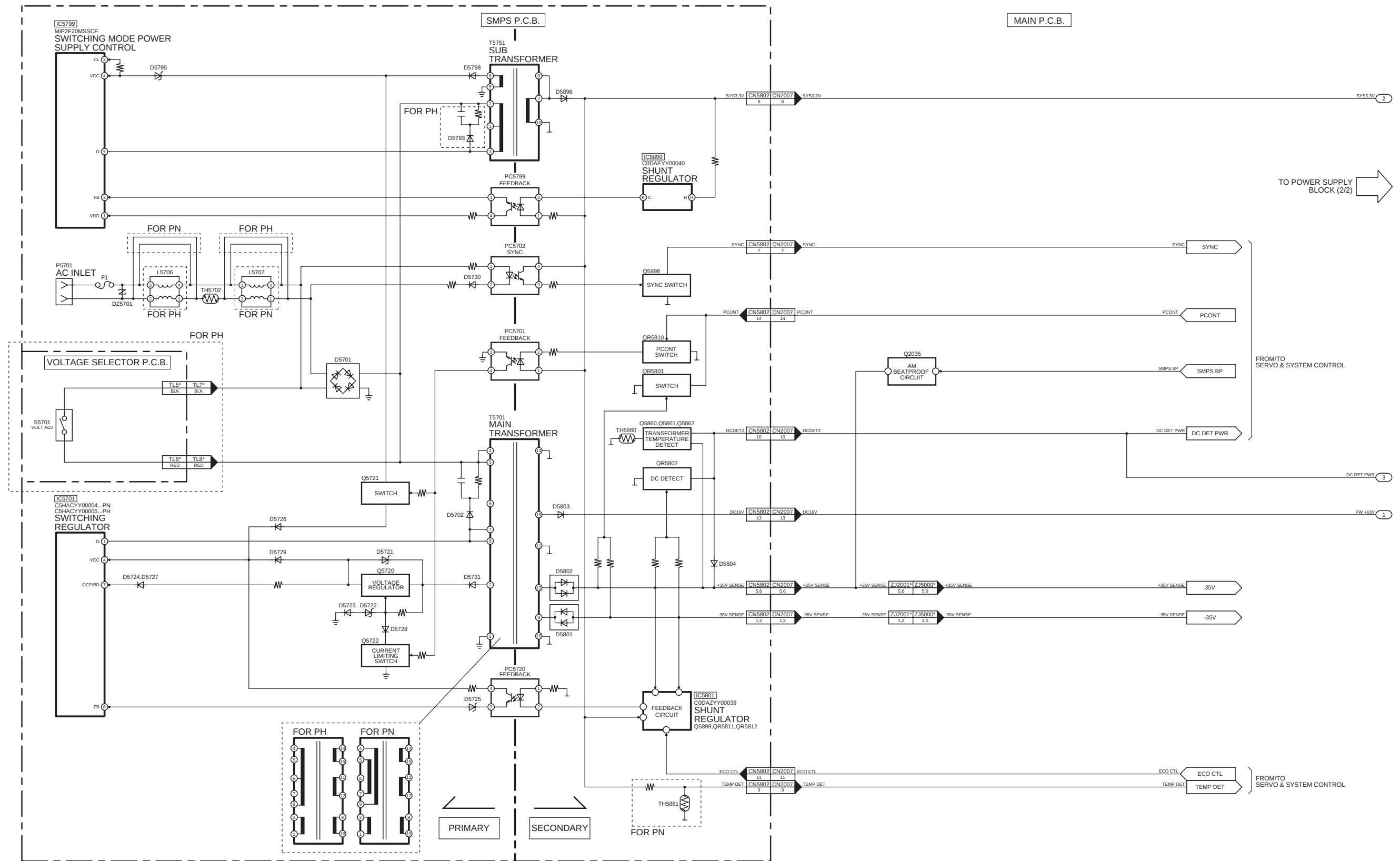
SA-AKX54PH/PN POWER SUPPLY (1/2) BLOCK DIAGRAM
