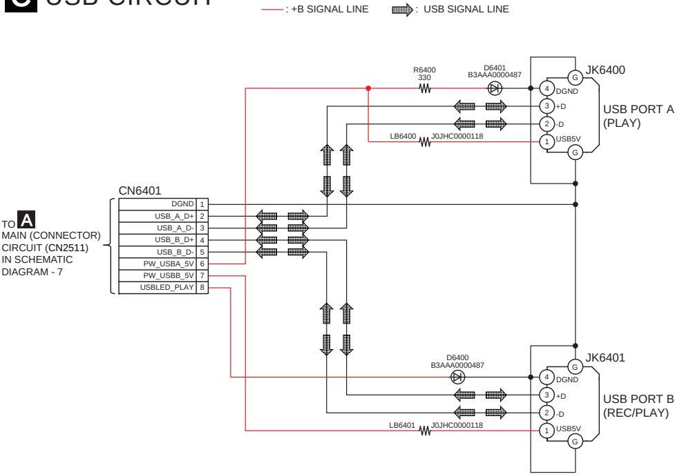
SCHEMATIC DIAGRAM - 14
