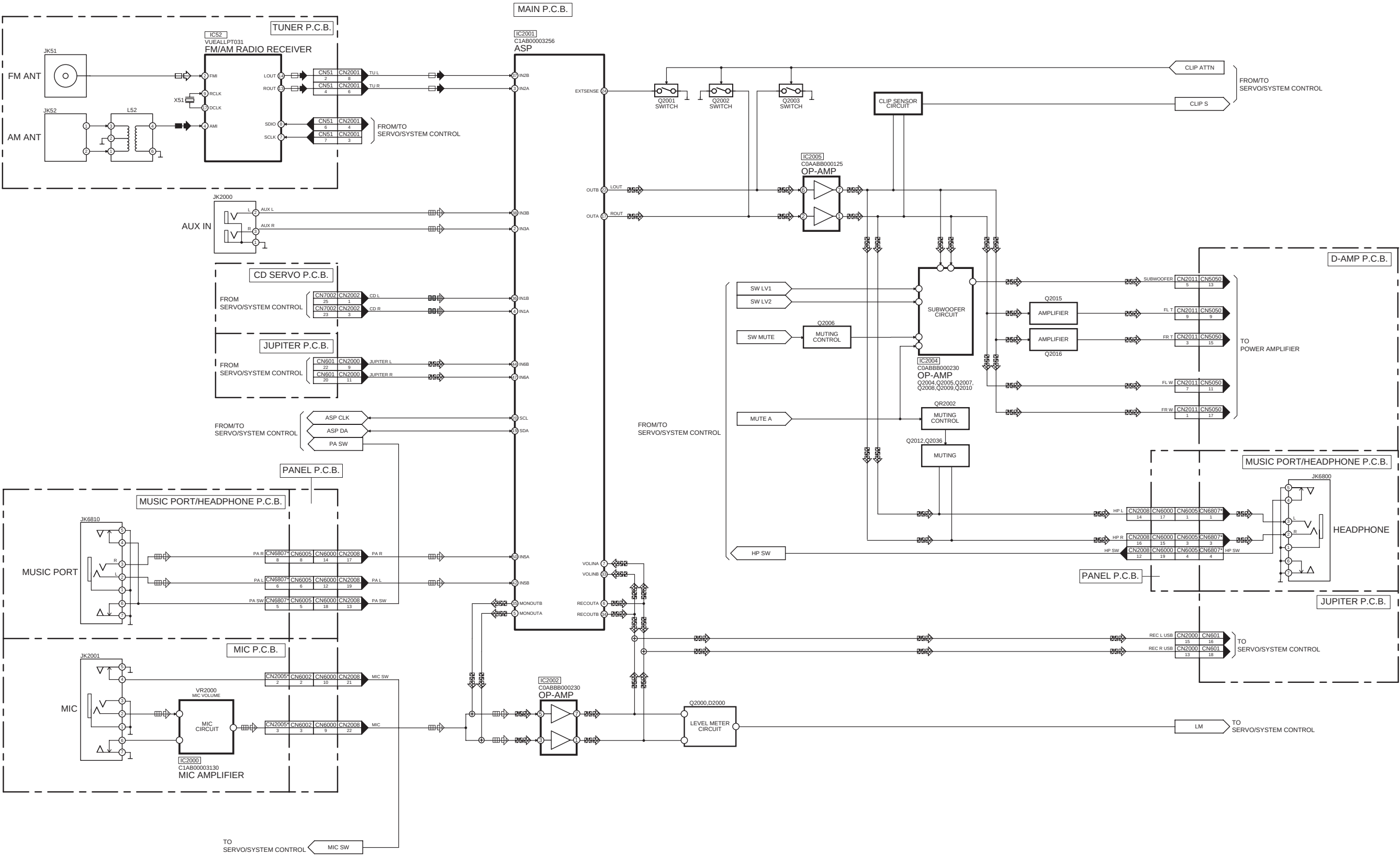
SA-AKX70PH/PN AUDIO BLOCK DIAGRAM
