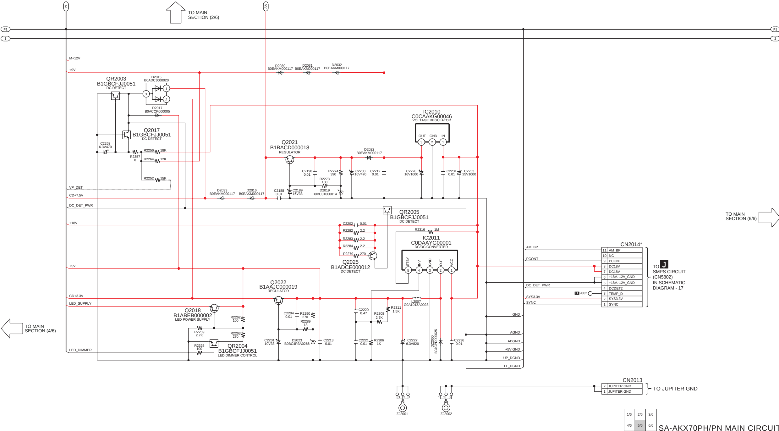
SA-AKX70PH/PN MAIN CIRCUIT
