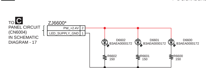
I TOP BAR LED CIRCUIT
