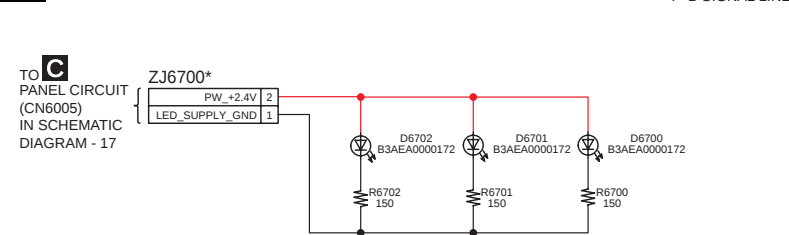
J BOTTOM BAR LED CIRCUIT
