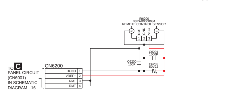
SCHEMATIC DIAGRAM - 18 D REMOTE SENSOR CIRCUIT
