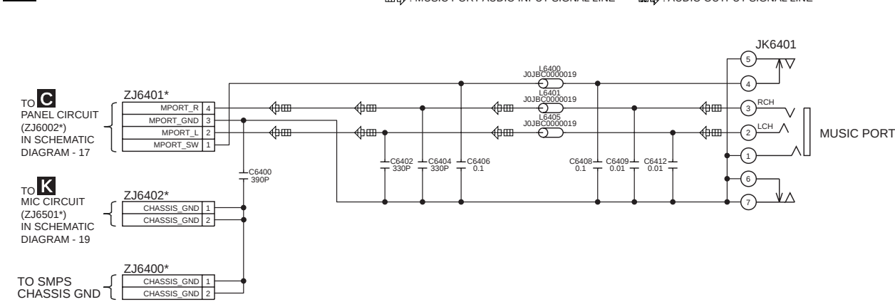
F MUSIC PORT CIRCUIT
