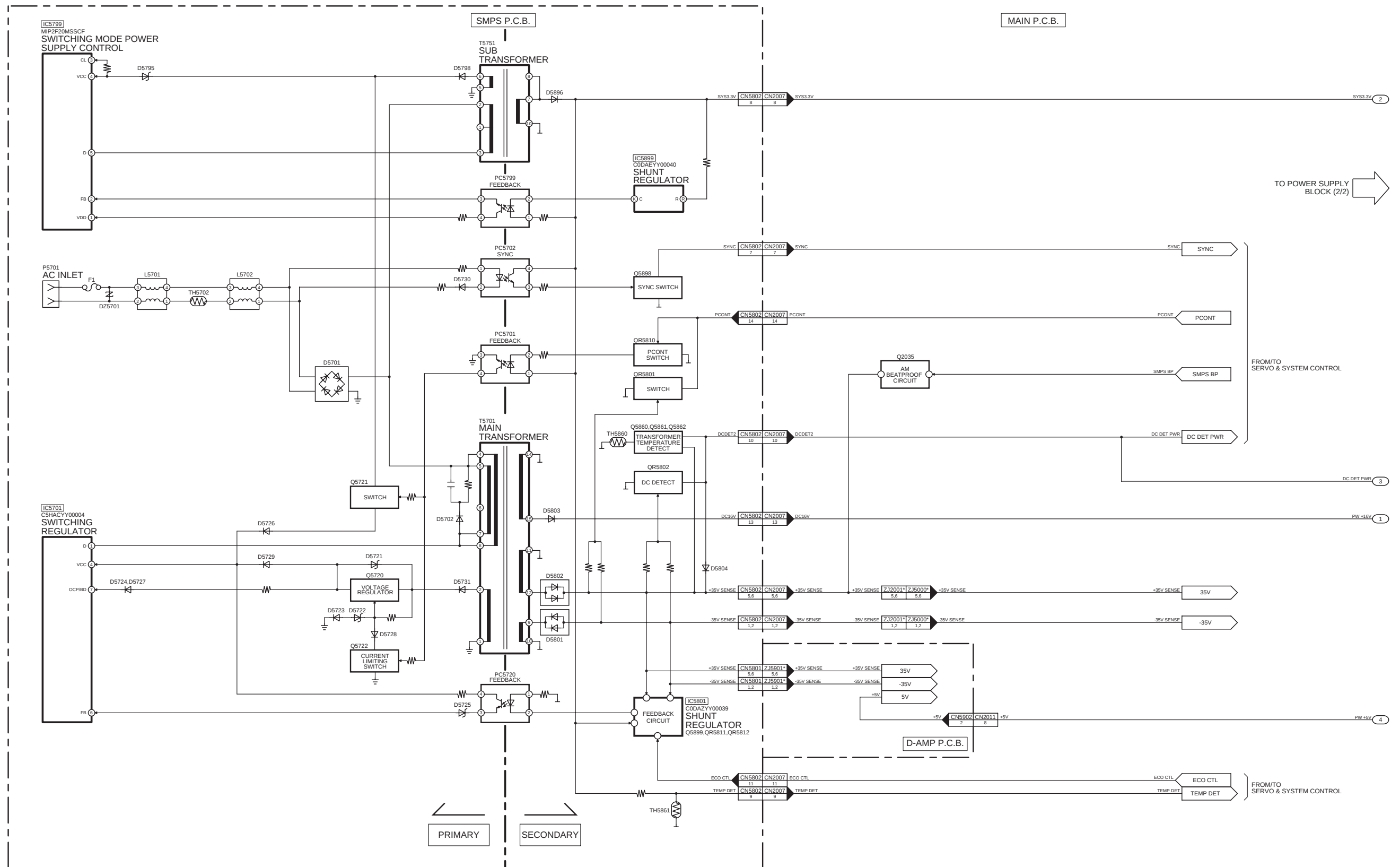
SA-AKX73P POWER SUPPLY (1/2) BLOCK DIAGRAM
