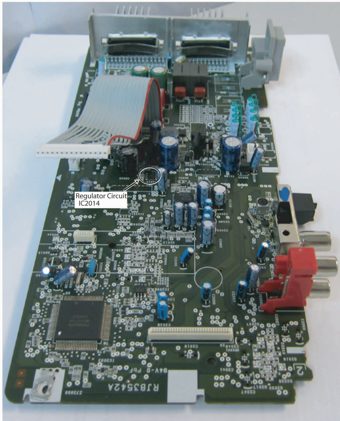
Fig. 2 Main P.C.B. (Front Side)
