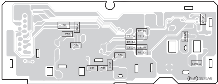
G TUNER P.C.B. (REP5297EB...AKX660PN) (REP5297AB...AKX880PN) (REP5297FB...AKX660PS) (REP5297BB...AKX880PS)
