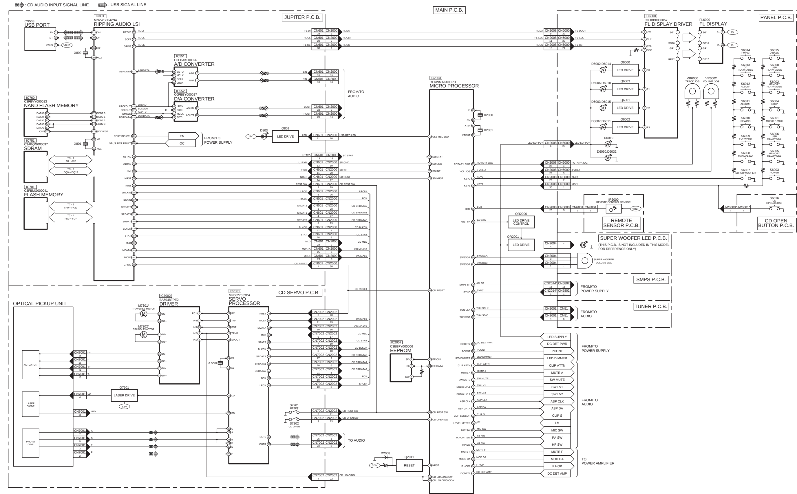
SA-AKX90PH/PR SERVO/SYSTEM CONTROL BLOCK DIAGRAM
