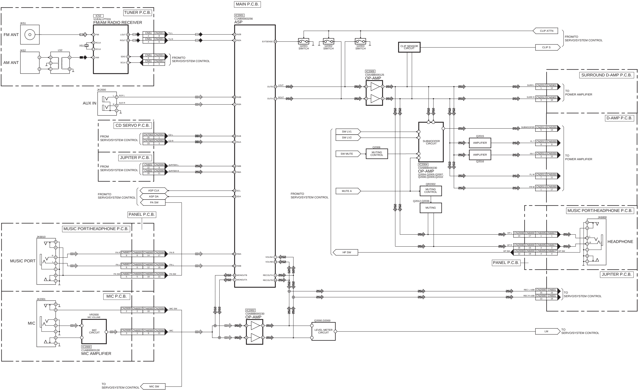
SA-AKX90PH/PR AUDIO BLOCK DIAGRAM
