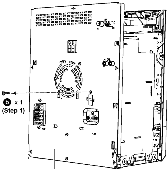
Rear Panel
