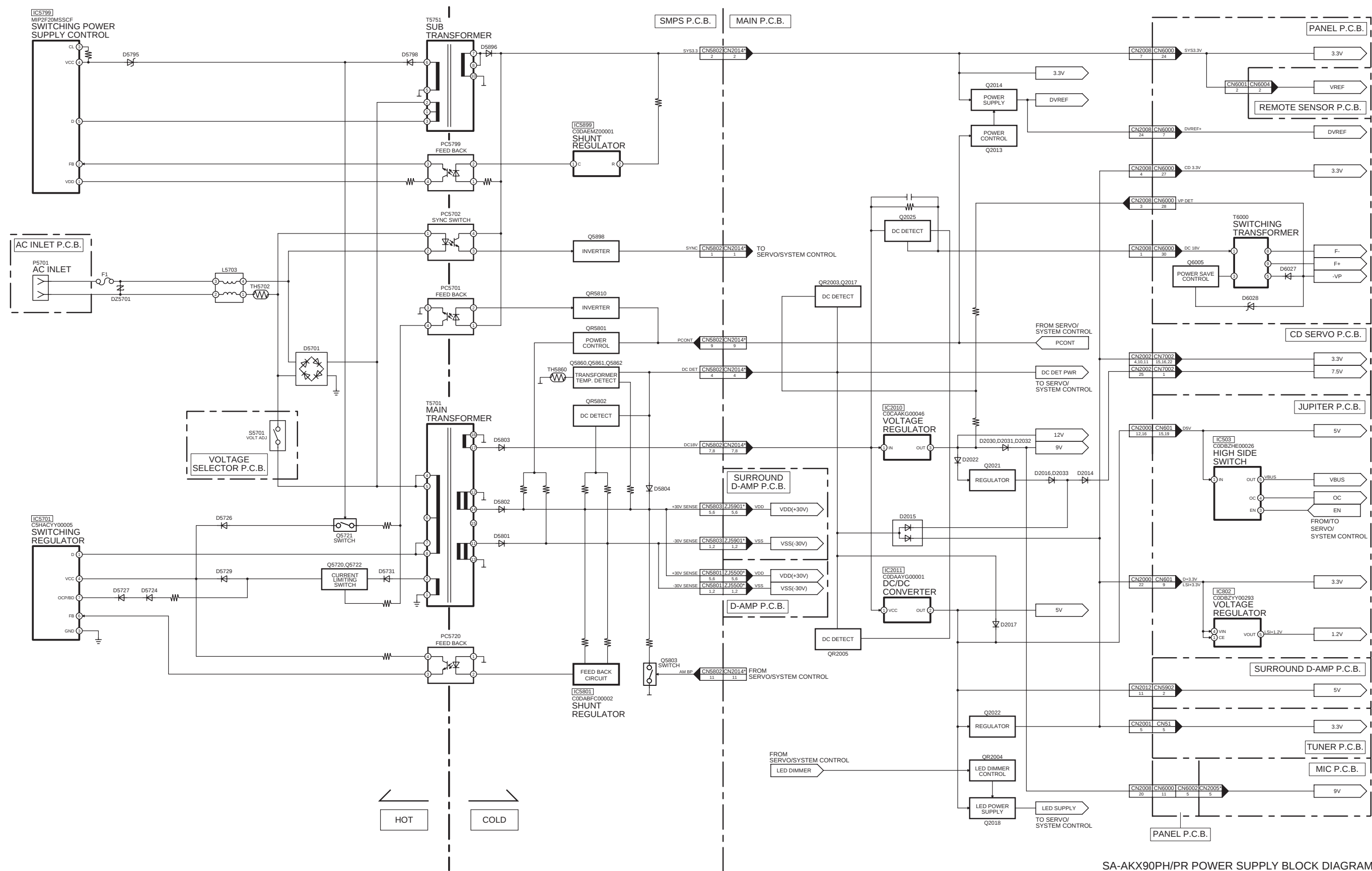
SA-AKX90PH/PR POWER SUPPLY BLOCK DIAGRAM
