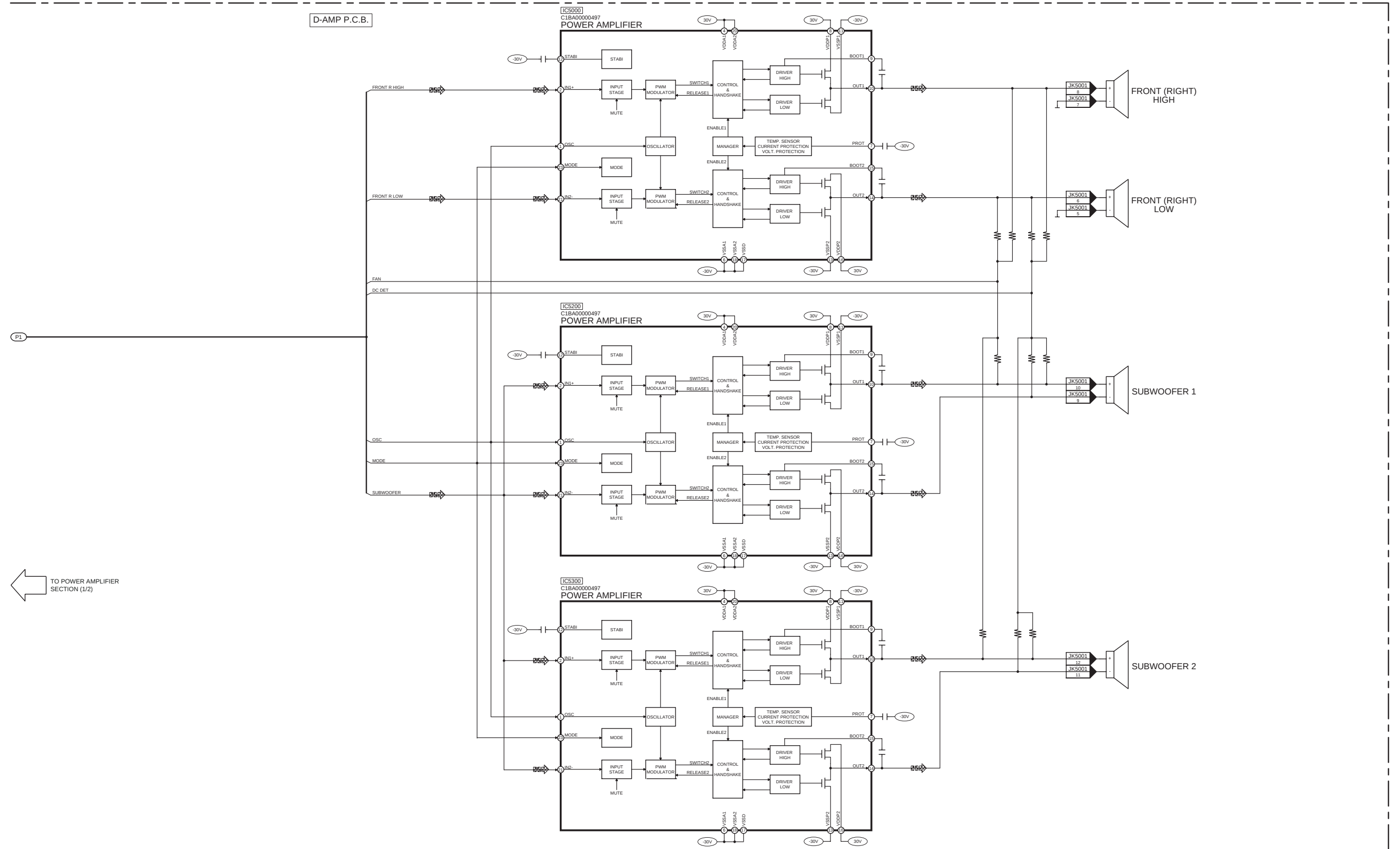
SA-AKX90PH/PR POWER AMPLIFIER (2/2) BLOCK DIAGRAM
