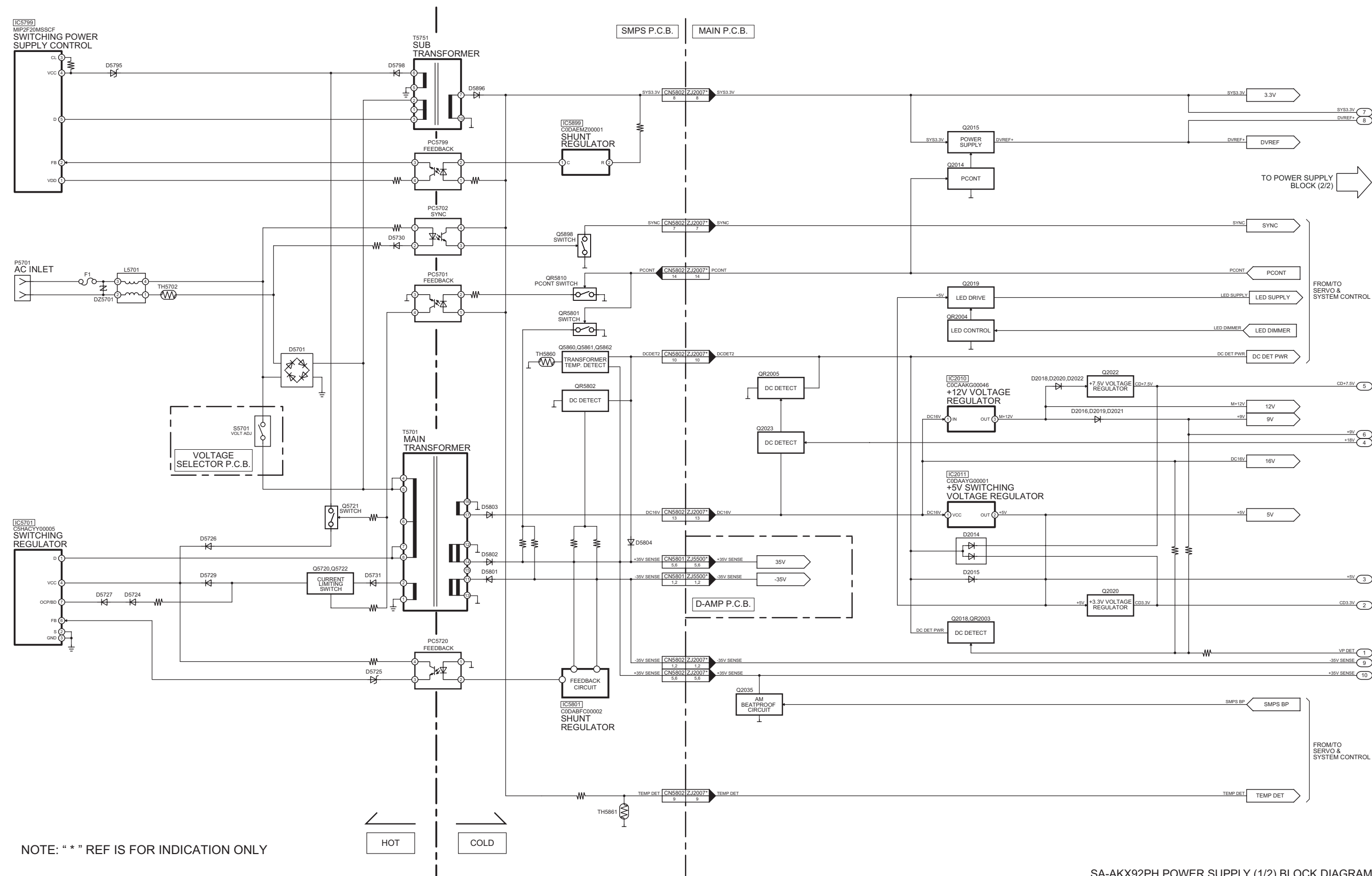
SA-AKX92PH POWER SUPPLY (1/2) BLOCK DIAGRAM
