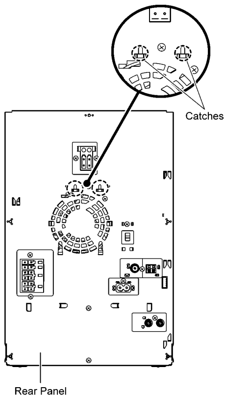
Rear Panel
