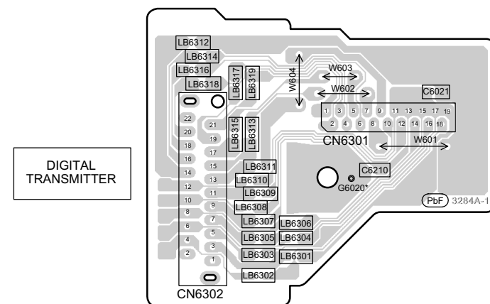
I WIRELESS ADAPTER P.C.B. (REP4371B)
