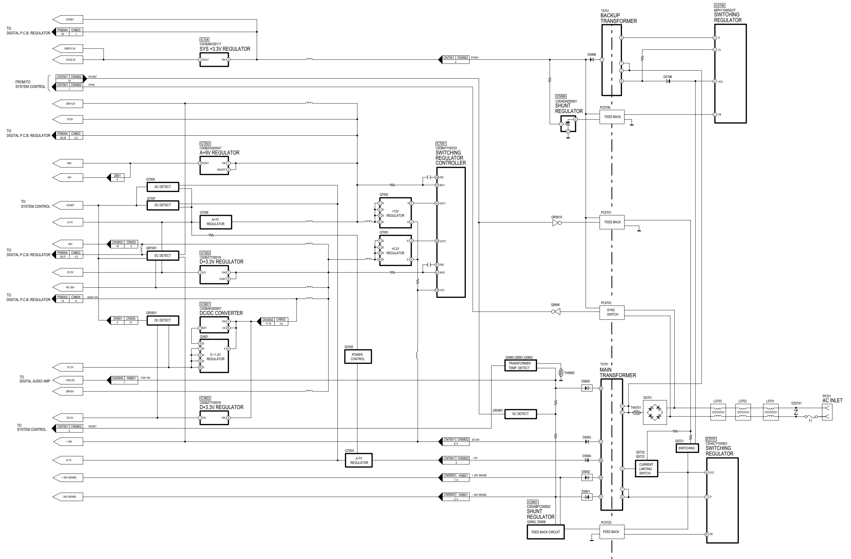
SA-BT100EB/EG POWER BLOCK DIAGRAM
