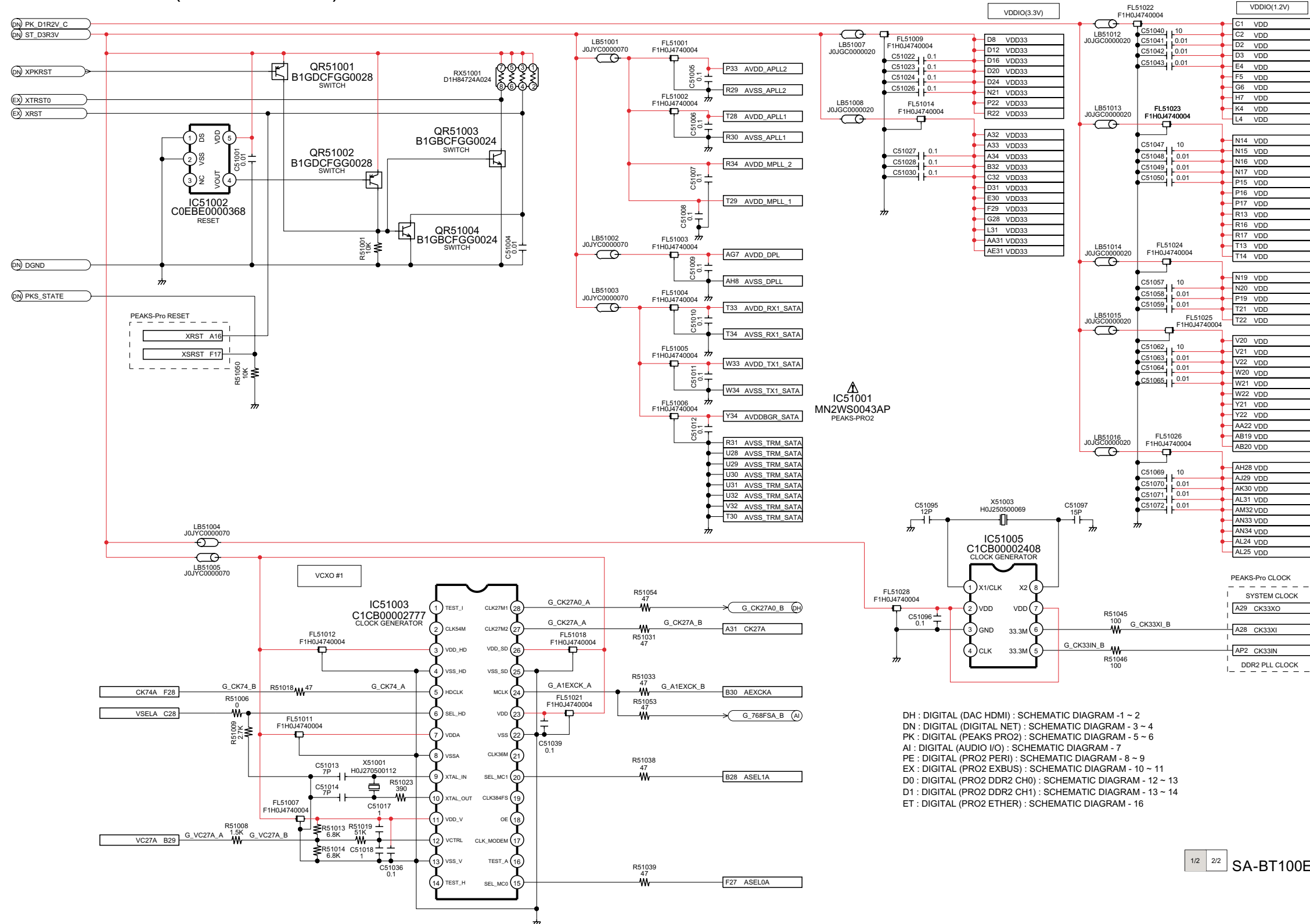
SCHEMATIC DIAGRAM - 5
