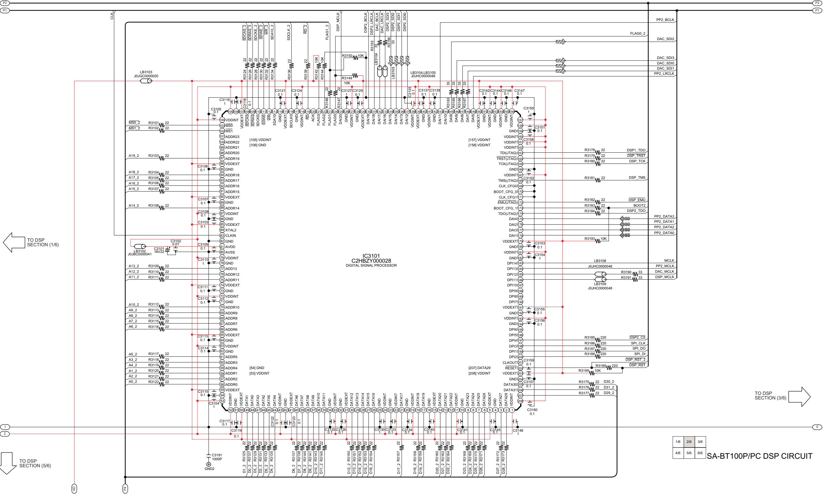
SCHEMATIC DIAGRAM - 18
