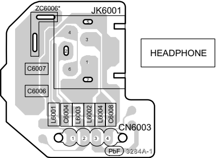
G HEADPHONE P.C.B. (REP4371A)
