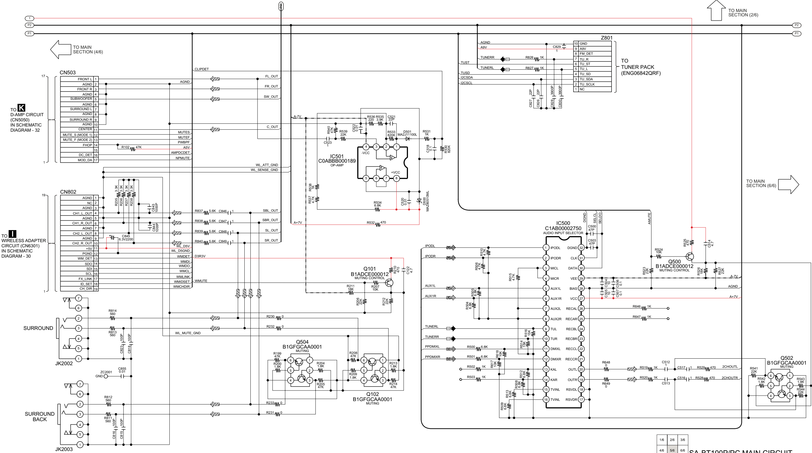
SCHEMATIC DIAGRAM - 27
