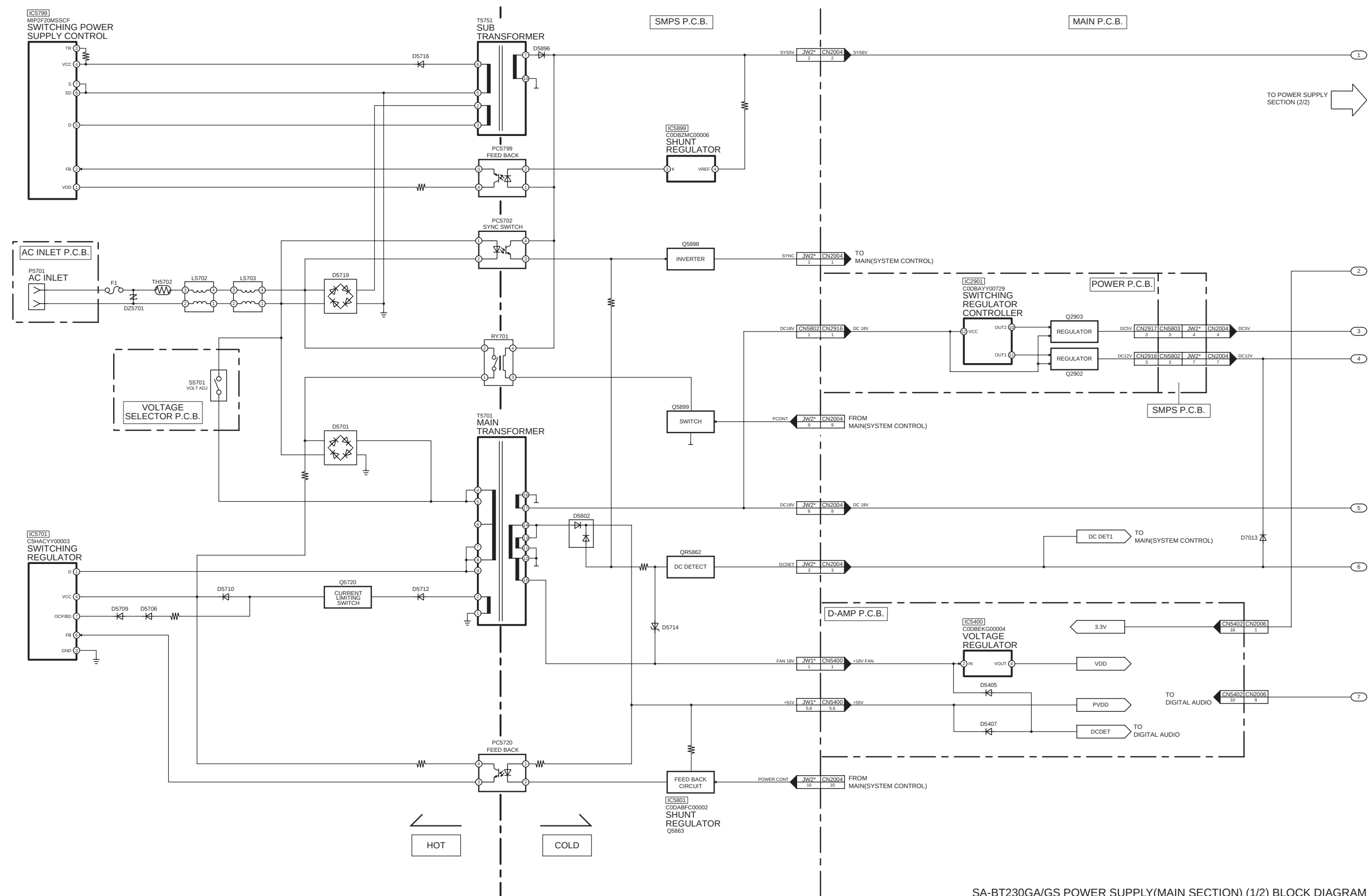
SA-BT230GA/GS POWER SUPPLY(MAIN SECTION) (1/2) BLOCK DIAGRAM
