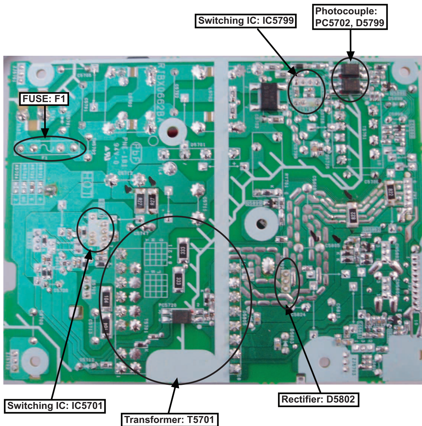
Figure 1. SMPS P.C.B.
