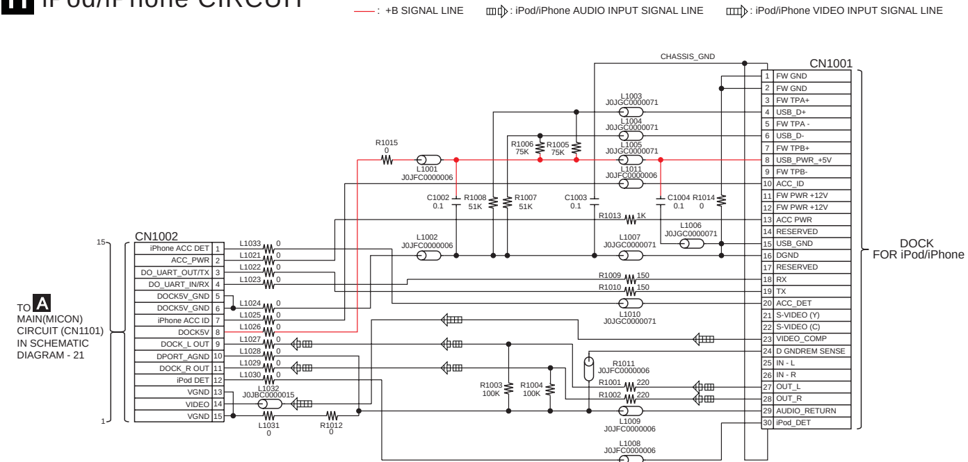
SCHEMATIC DIAGRAM - 33
