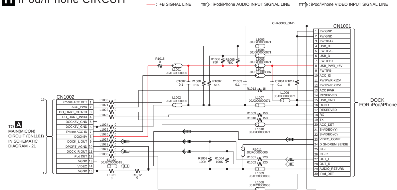
SCHEMATIC DIAGRAM - 34
