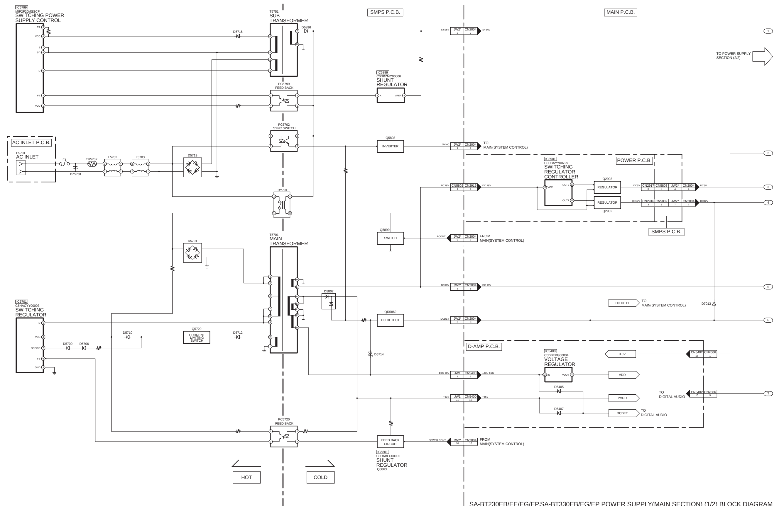
SA-BT230EB/EE/EG/EP,SA-BT330EB/EG/EP POWER SUPPLY(MAIN SECTION) (1/2) BLOCK DIAGRAM
