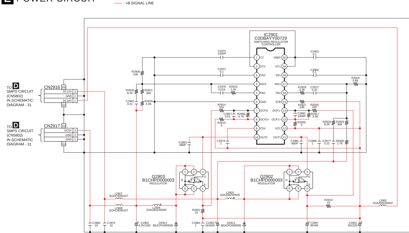
SCHEMATIC DIAGRAM - 33 E POWER CIRCUIT
