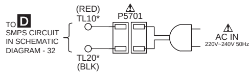
G AC INLET CIRCUIT
