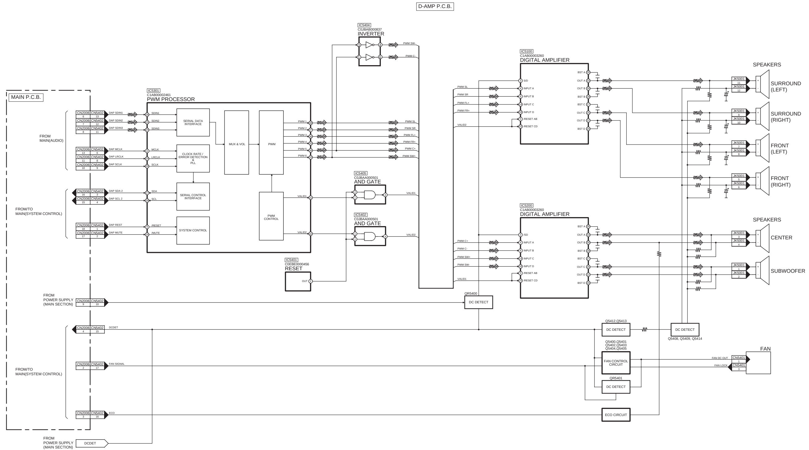
SA-BT230EB/EE/EG/EP,SA-BT330EB/EG/EP DIGITAL AUDIO BLOCK DIAGRAM
