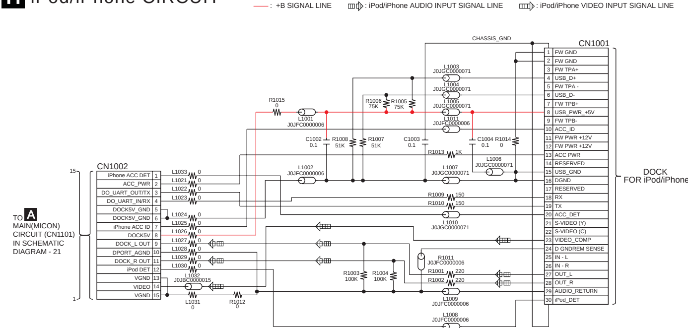
SCHEMATIC DIAGRAM - 34
