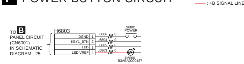
F POWER BUTTON CIRCUIT
