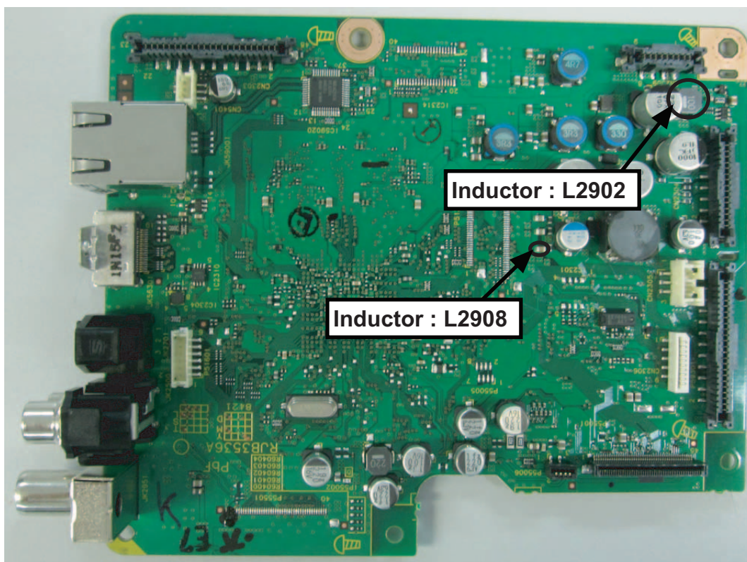
Fig 2. Digital P.C.B.
