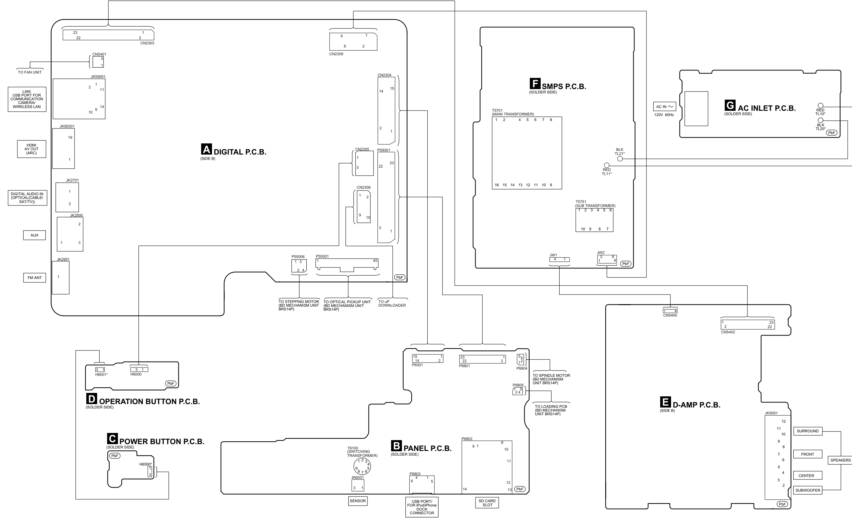
SA-BTT190P/PC,SA-BTT195P/PC,SA-BTT196P WIRING CONNECTION DIAGRAM
