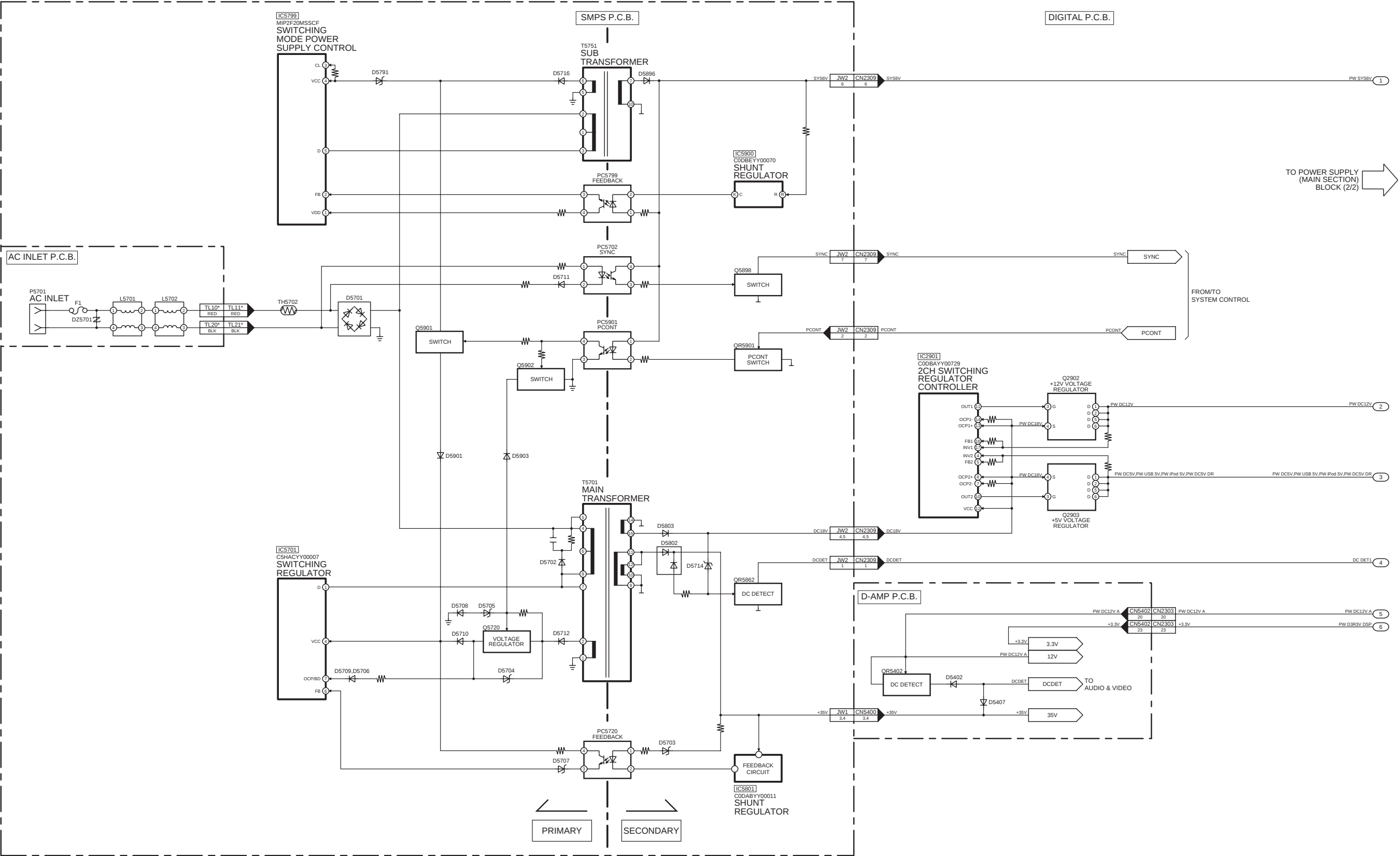
NOTE: " * " REF IS FOR INDICATION ONLY SA-BTT190P/PC,SA-BTT195P/PC,SA-BTT196P POWER SUPPLY(MAIN SECTION) (1/2) BLOCK DIAGRAM
