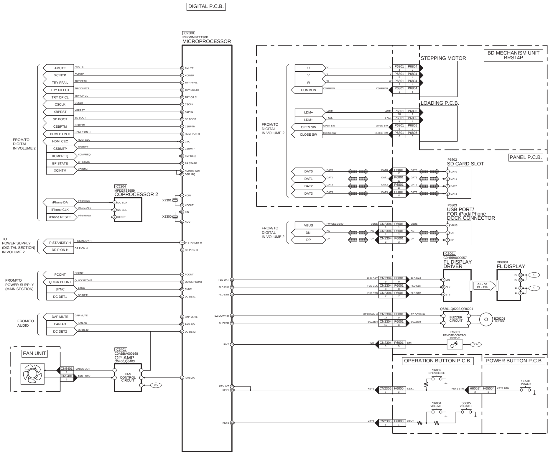
SA-BTT190P/PC,SA-BTT195P/PC,SA-BTT196P SYSTEM CONTROL BLOCK DIAGRAM
