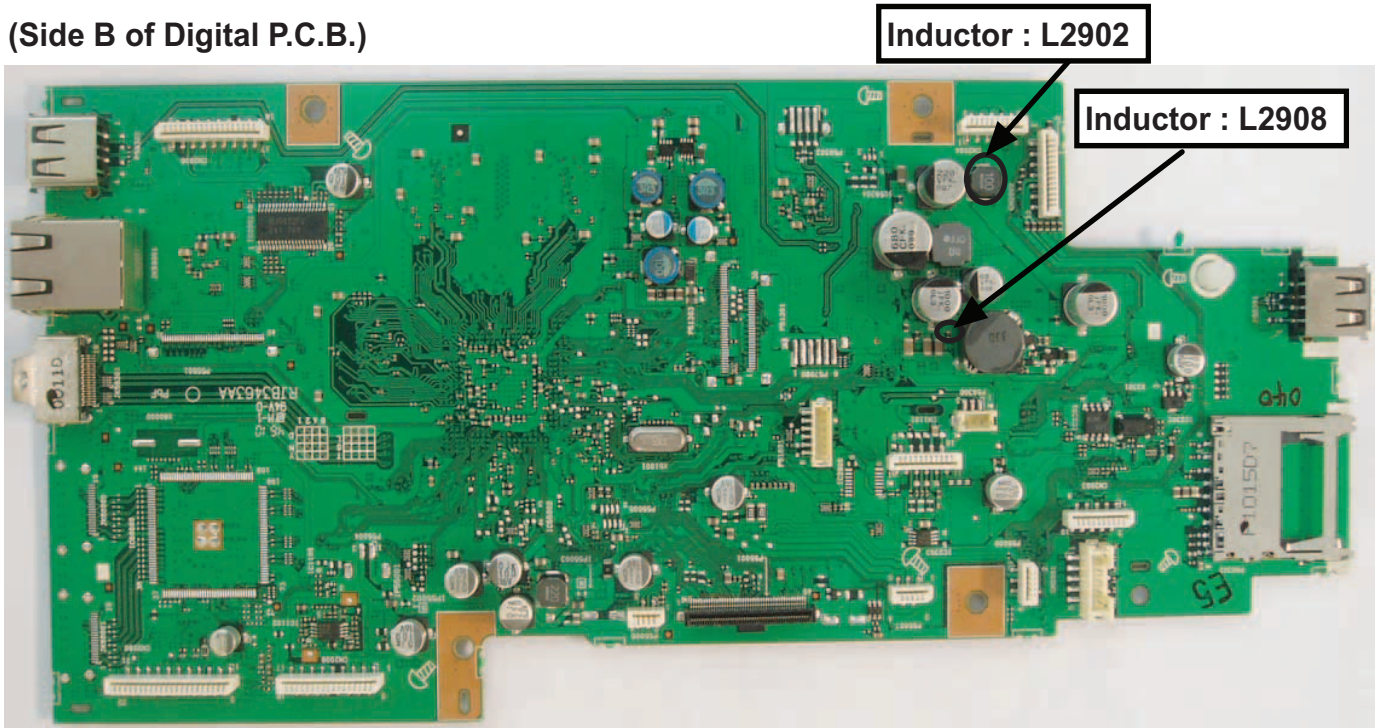
Fig 2. Digital P.C.B.
