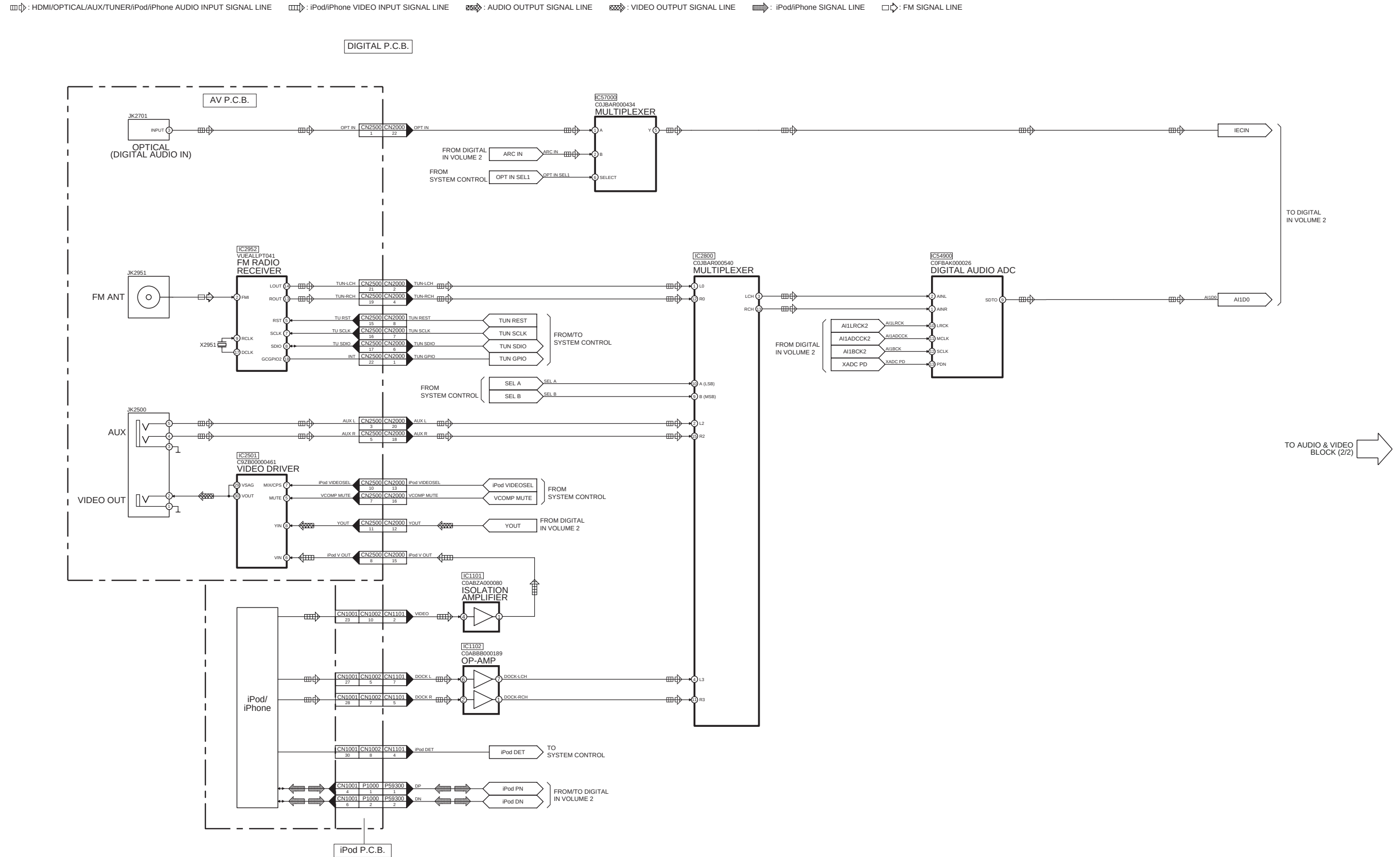
SA-BTT262EB/EG AUDIO & VIDEO (1/2) BLOCK DIAGRAM
