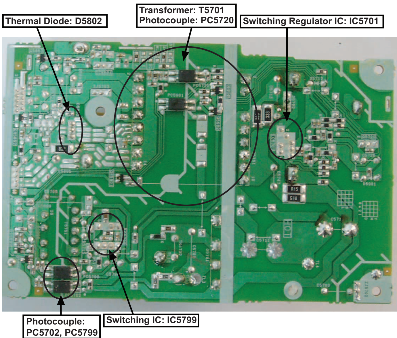
Figure 1. SMPS P.C.B.
