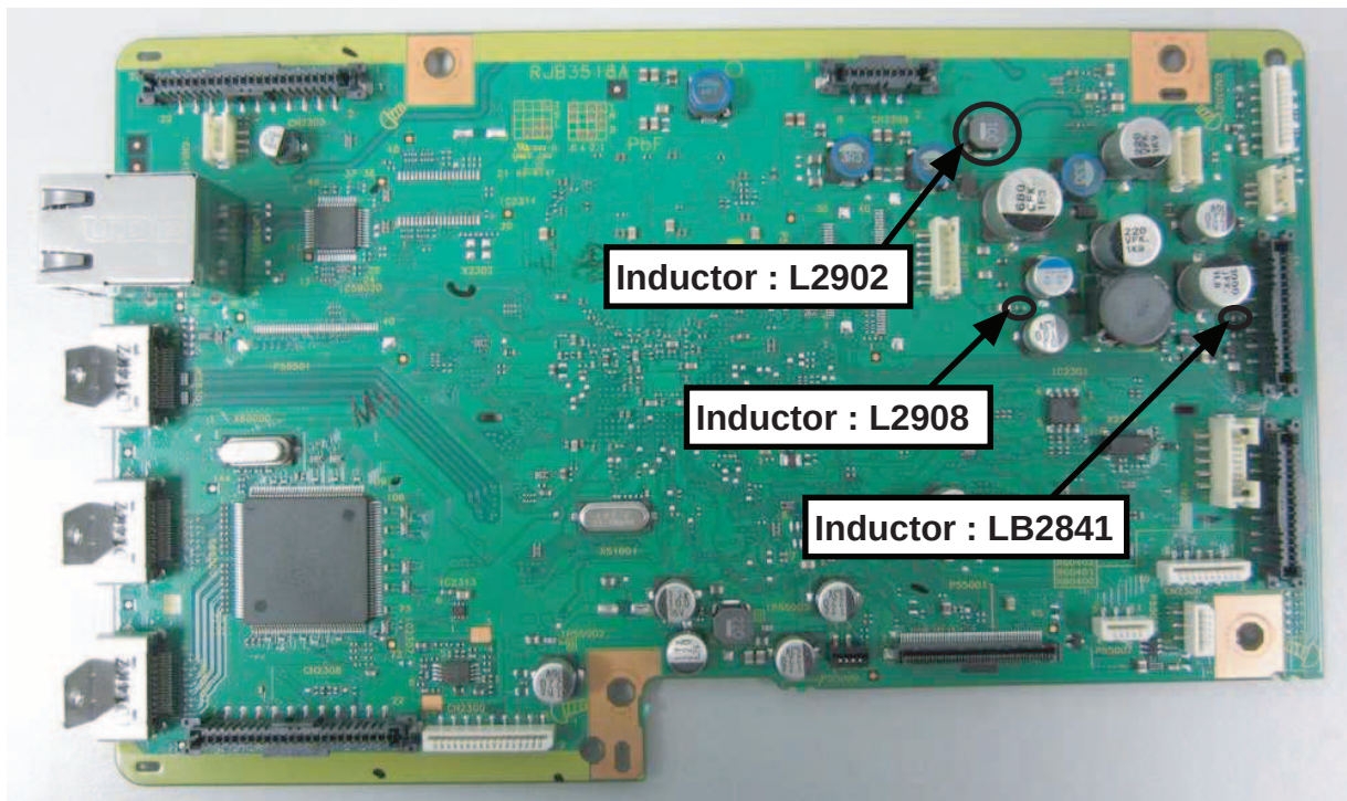
Fig 2. Digital P.C.B.
