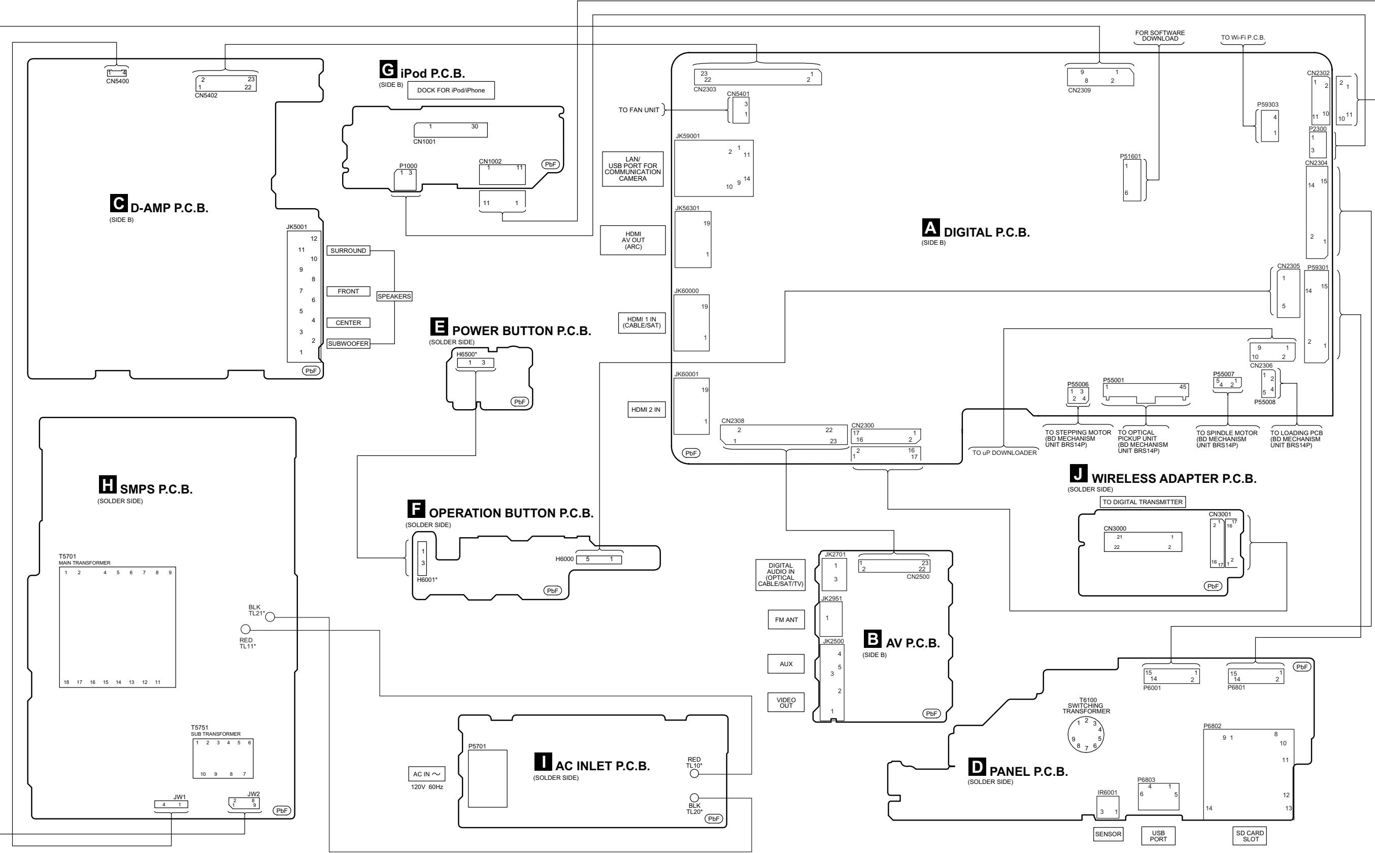
SA-BTT490P/PC WIRING CONNECTION DIAGRAM
