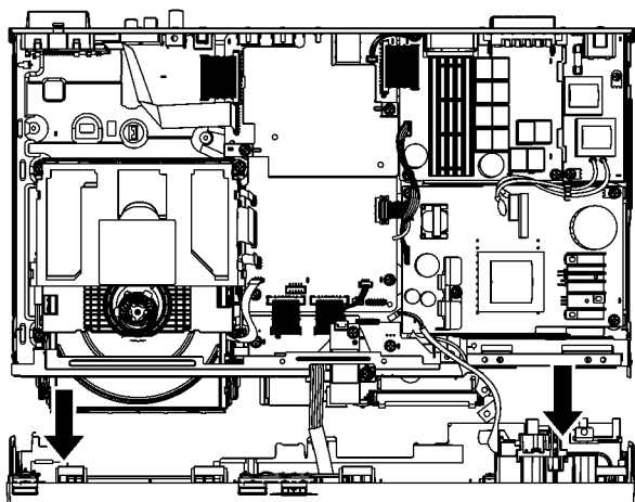
Front Panel Block Assembly (Step 8)
