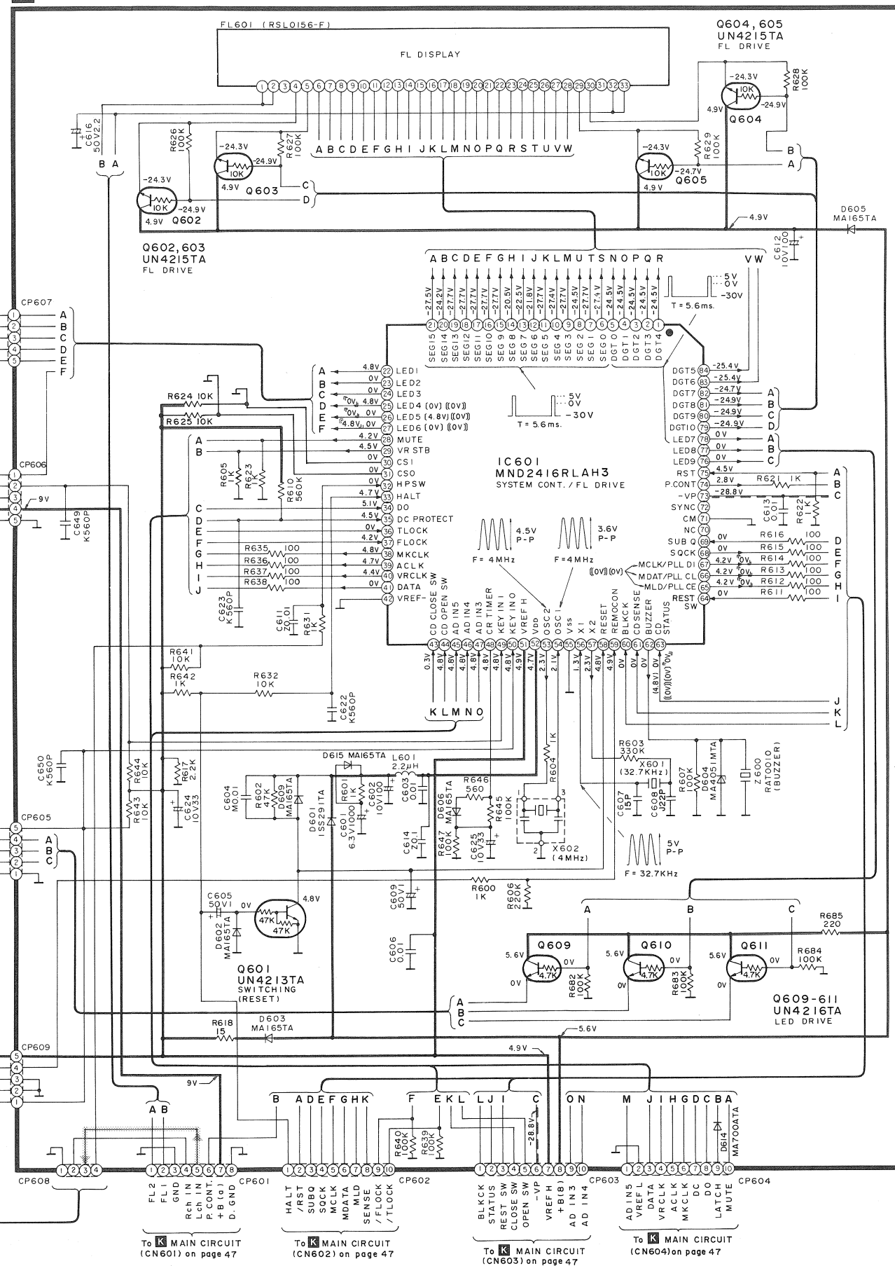
I FL CIRCUIT
