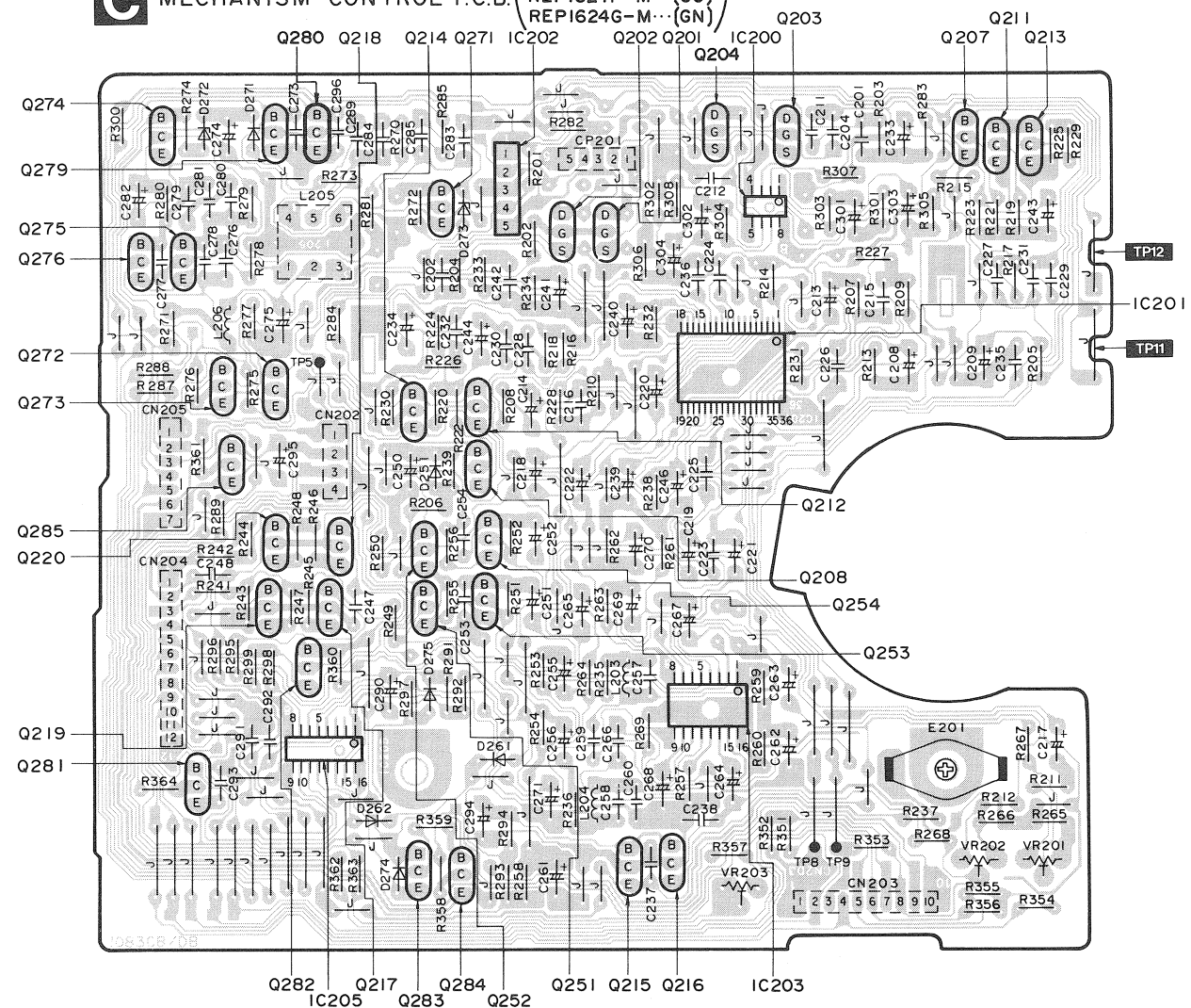
C MECHANISM CONTROL P.C.B. (REPI624C-M... (E), REPI624D-M... (EB), REPI624E-M... (EG), REPI624F-M... (GC), REPI624G-M... (GN))
