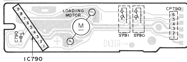
J LOADING MOTOR P.C.B.(REP0767)
