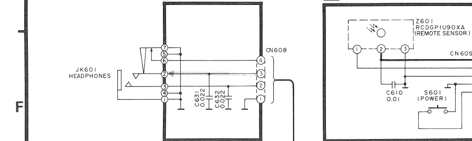
G HEADPHONE JACK CIRCUIT
