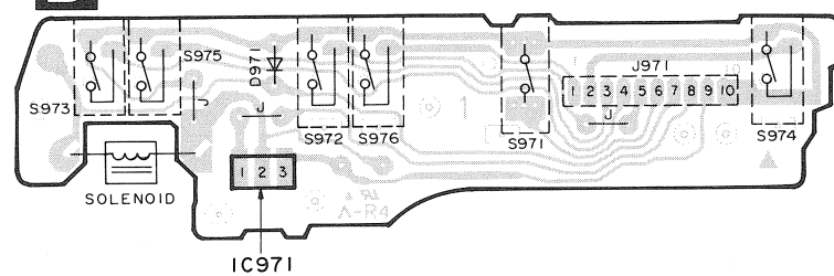
D MECHANISM P.C.B. (REP0075)
