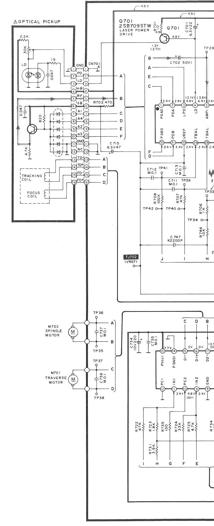
A SERVO CIRCUIT
