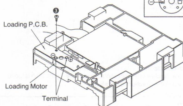
Loading Motor
