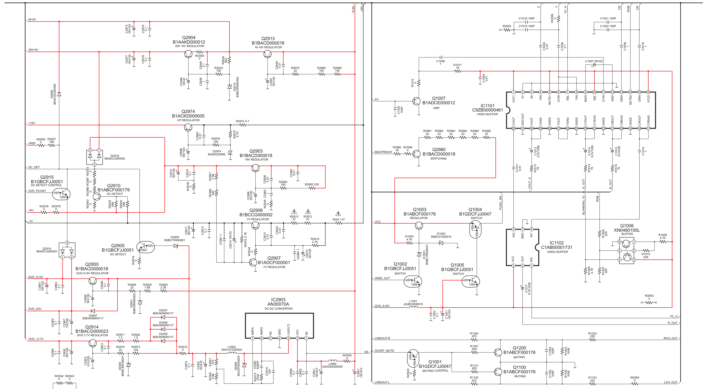
SA-HT340EE MAIN CIRCUIT
