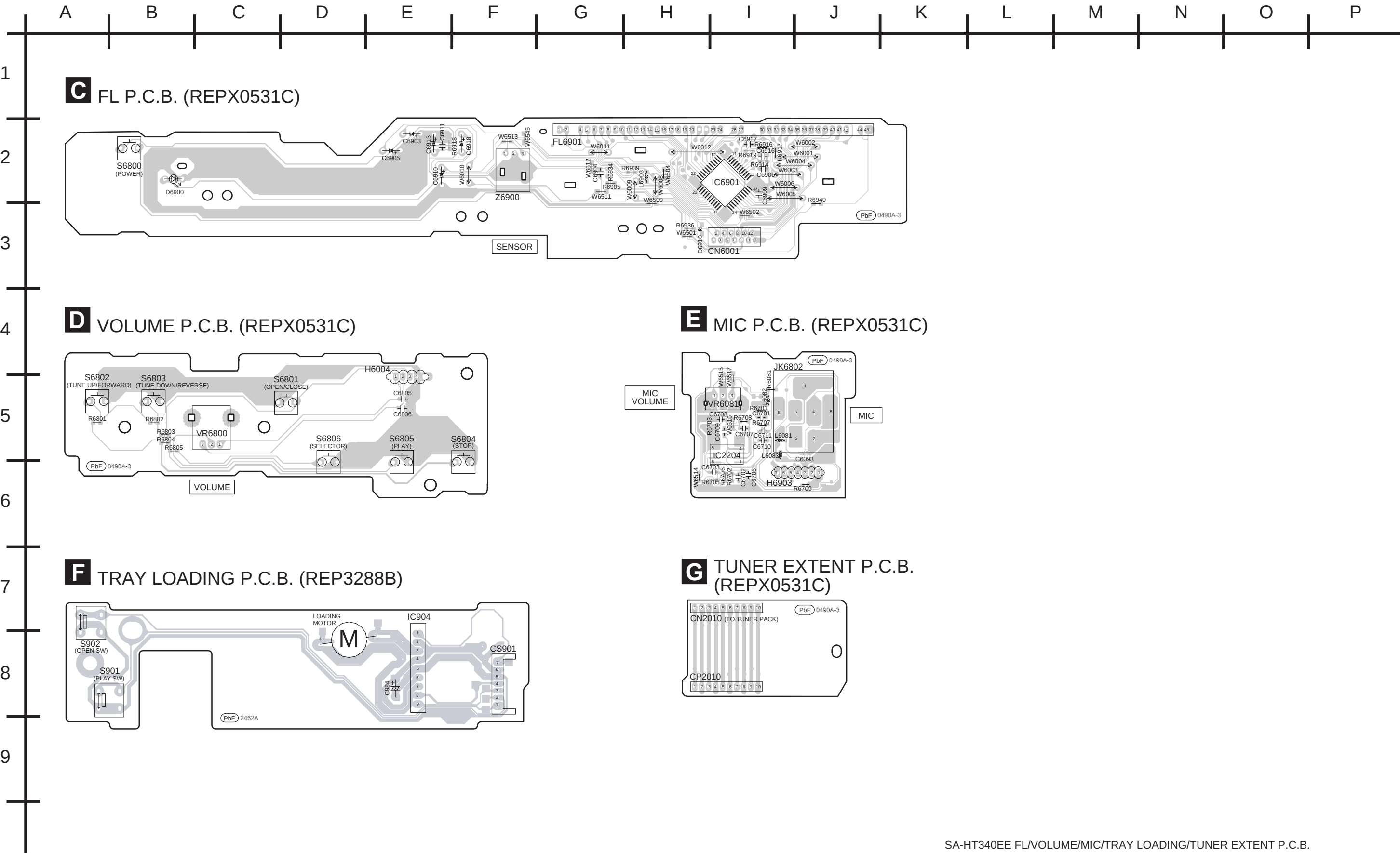
SA-HT340EE FL/VOLUME/MIC/TRAY LOADING/TUNER EXTENT P.C.B.
