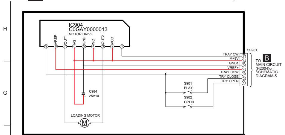
SCHEMATIC DIAGRAM-11
