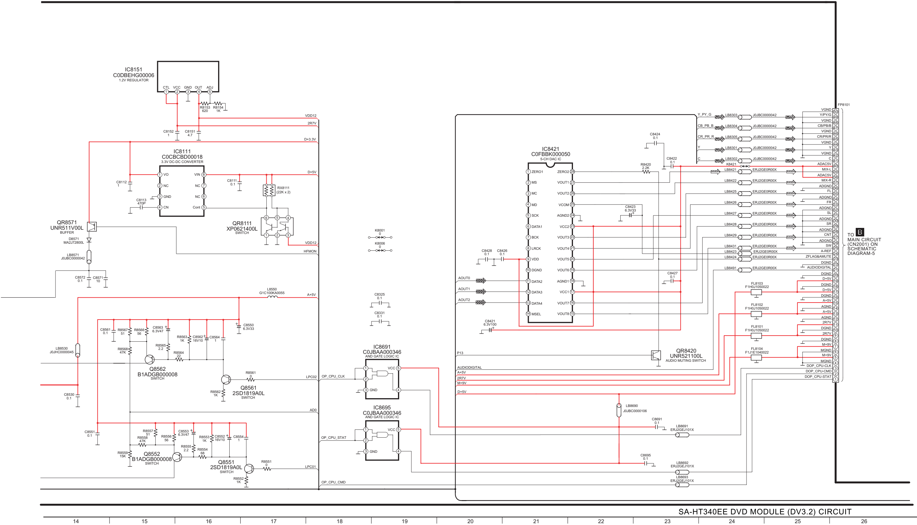
SCHEMATIC DIAGRAM-2
