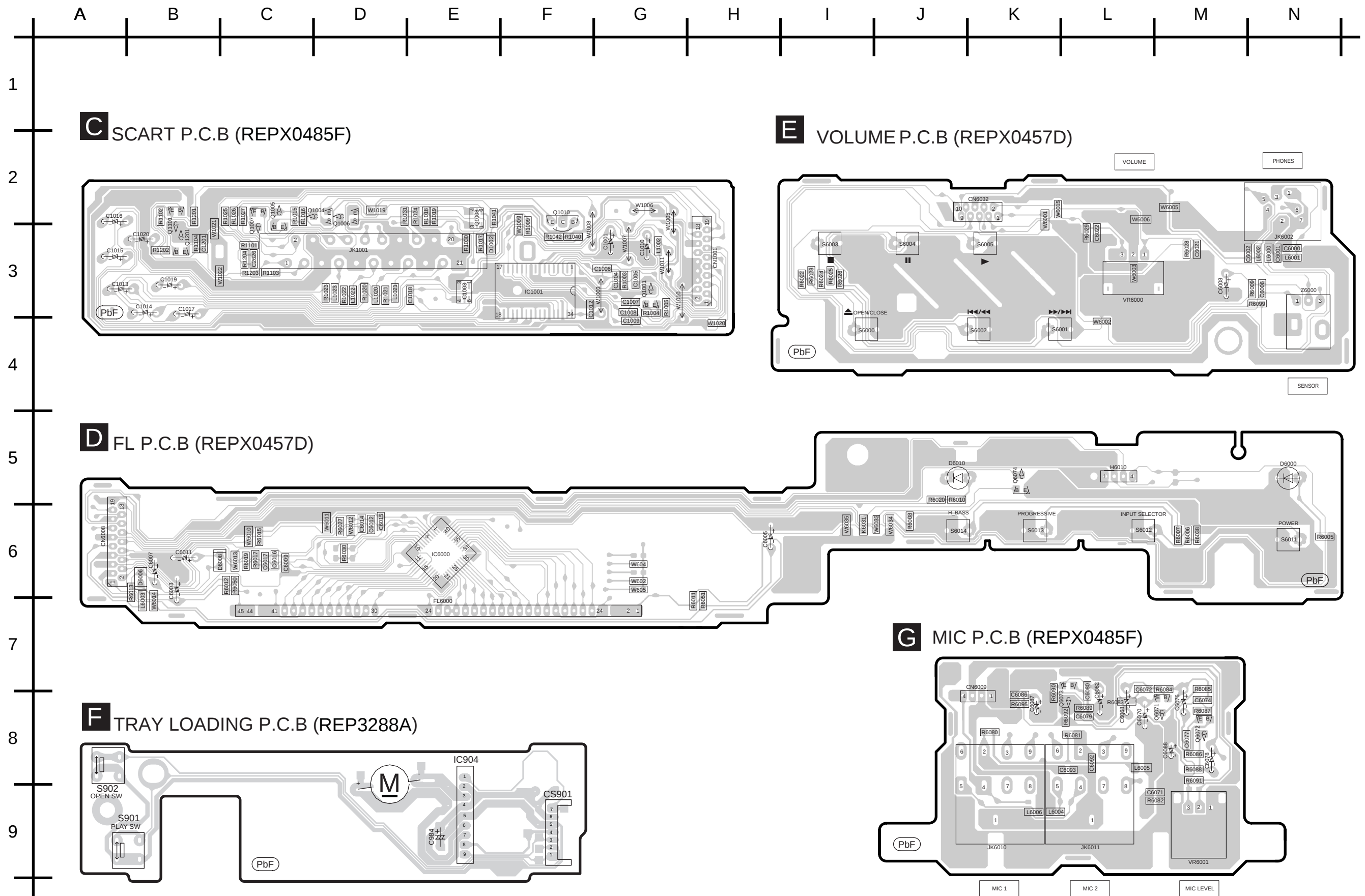
SA-HT845EE SCART/VOLUME/TRAY LOADING/FL/MIC P.C.B.
