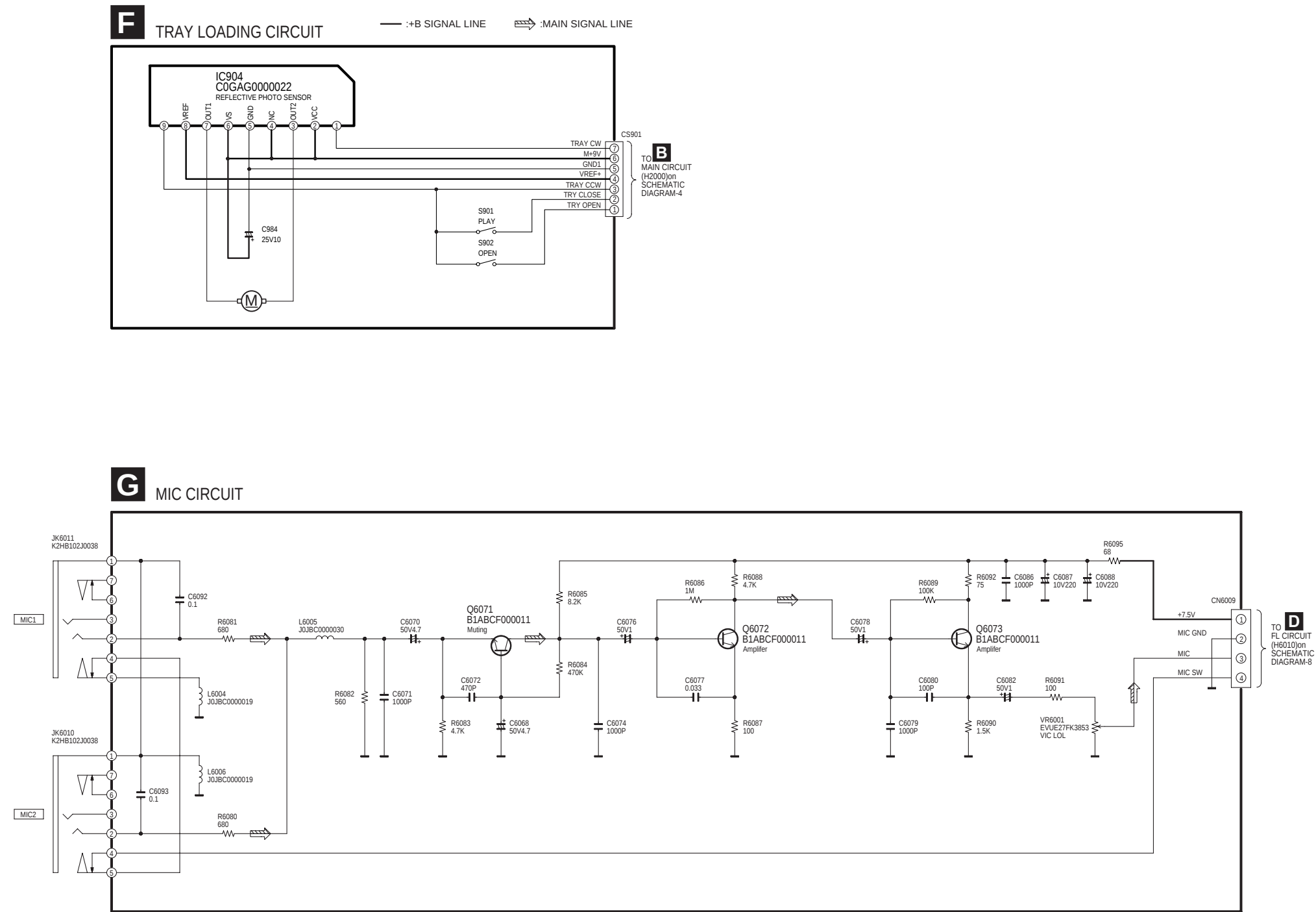
SCHEMATIC DIAGRAM-9
