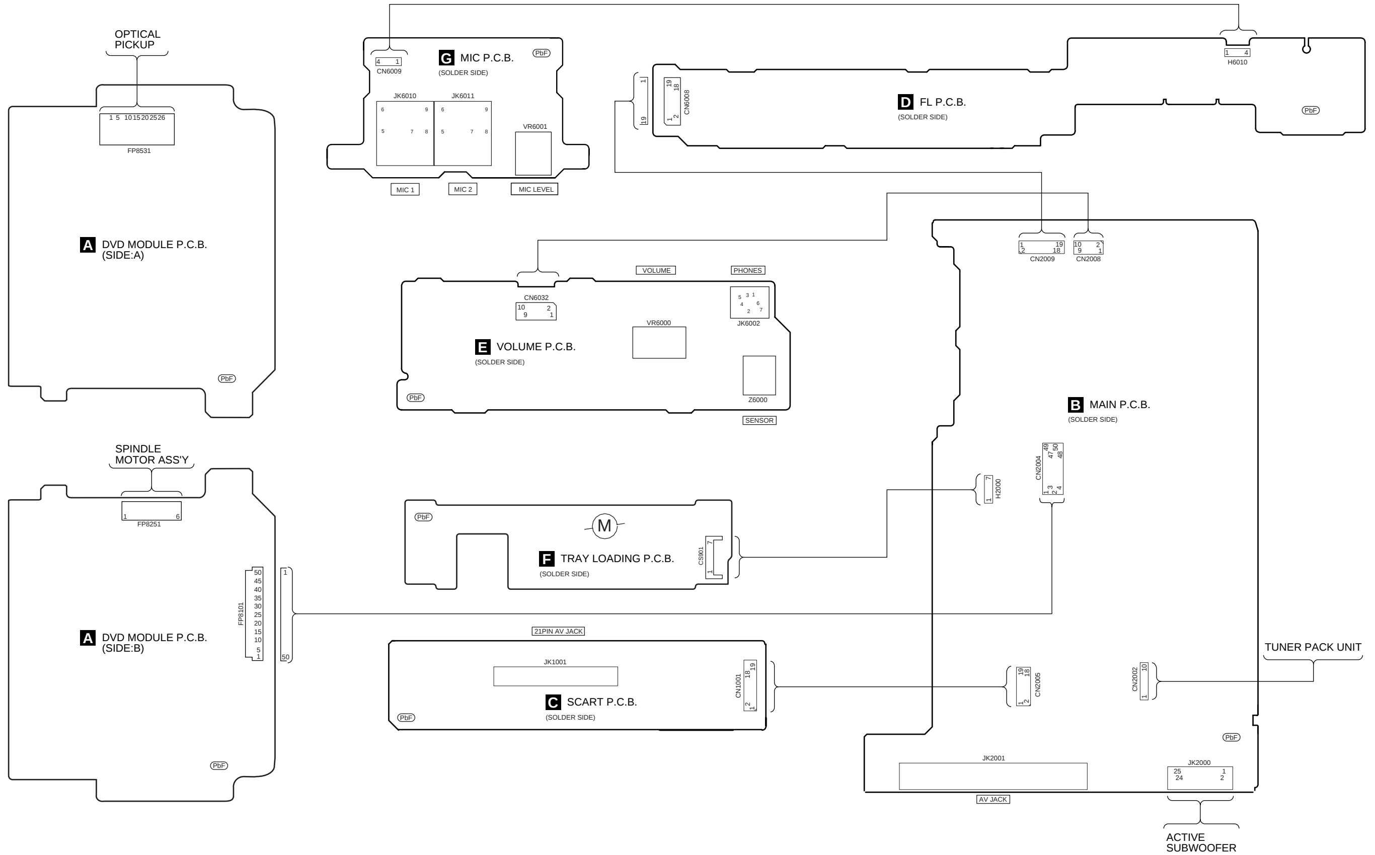
SA-HT845EE WIRING CONNECTION
