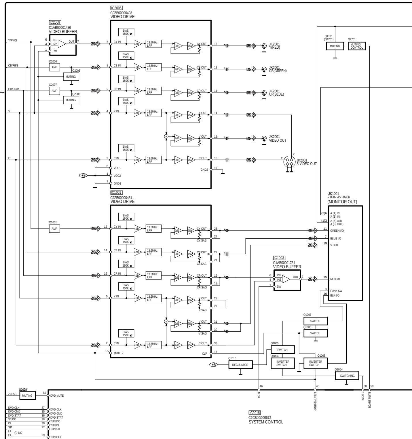
SA-HT845EE BLOCK DIAGRAM
