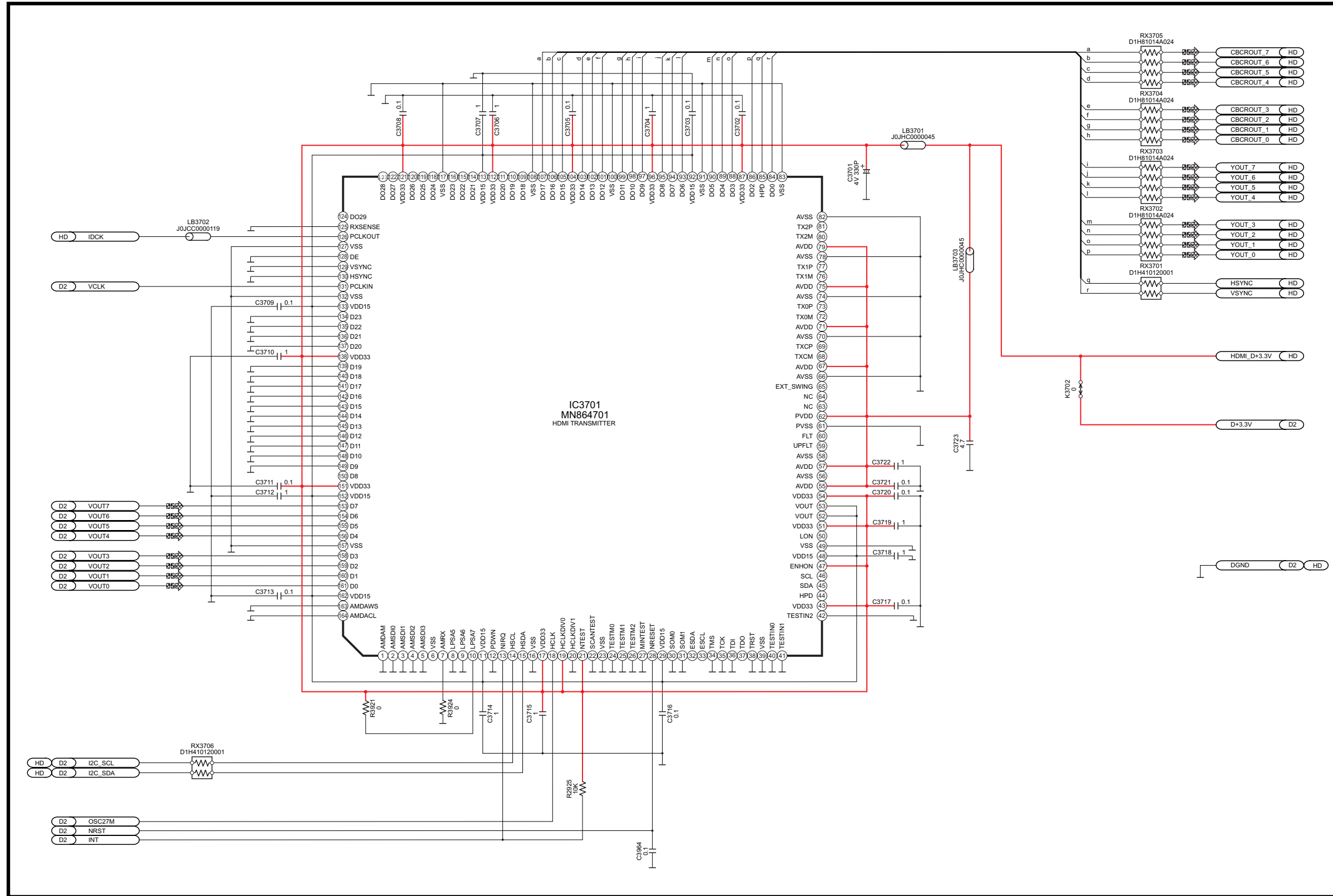
SA-HT855E/EB/EG HDMI MODULE CIRCUIT (UP)
