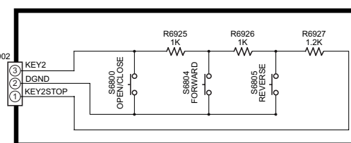
F TOP BUTTON CIRCUIT
