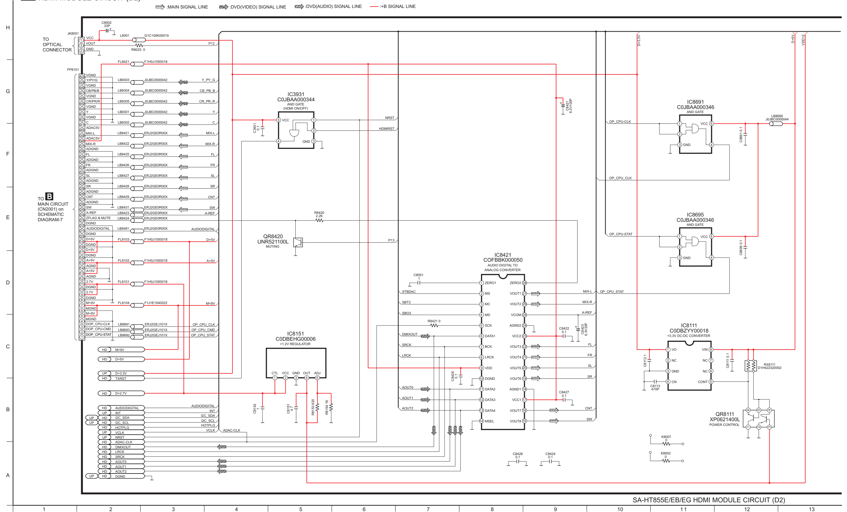
SCHEMATIC DIAGRAM-1
