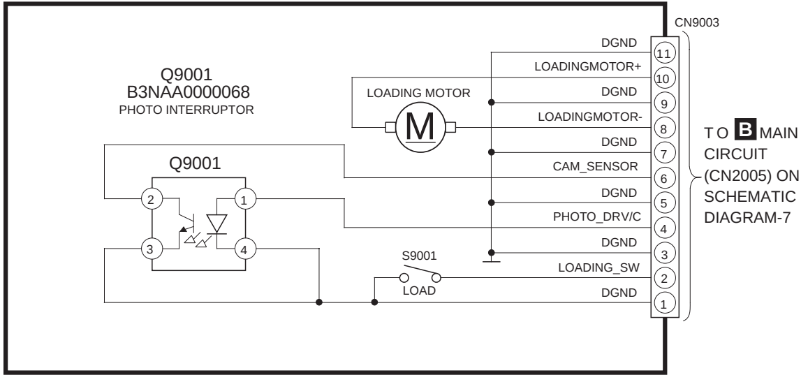
H LOADING MOTOR CIRCUIT
