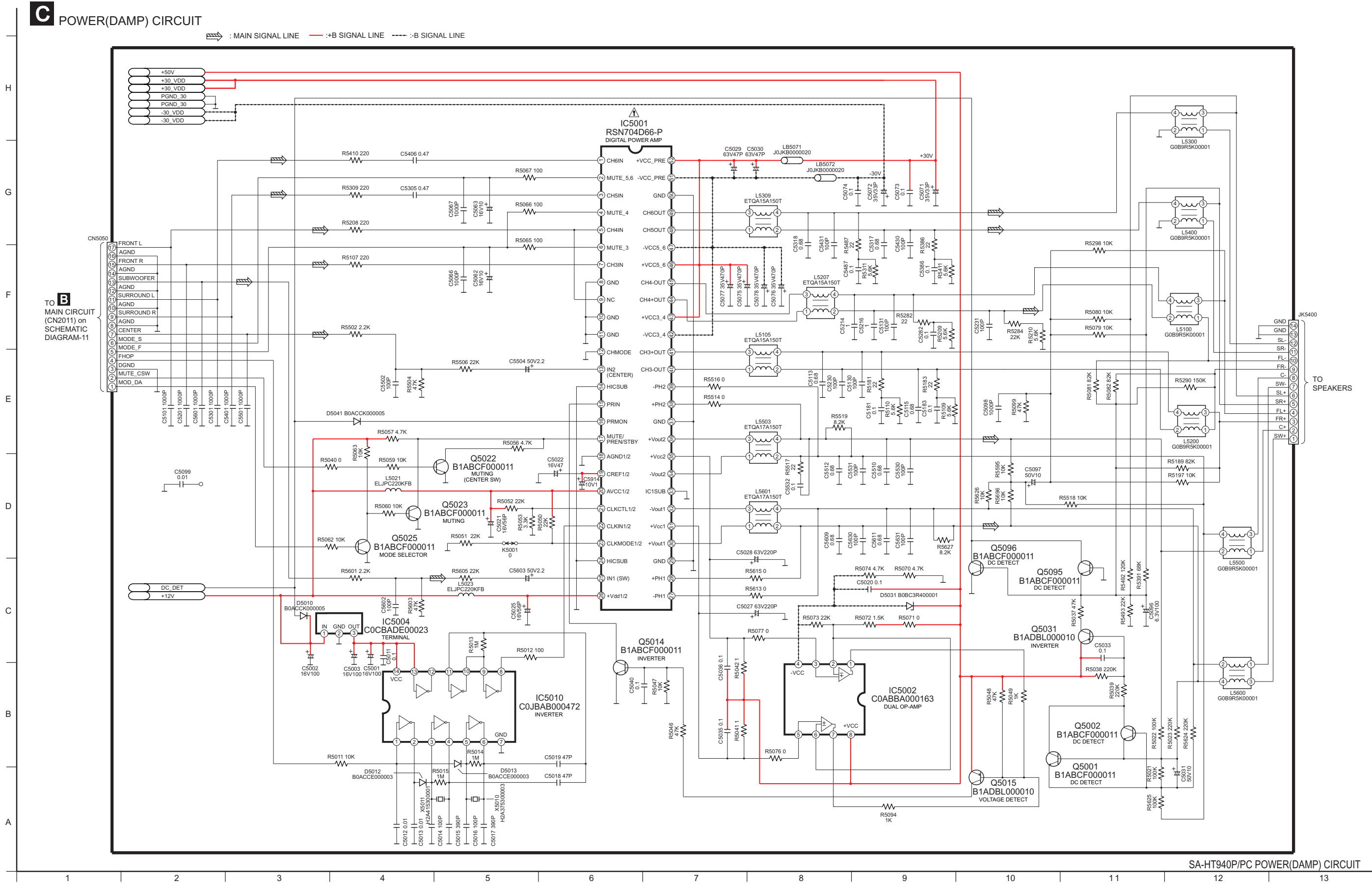
SCHEMATIC DIAGRAM-12
