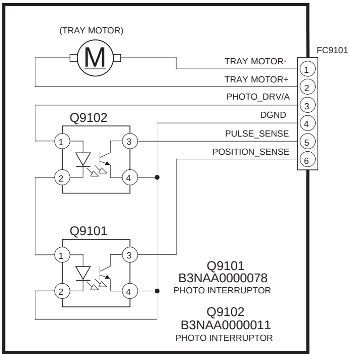
I TRAY MOTOR CIRCUIT
