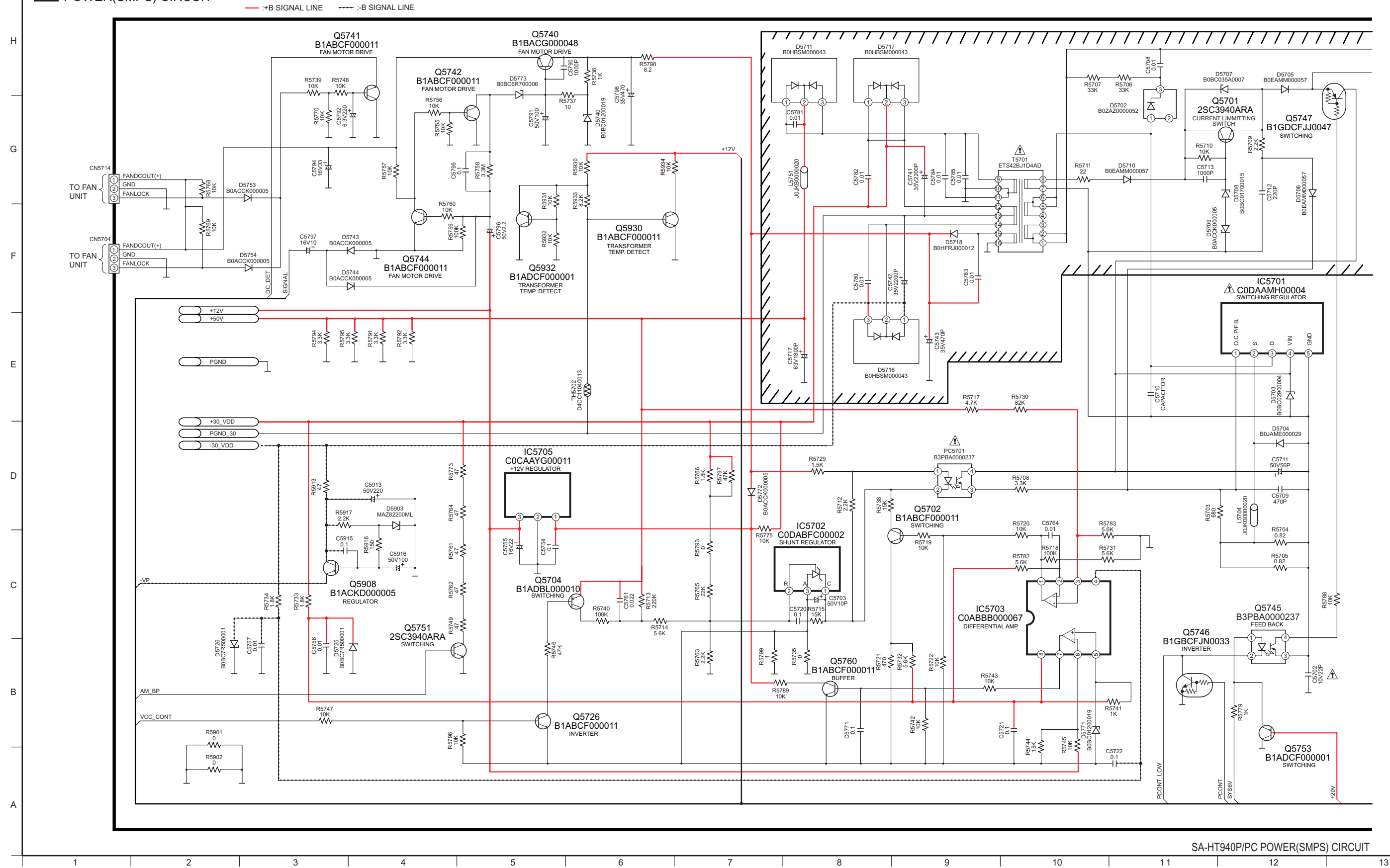
SCHEMATIC DIAGRAM-13
