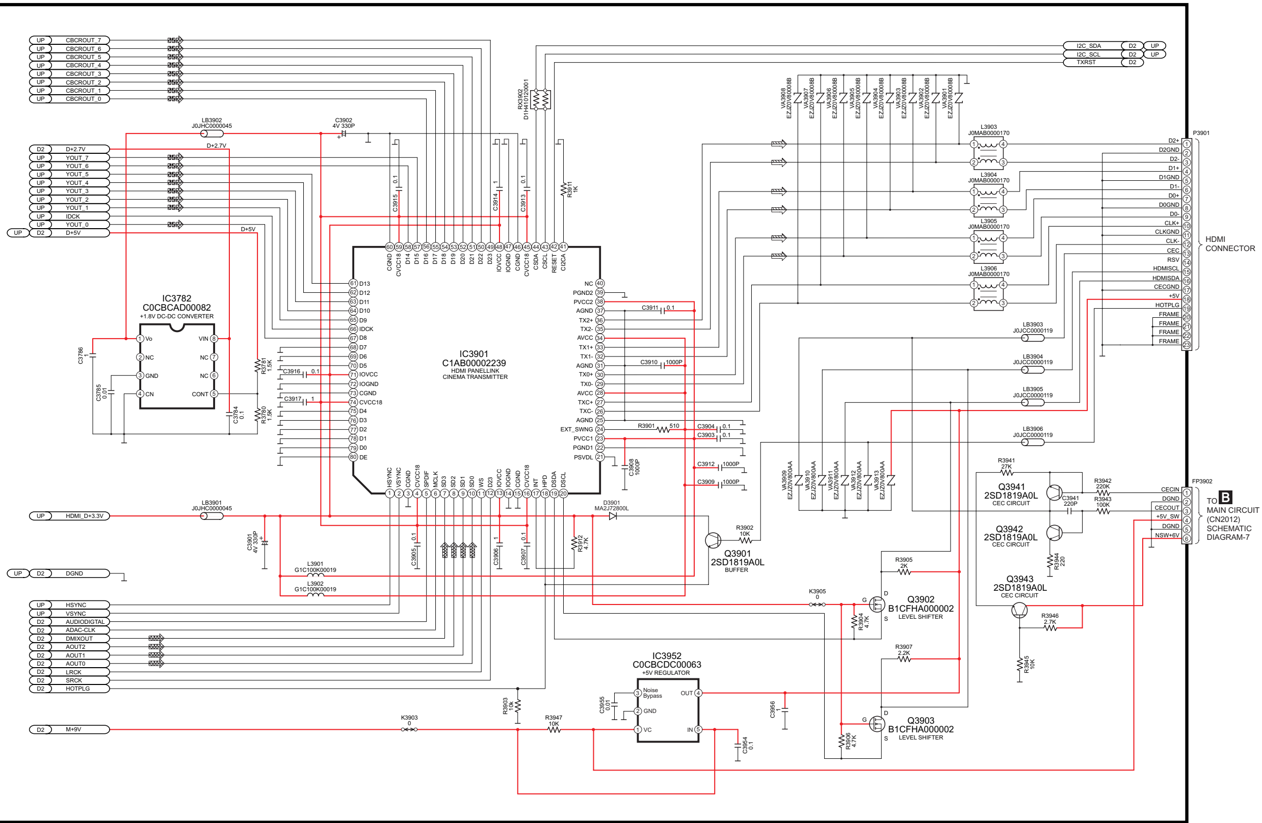
SA-HT940P/PC HDMI MODULE CIRCUIT
