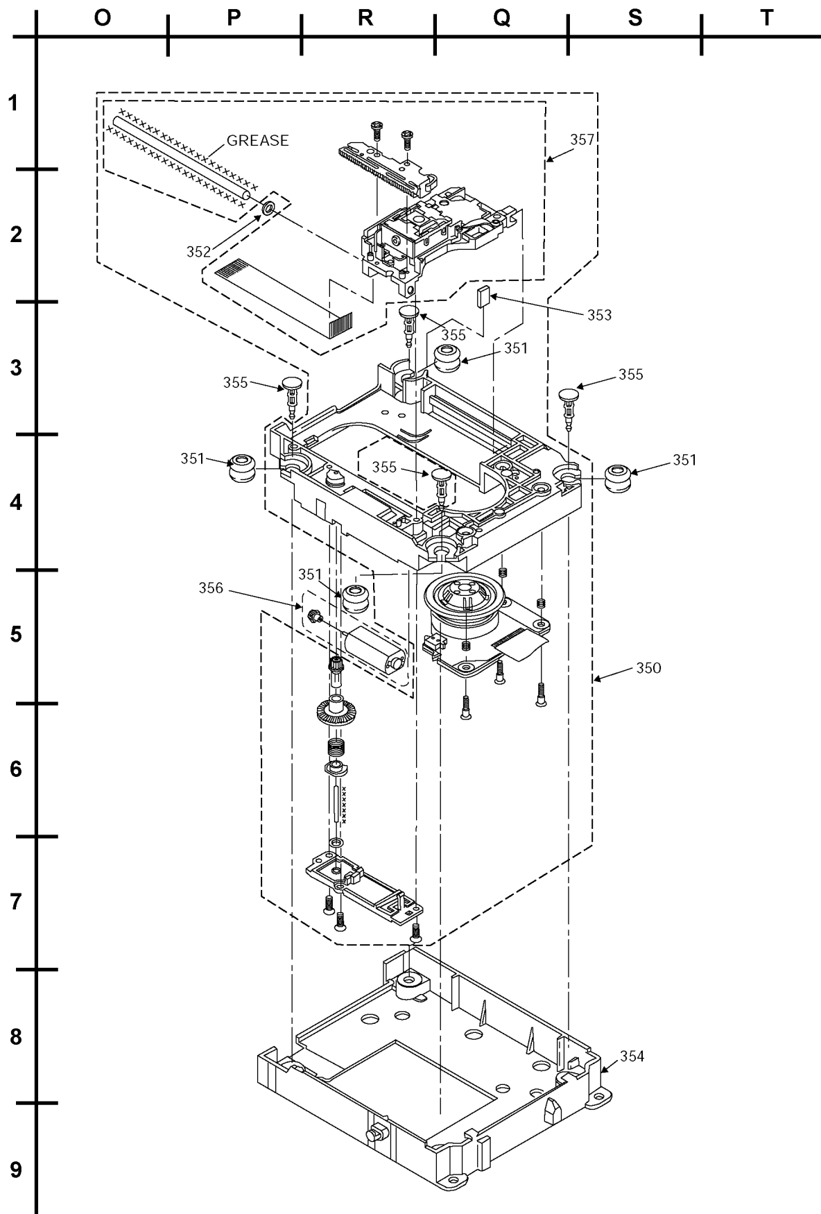
SA-HT940P/PC TRAVERSE MECHANISM DRAWINGS
