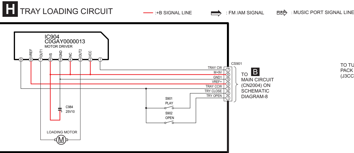
SCHEMATIC DIAGRAM-18
