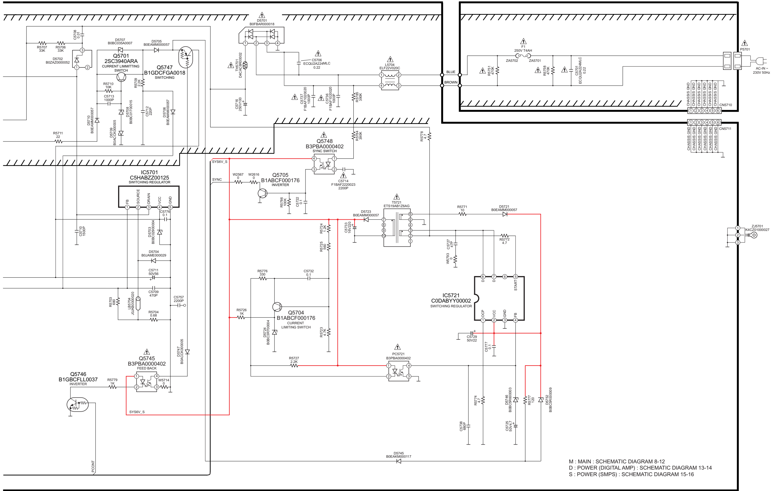
SA-HT995EE POWER(SMPS)/ AC-INLET CIRCUIT
