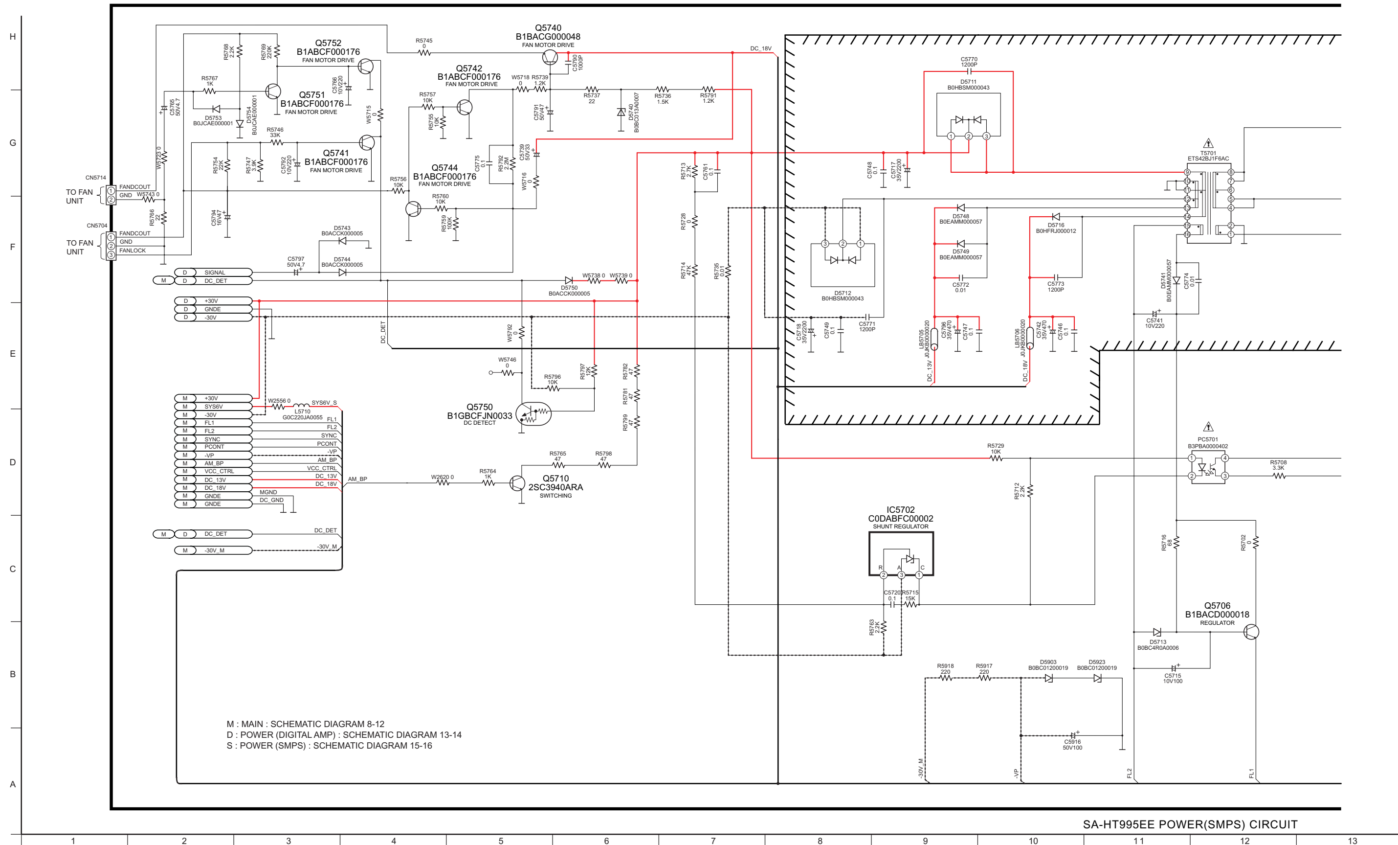
SCHEMATIC DIAGRAM-15
