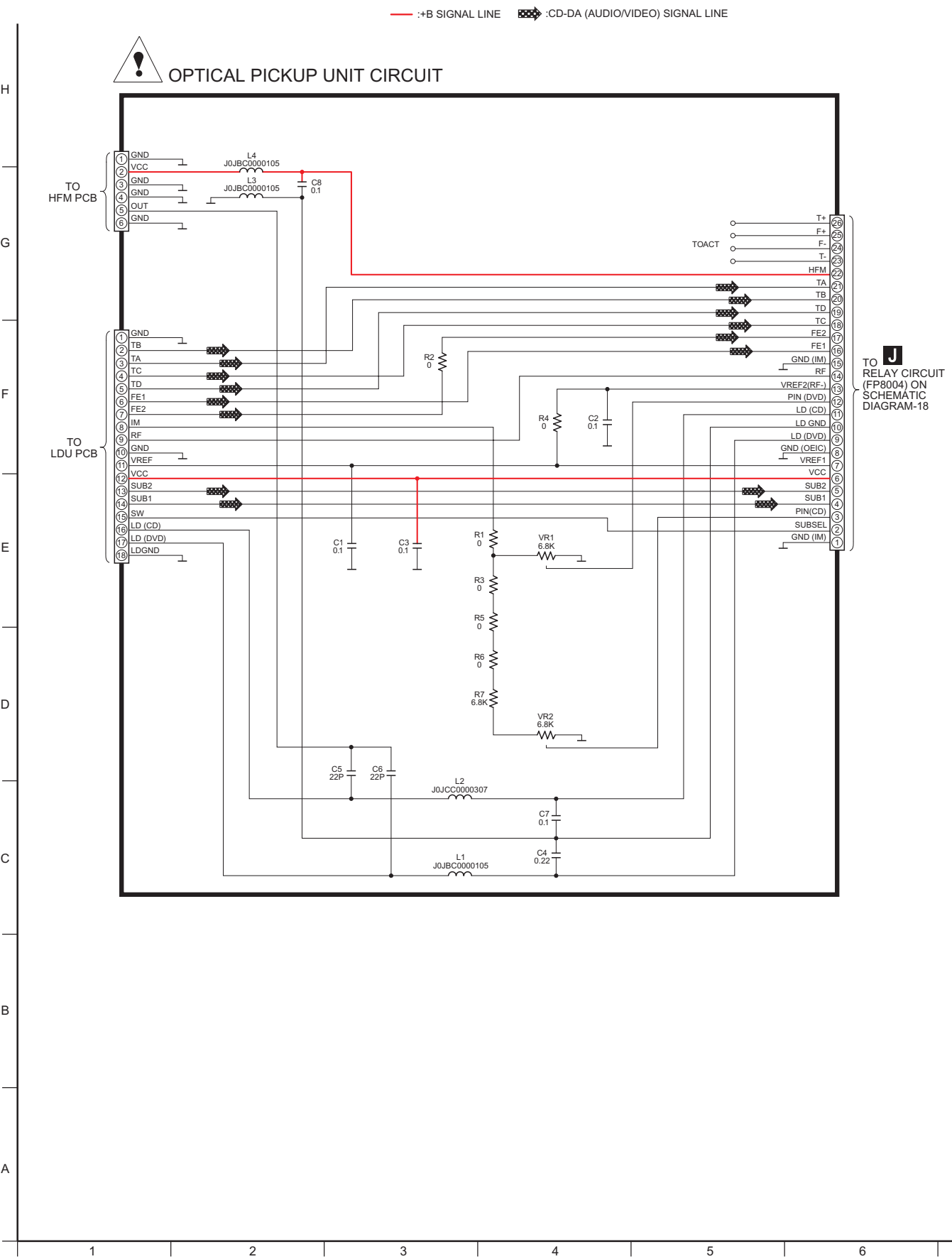
SCHEMATIC DIAGRAM-1
