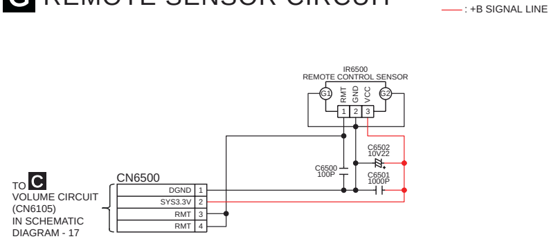
SCHEMATIC DIAGRAM - 20
