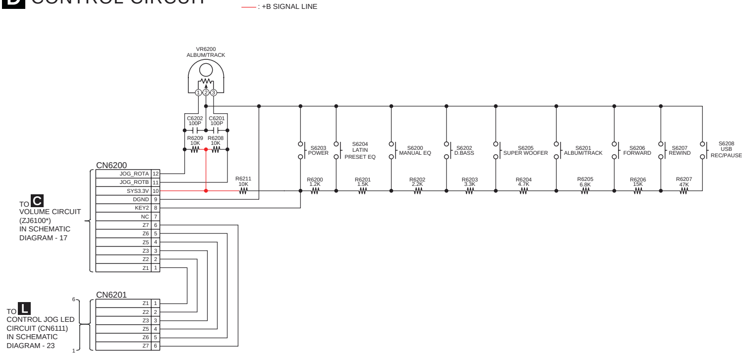
SCHEMATIC DIAGRAM - 18 D CONTROL CIRCUIT
