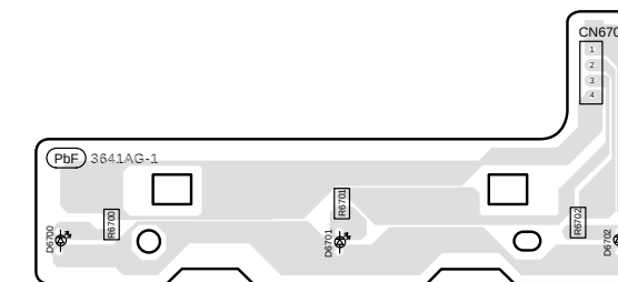
H LED P.C.B. (REP4883AG)
