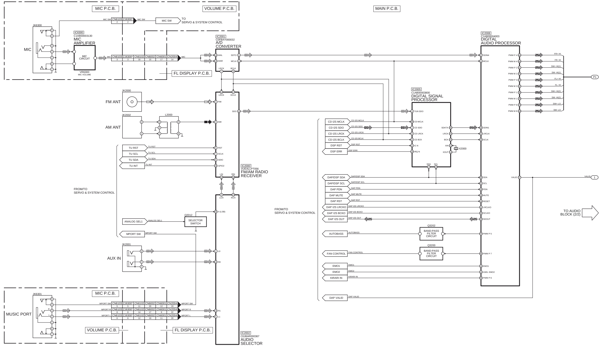
SA-MAX200PH AUDIO (1/2) BLOCK DIAGRAM
