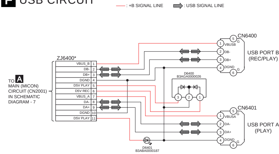
F USB CIRCUIT
