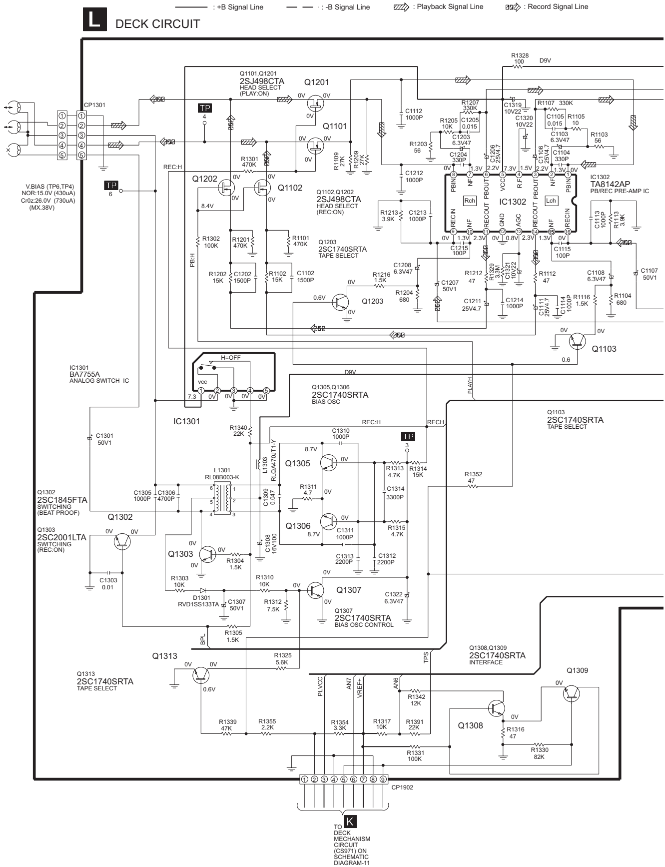
SCHEMATIC DIAGRAM-10
