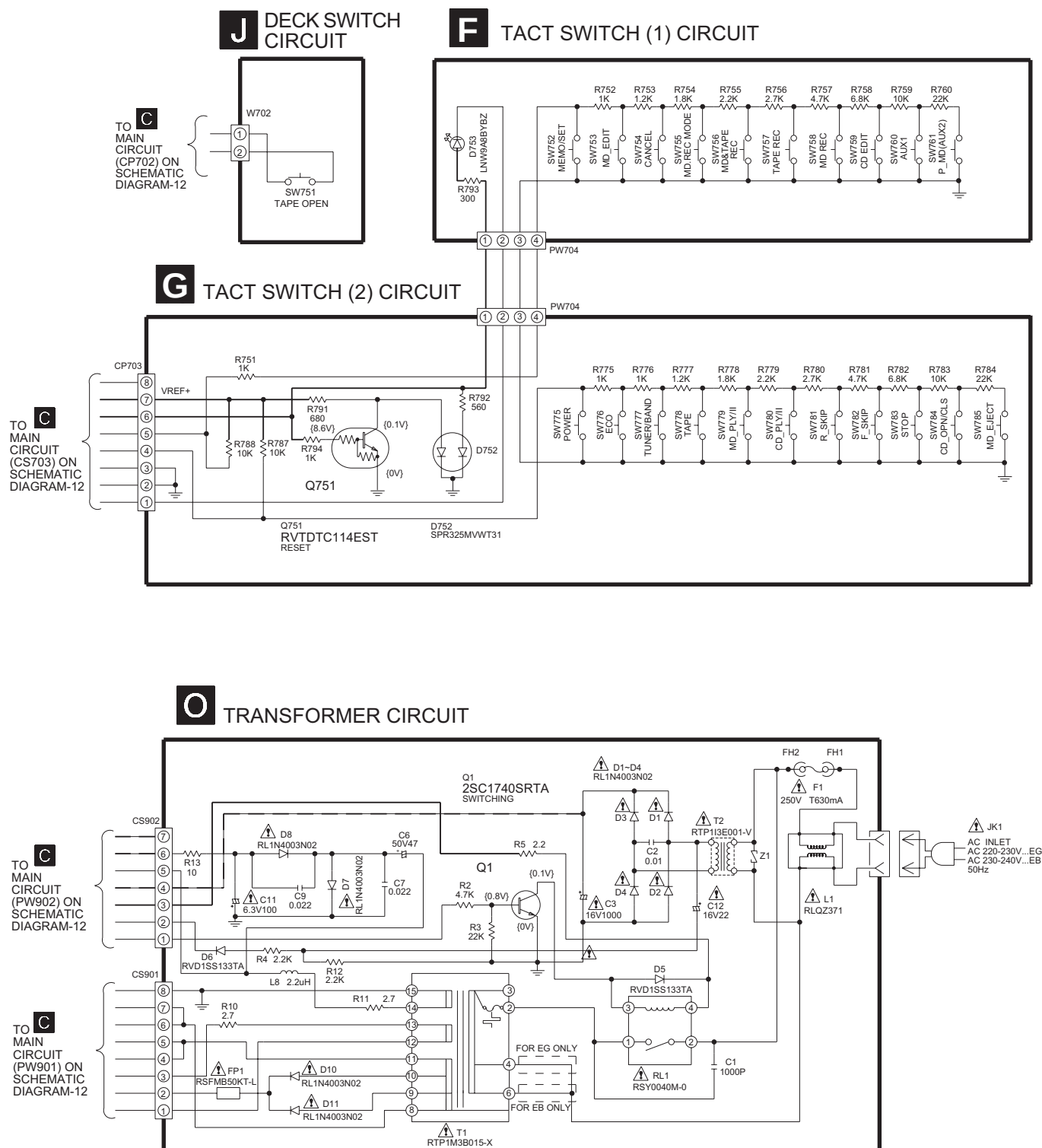
SCHEMATIC DIAGRAM-16
