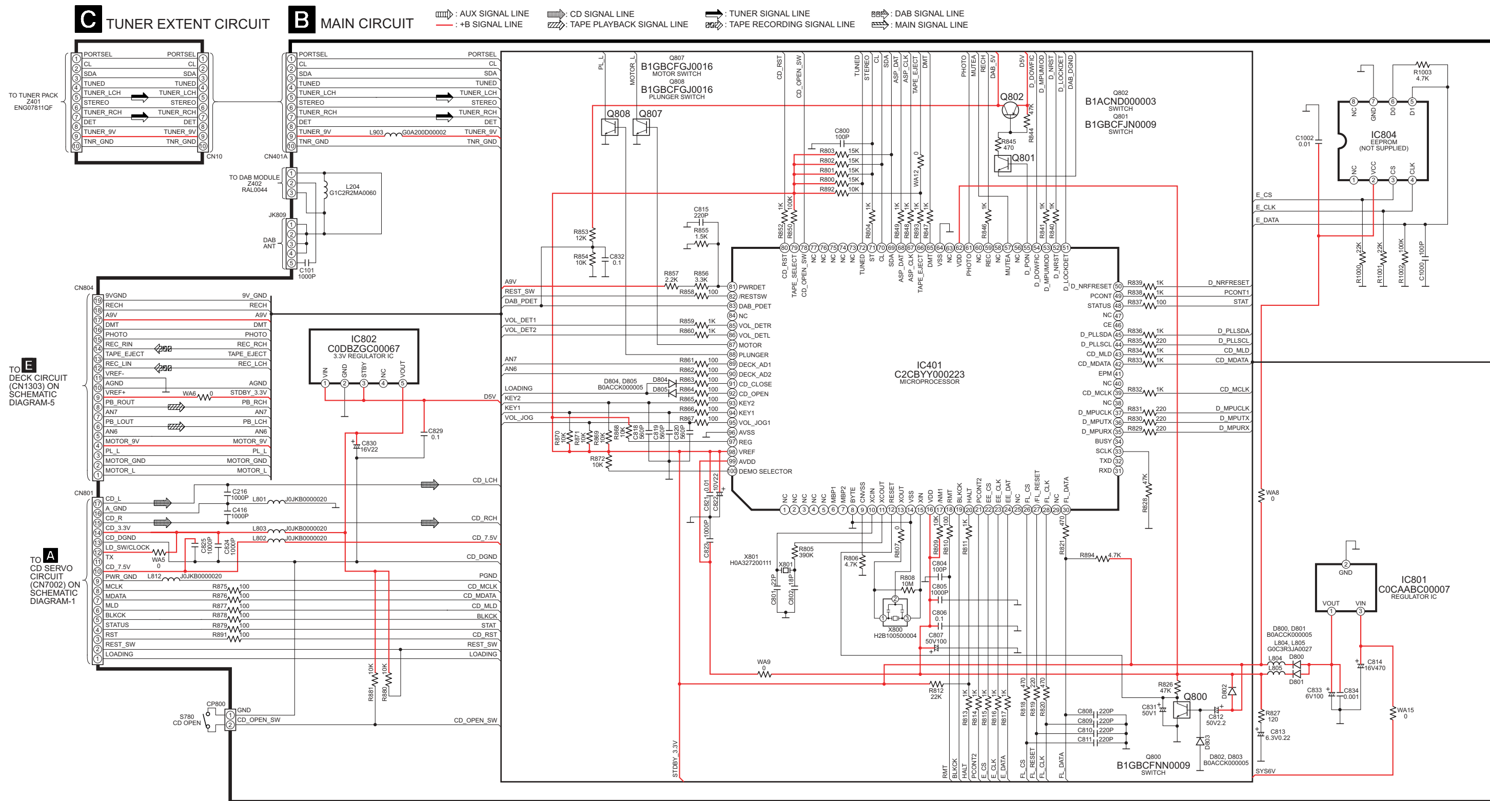
SCHEMATIC DIAGRAM - 2
