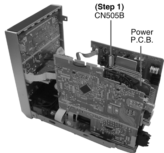
Step 1: Detach the connector CN505B.
