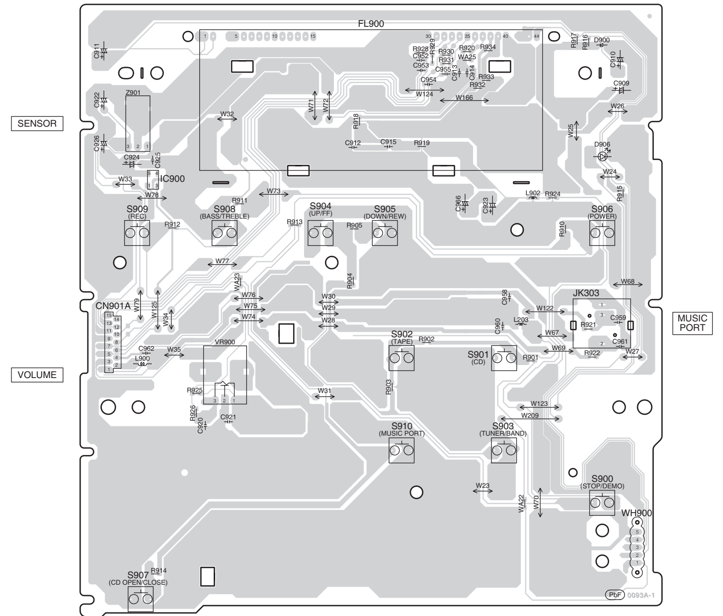
D PANEL P.C.B (REPV0093A)
