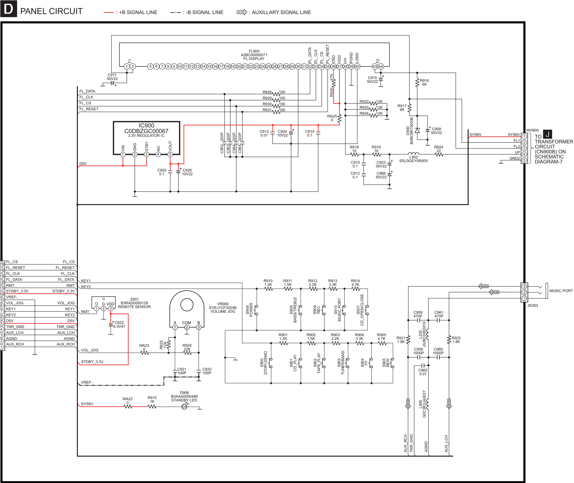
SCHEMATIC DIAGRAM - 4
