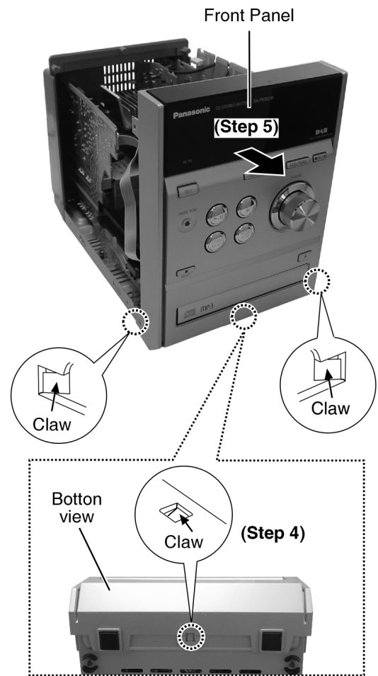
Step 4: Release 3 claws.
