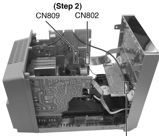
Step 2: Disconnect FFC cable (CN802 and CN809).
