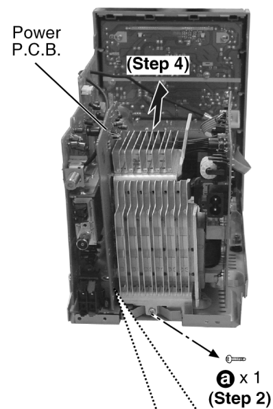
Step 1: Detach the connector CN505B.
