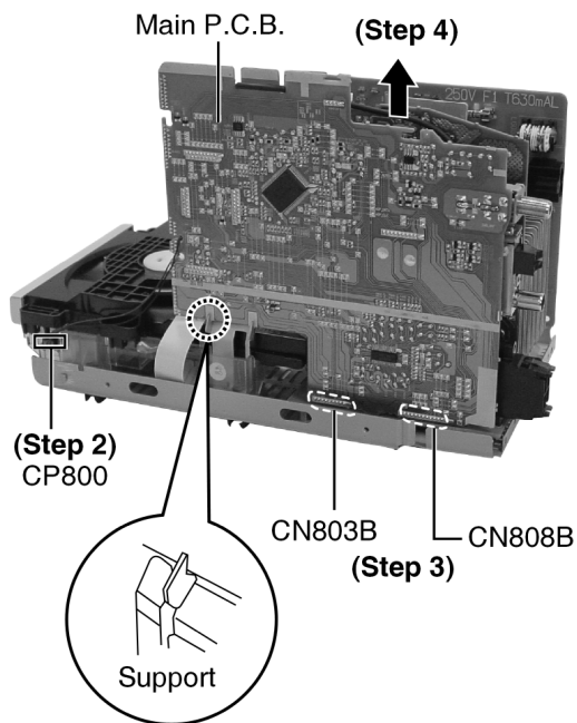
Step 2: Detach connector CP800.
