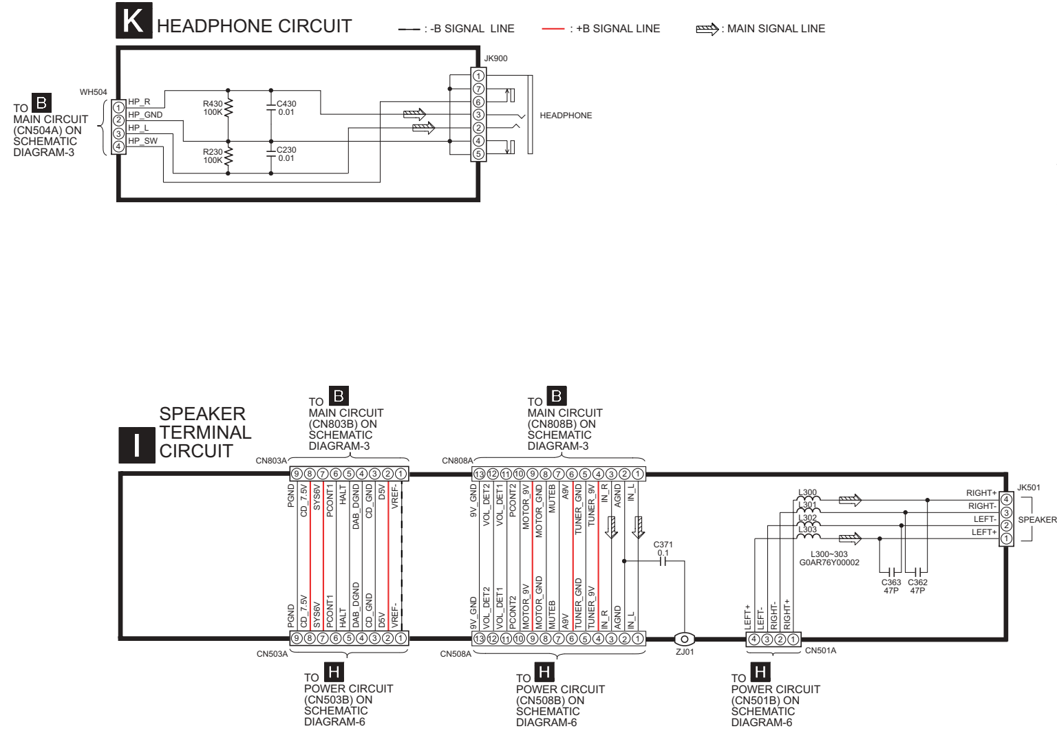
SCHEMATIC DIAGRAM - 7
