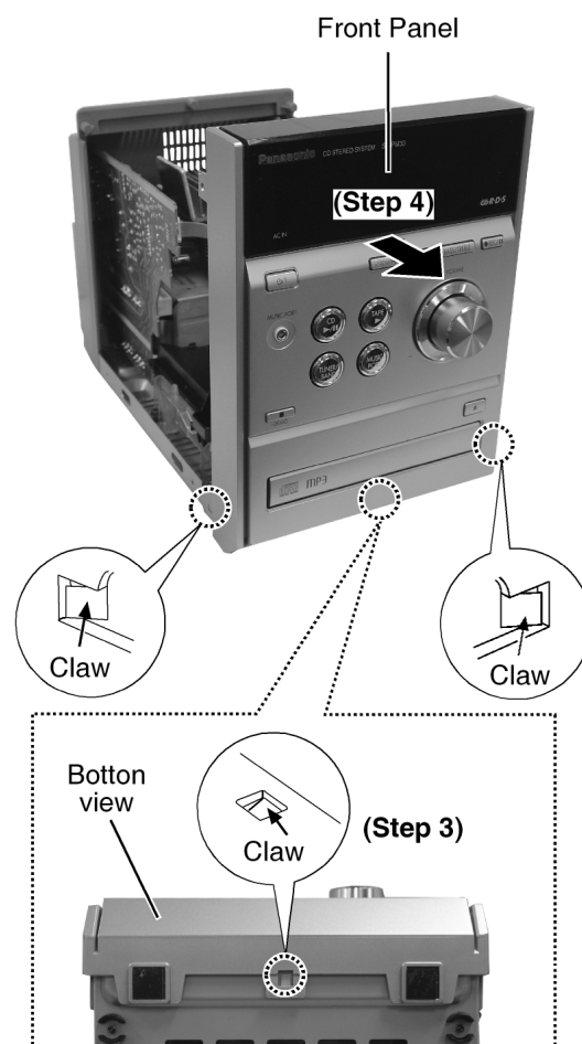
Step 3: Release 3 claws.
