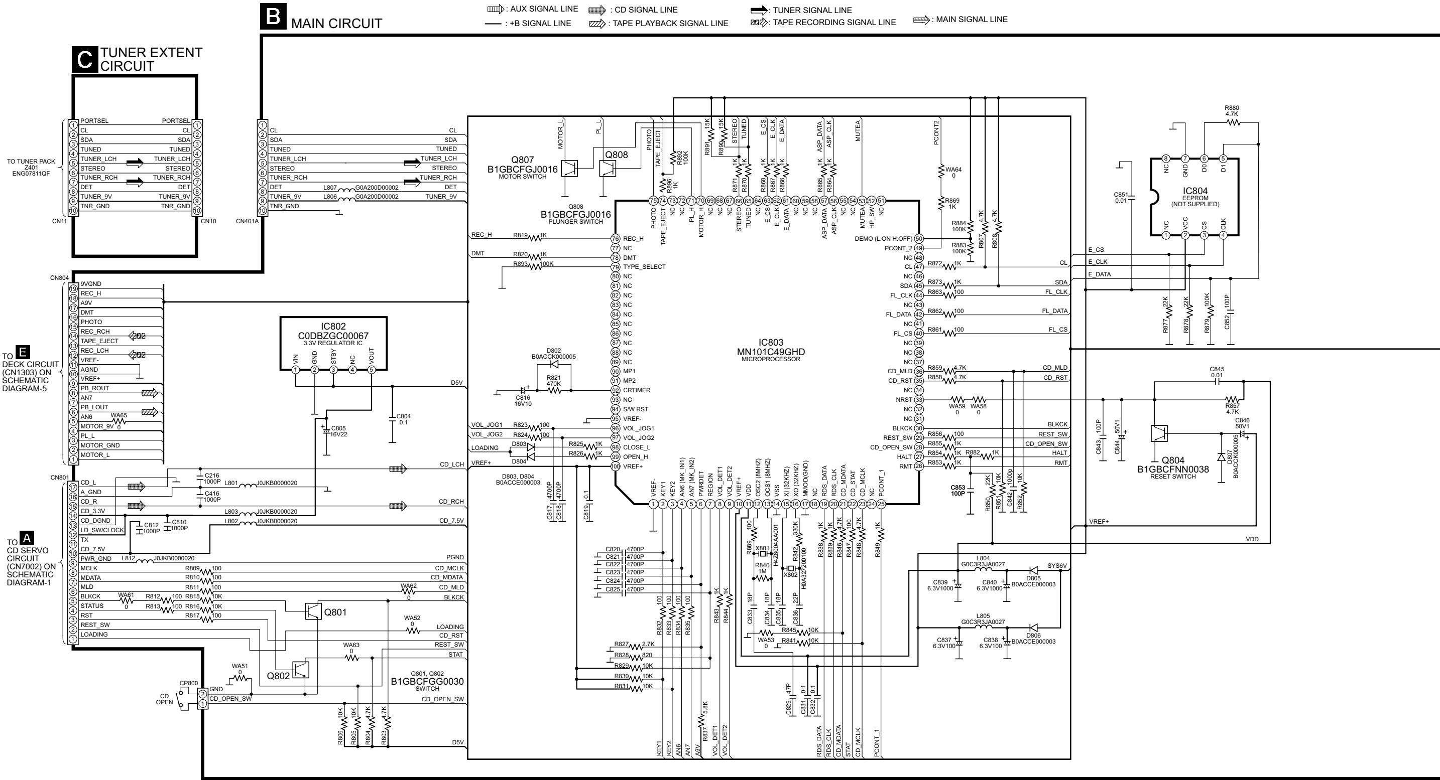
SCHEMATIC DIAGRAM - 2
