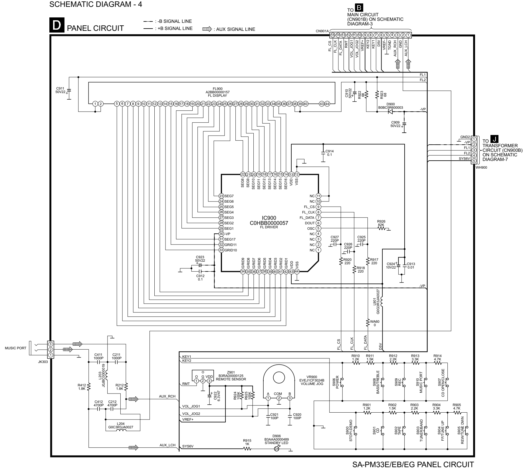
SCHEMATIC DIAGRAM - 4
