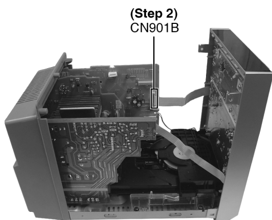
Step 2: Disconnect FFC cable (CN901B).
