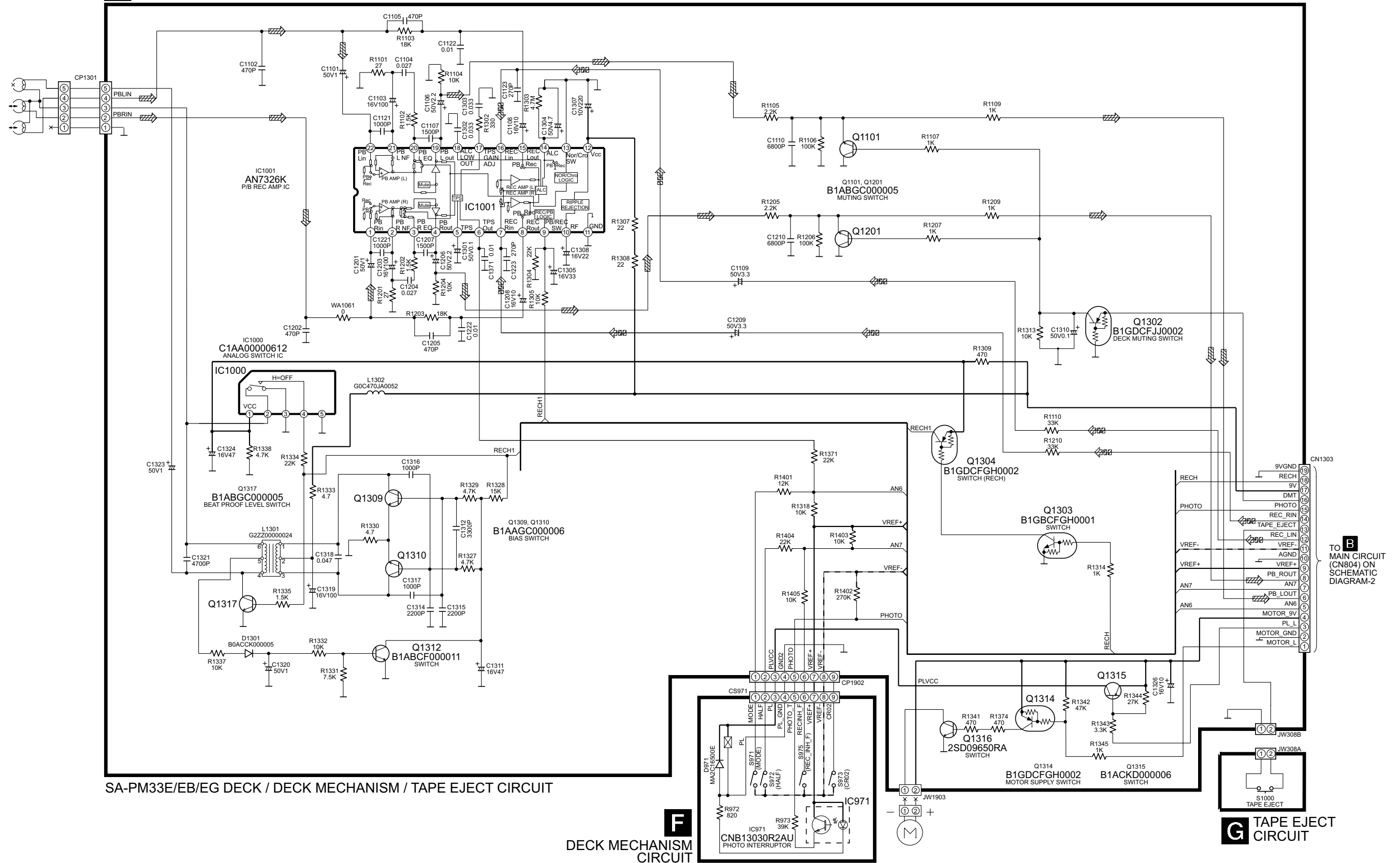
SCHEMATIC DIAGRAM - 5
