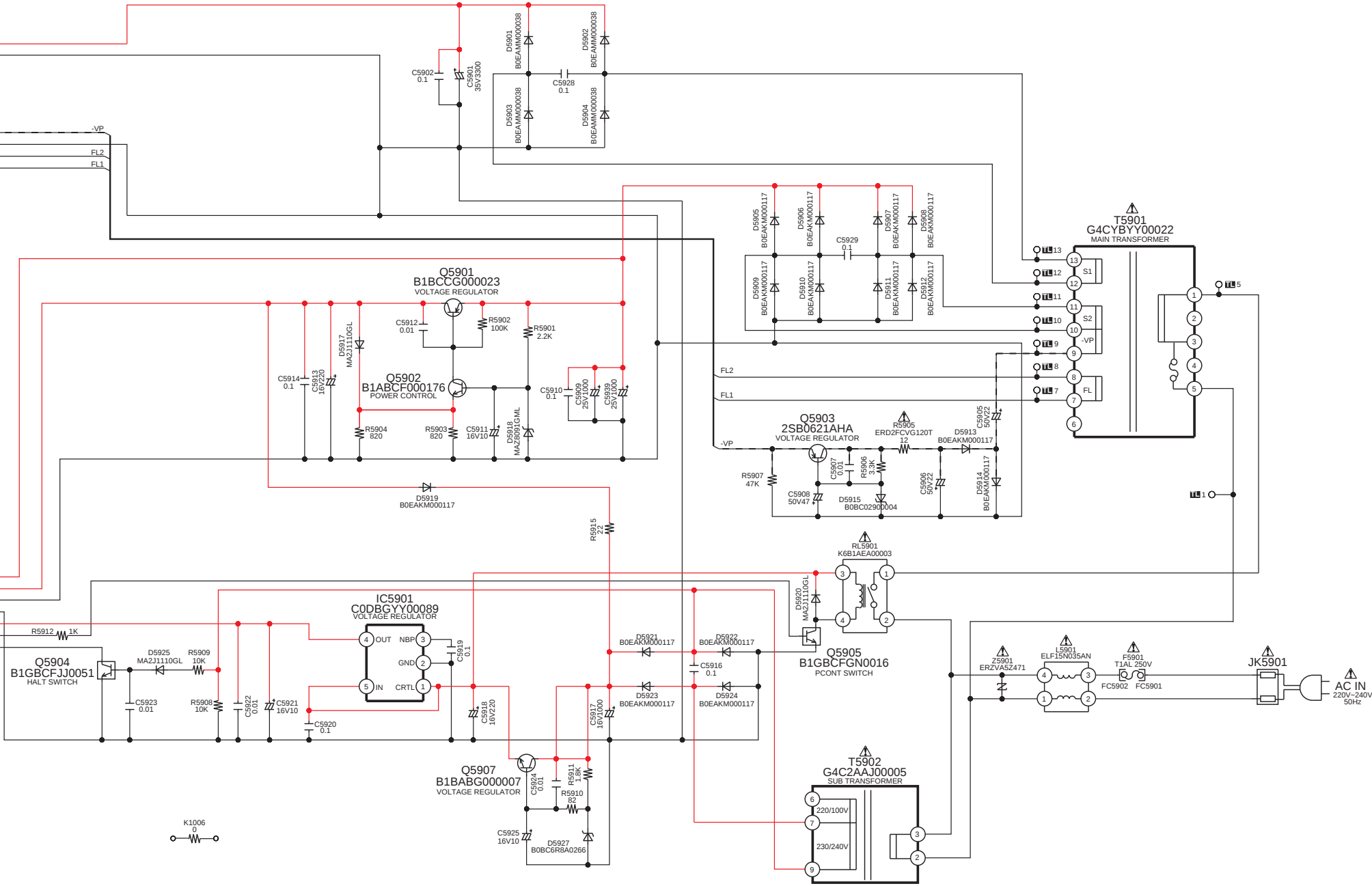
SA-PM42EF/EG/EP TRANSFORMER CIRCUIT
