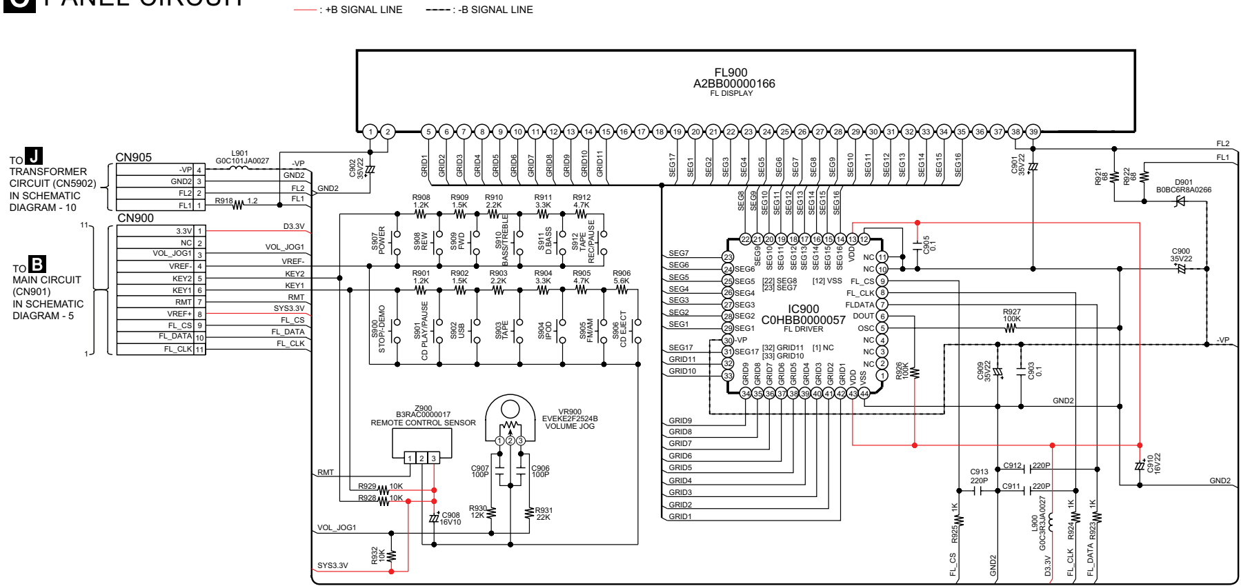
SCHEMATIC DIAGRAM - 6
