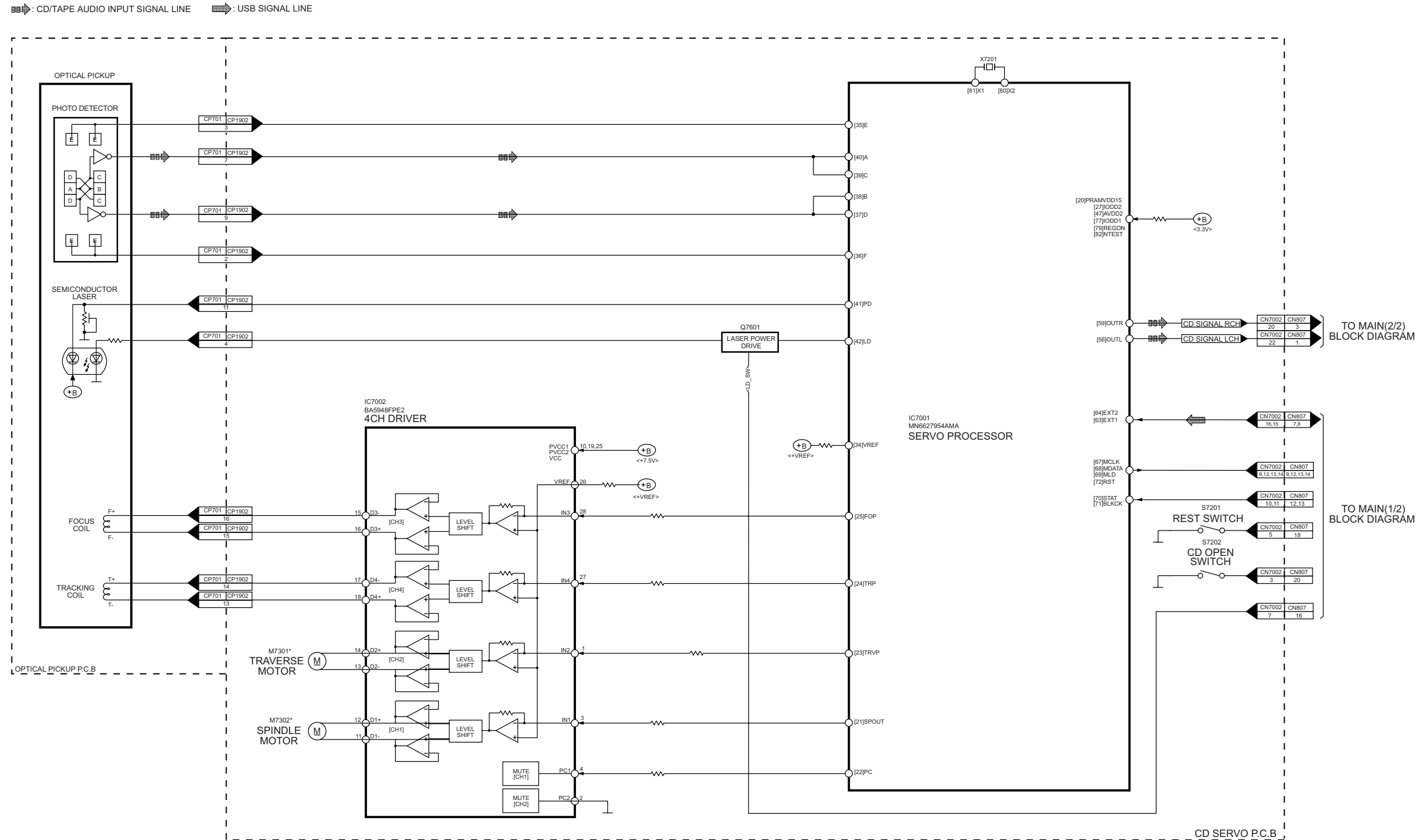
SA-PM48EG CD SERVO BLOCK DIAGRAM
