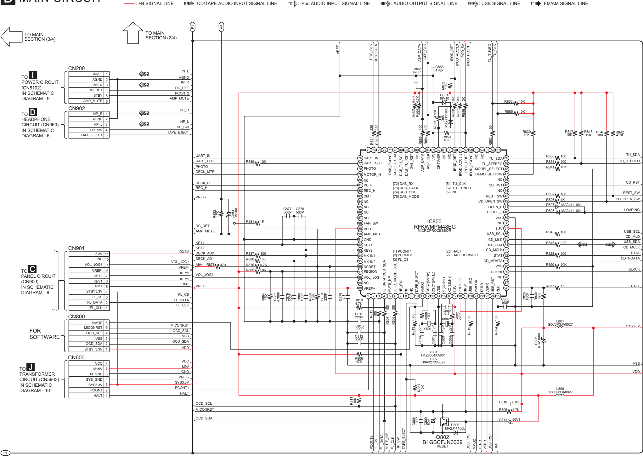
SCHEMATIC DIAGRAM - 5 B MAIN CIRCUIT
