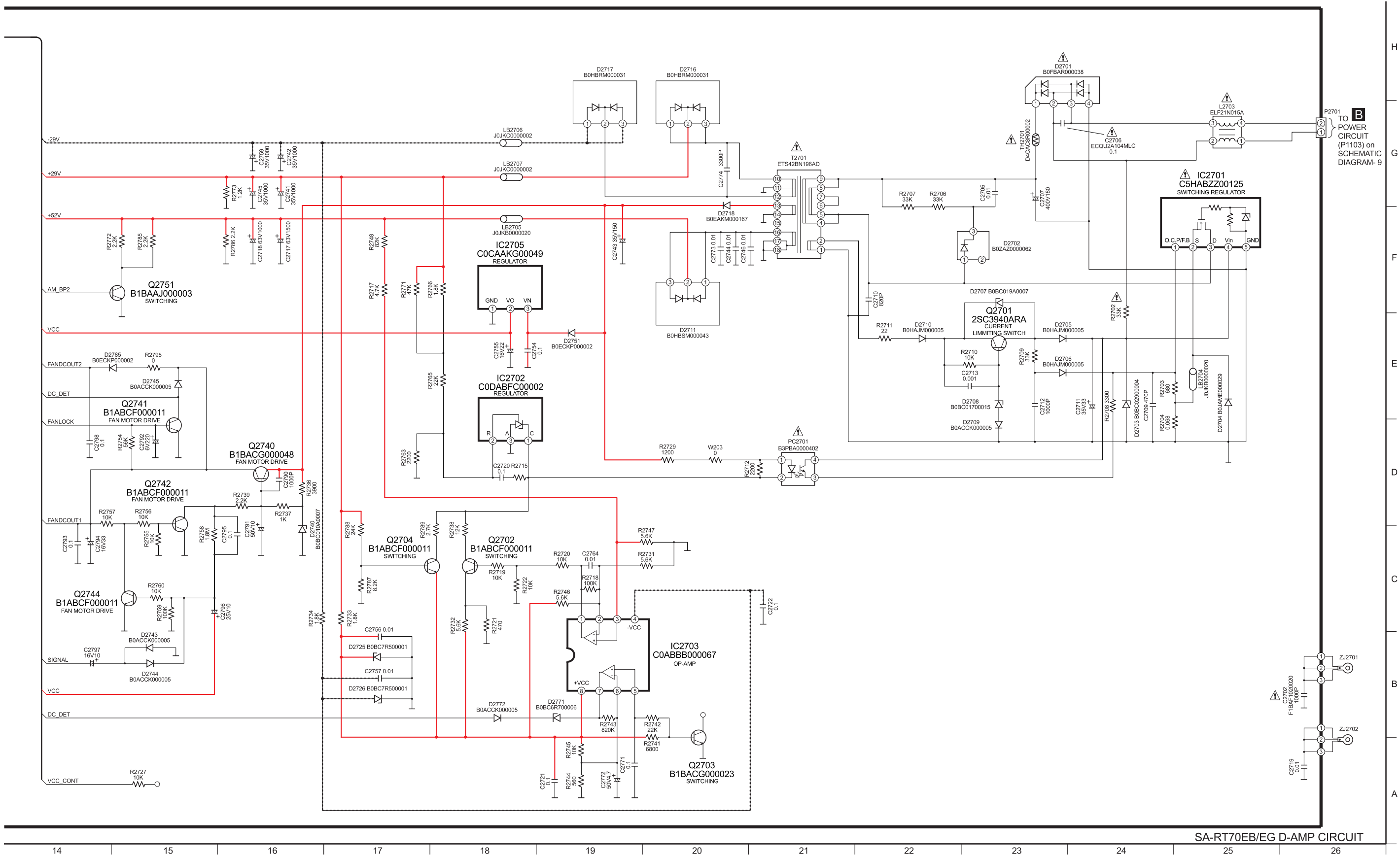
SCHEMATIC DIAGRAM-12
