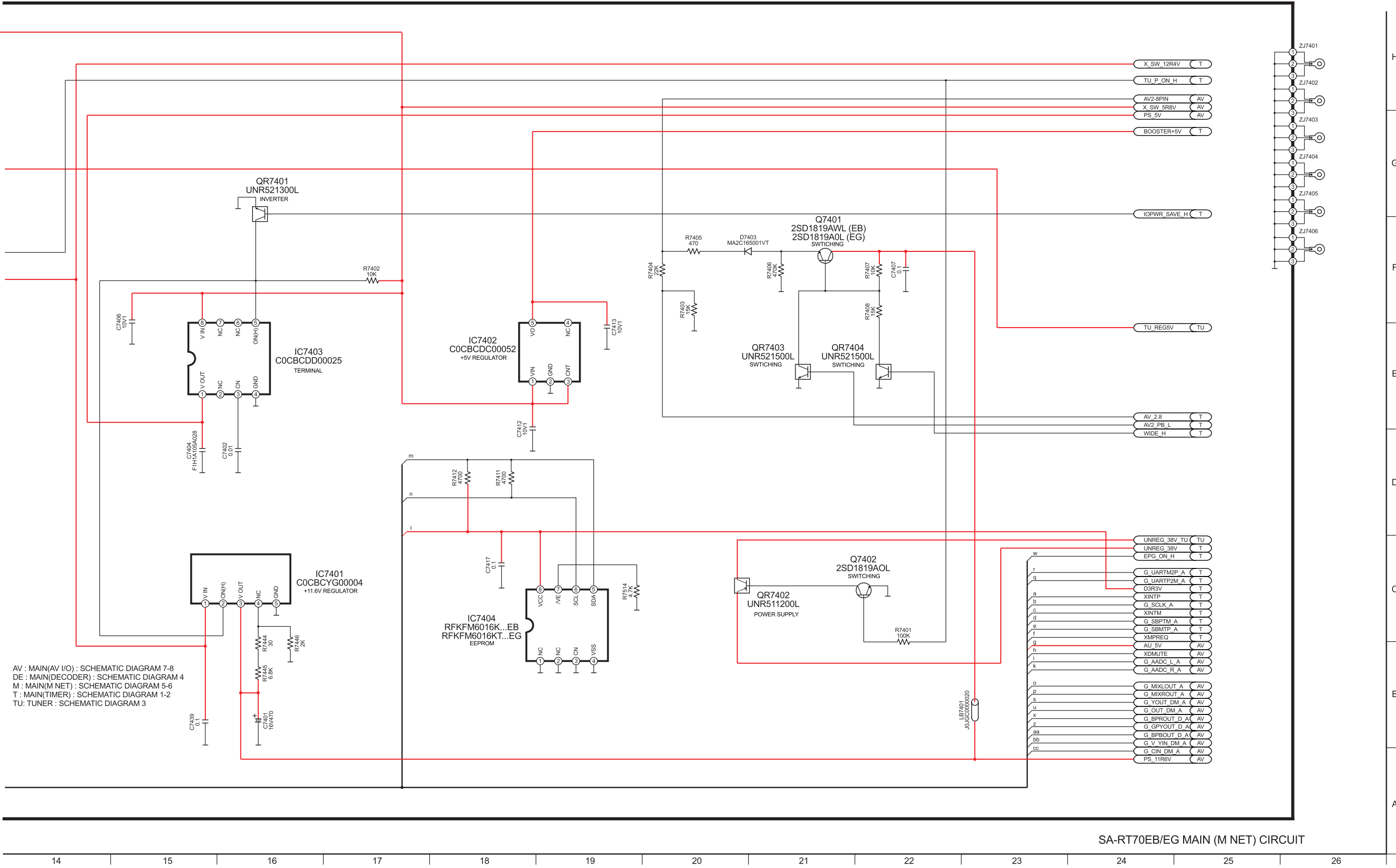
SCHEMATIC DIAGRAM-6
