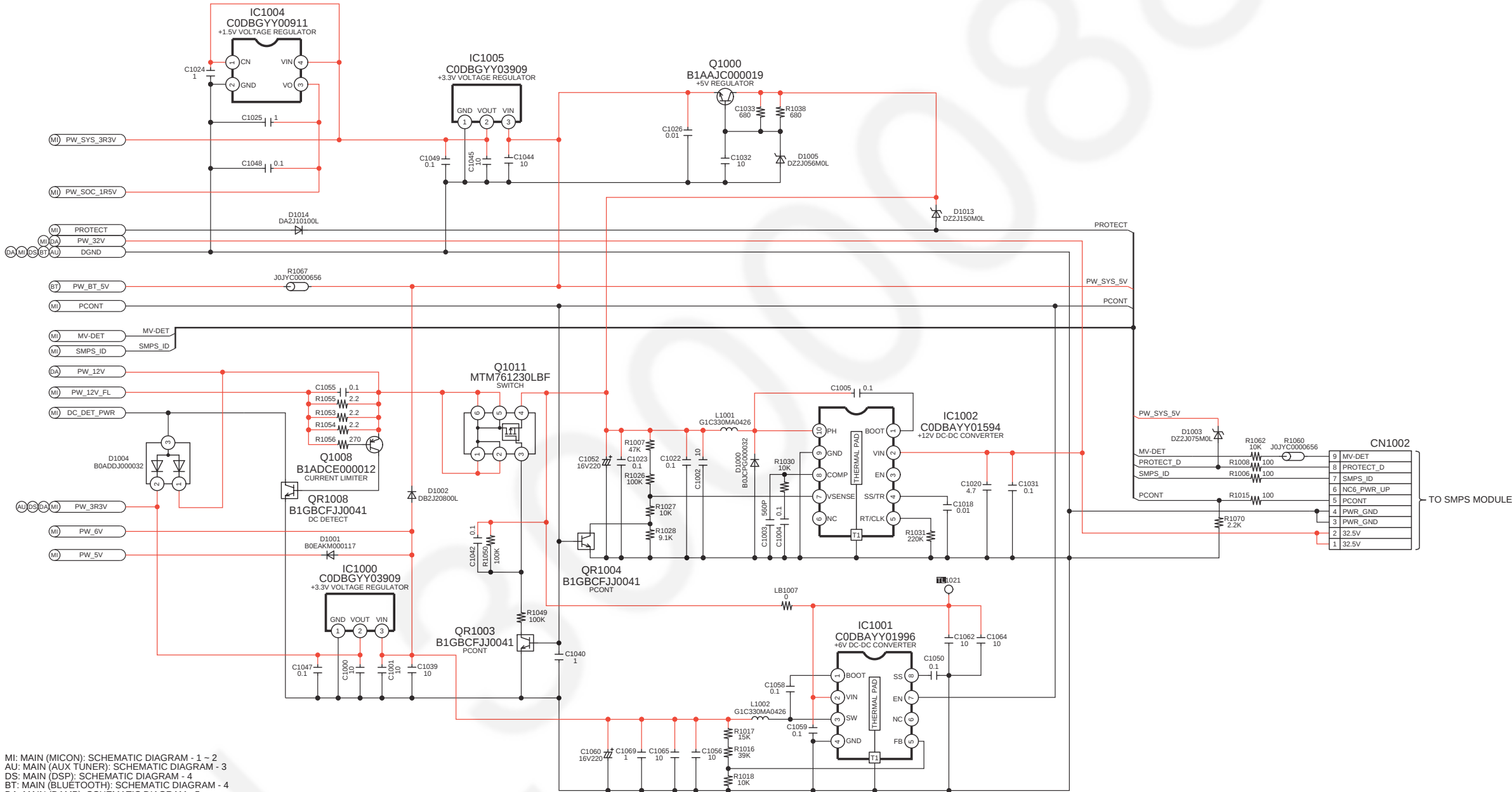
SA-UX100EE/GSX MAIN (VOLTAGE REGULATOR) CIRCUIT
