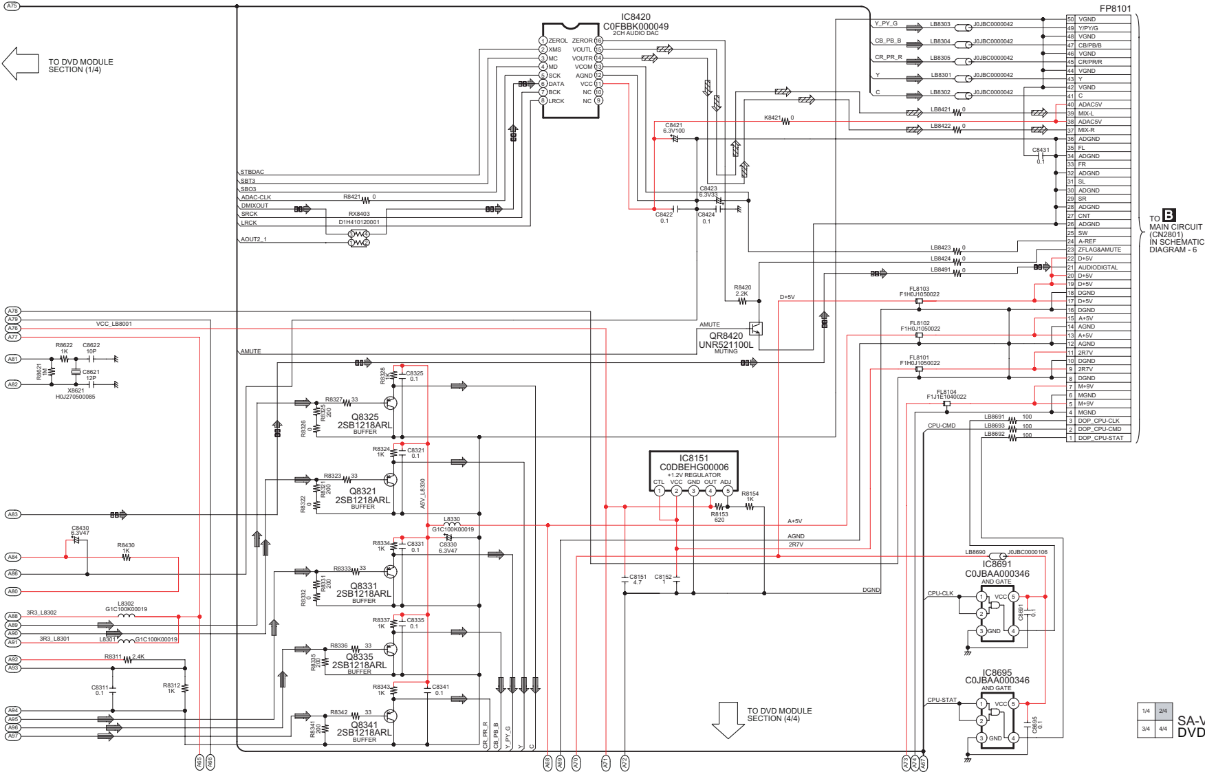
SCHEMATIC DIAGRAM - 2
