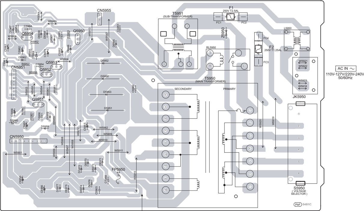
I SMPS P.C.B. (REPX0519D...GS/GCS/GCT)
