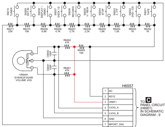
SCHEMATIC DIAGRAM - 11
