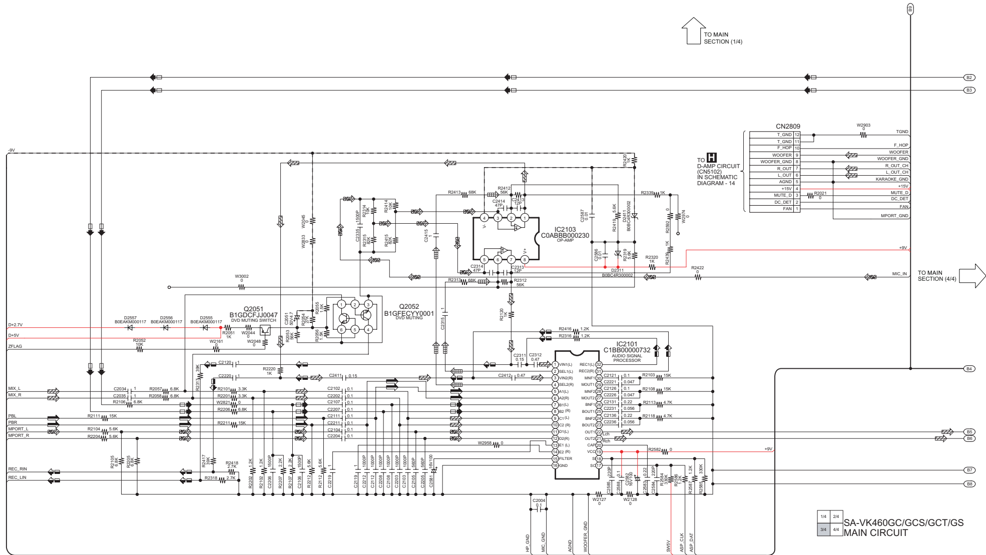
SCHEMATIC DIAGRAM - 7
