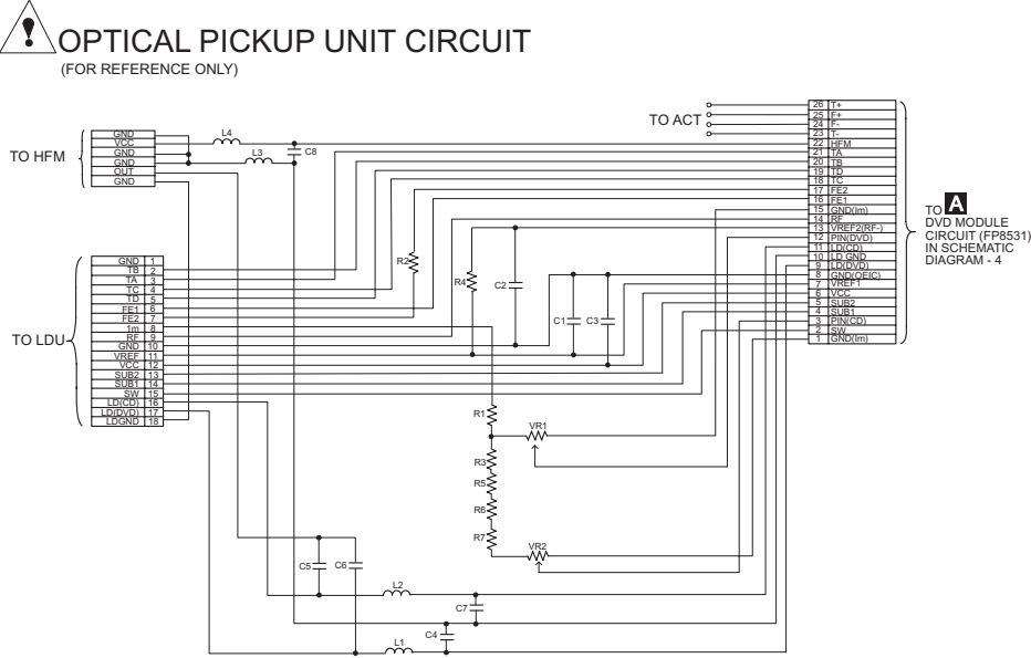
SCHEMATIC DIAGRAM - 16
