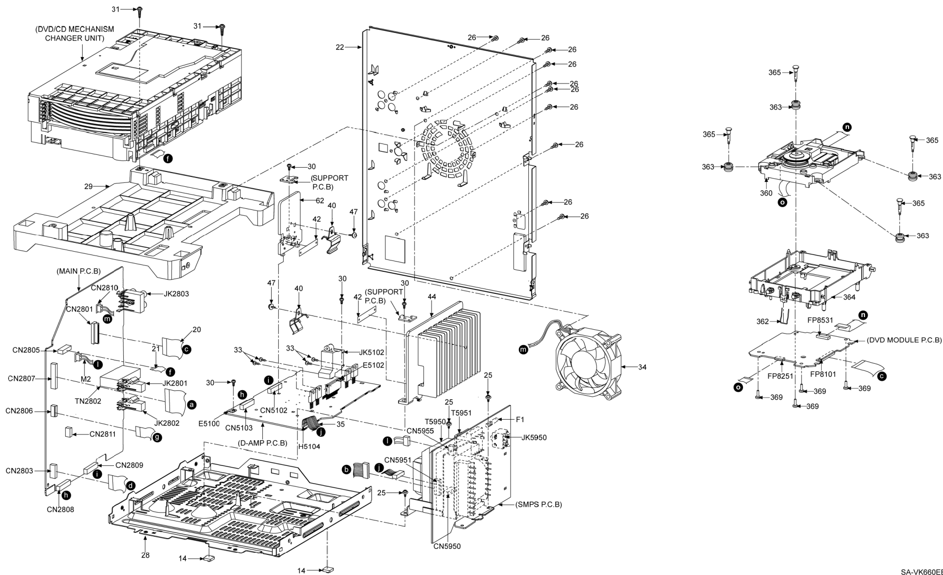
SA-VK660EE-K CABINET UNIT DRAWINGS
