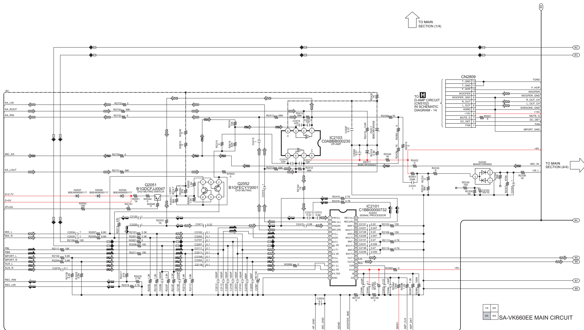
SCHEMATIC DIAGRAM - 7
