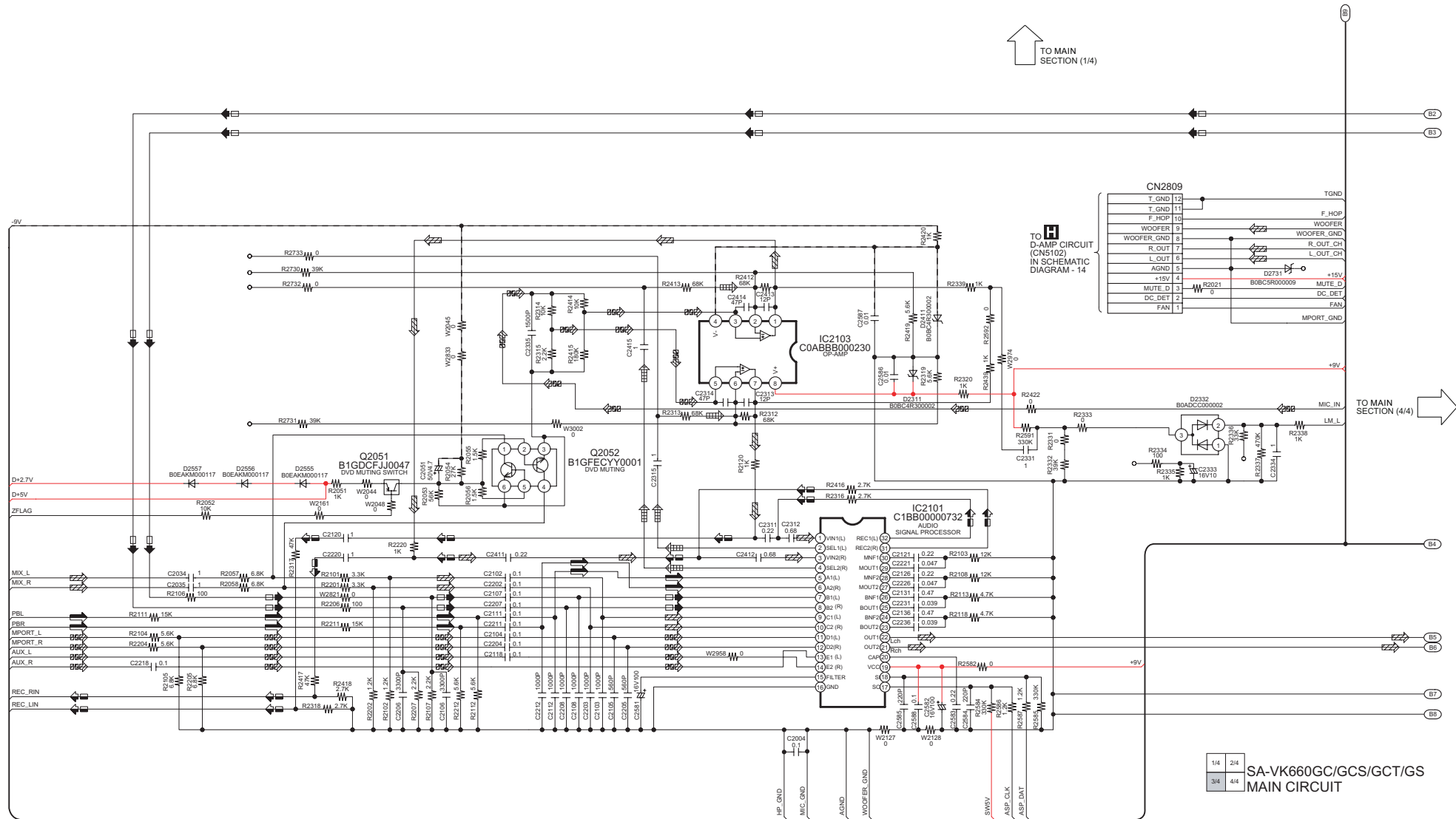
SCHEMATIC DIAGRAM - 7
