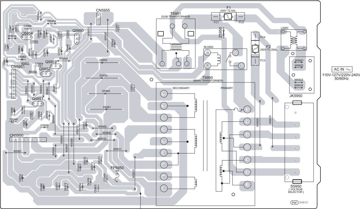
I SMPS P.C.B. (REPX0519D...GCS/GS/GCT)
