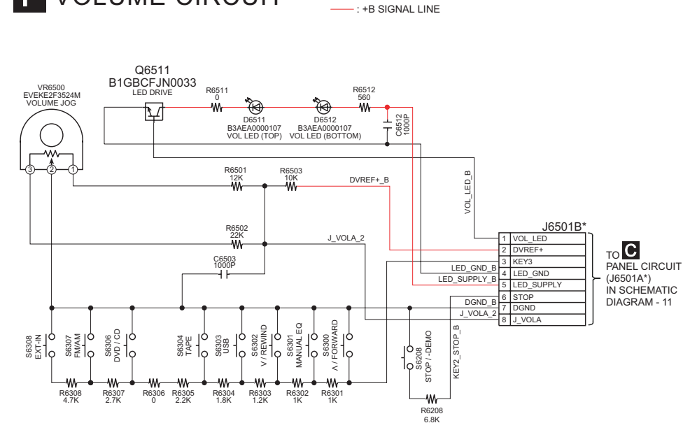
SCHEMATIC DIAGRAM - 12
