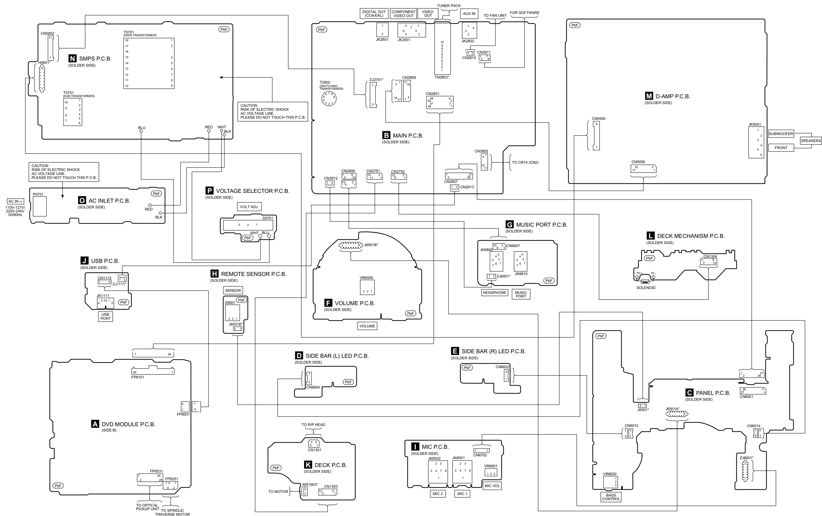
SA-VK680PU WIRING CONNECTION
