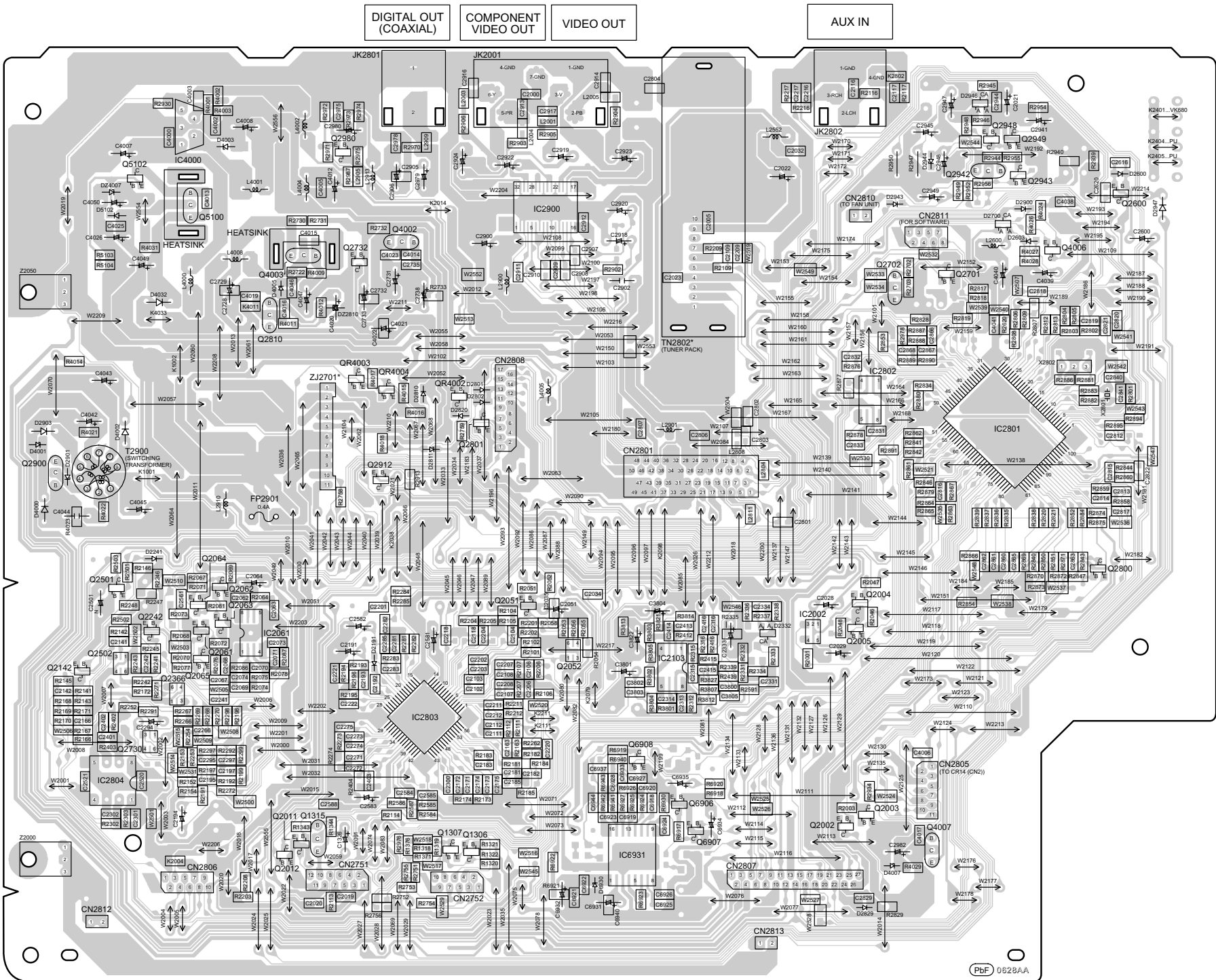
B MAIN P.C.B. (REPX0736H)
