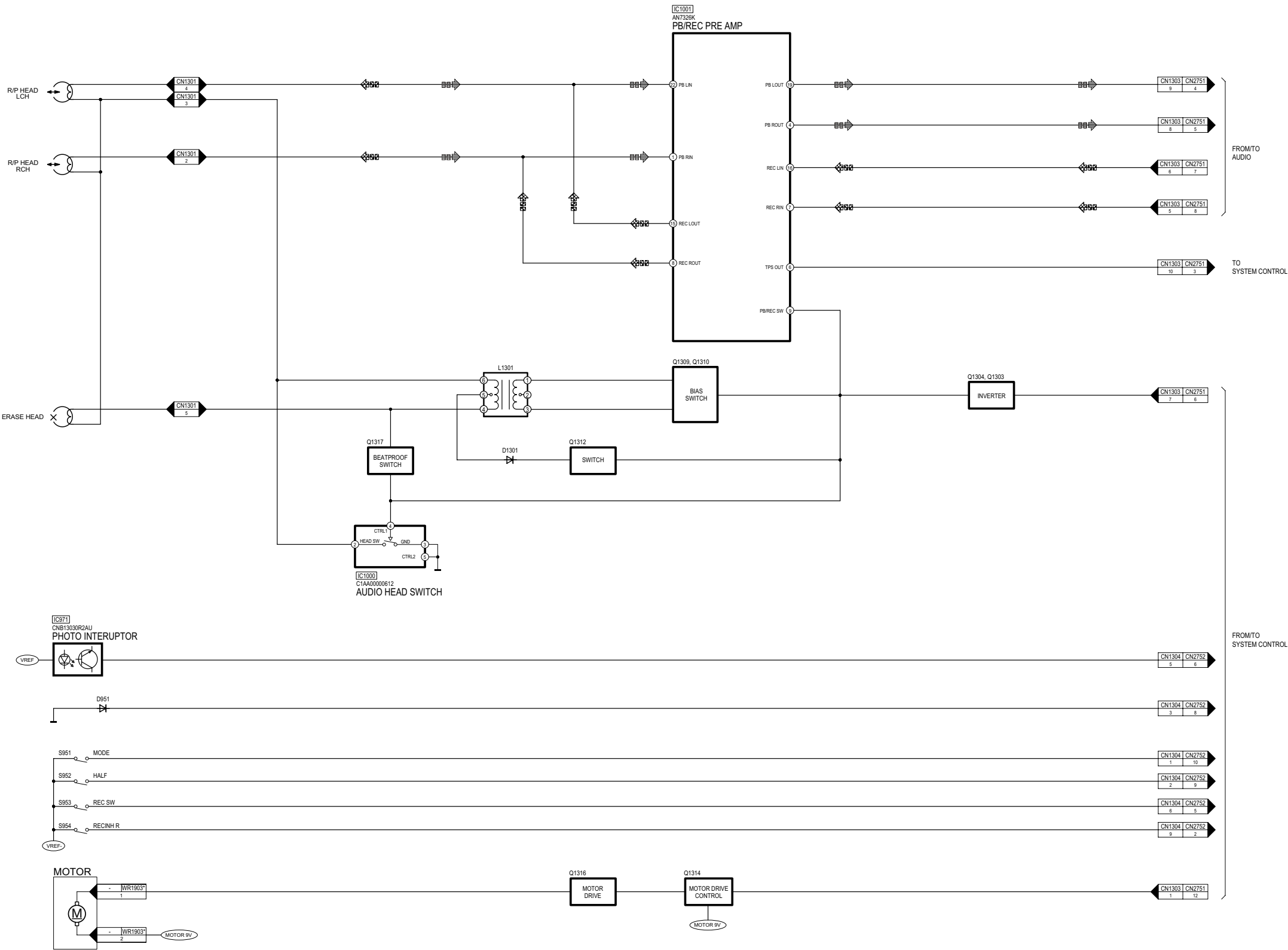
SA-VK680PU DECK BLOCK DIAGRAM
